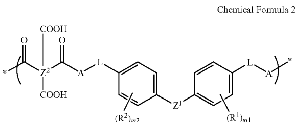
Chemical Formula 2
