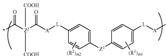
Chemical Formula 2
