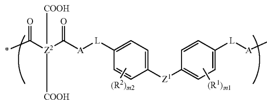
Chemical Formula 2
