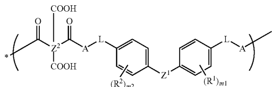
Chemical Formula 2
