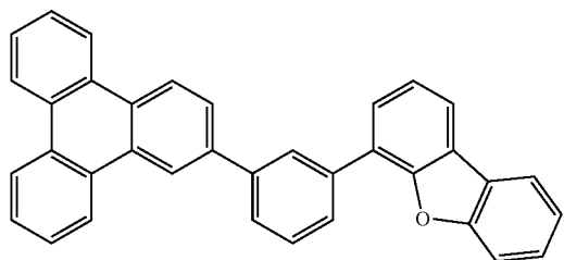
compound I-11
