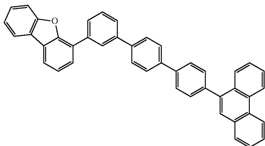
compound 1-5
