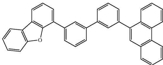
compound 1-3
