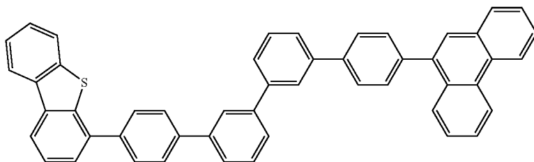
compound 1-8
