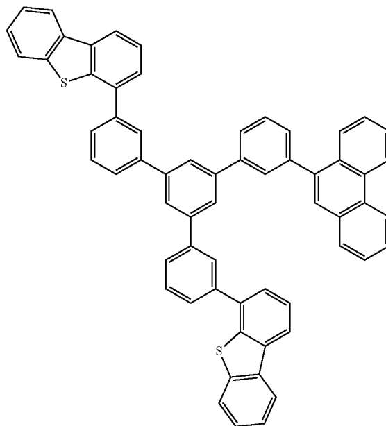
compound 1-22
