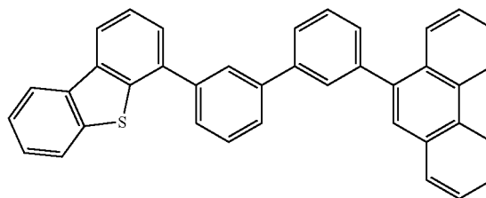
compound 1-4
