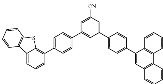
compound 1-11
