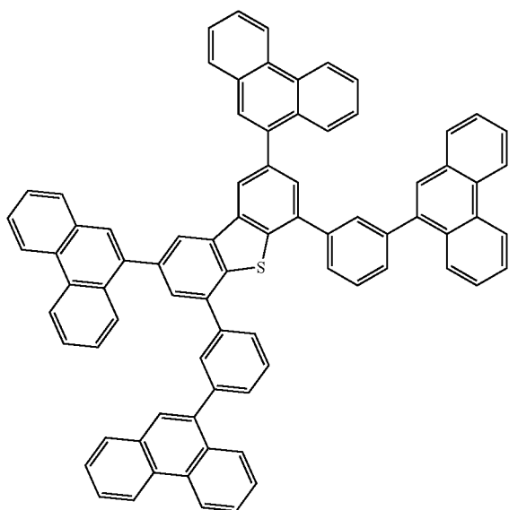
compound 1-25
