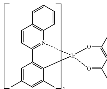
iridium complex A
