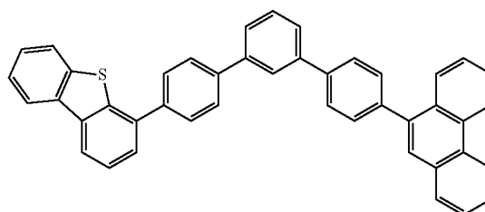
compound 1-4
