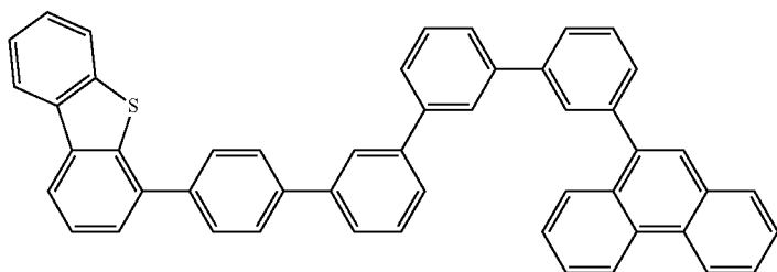
compound 1-8
