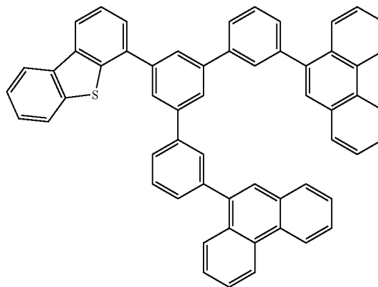
compound 1-20
