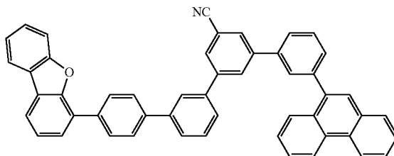
compound 1-13
