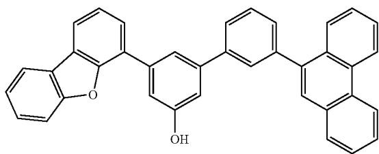
compound 1-9
