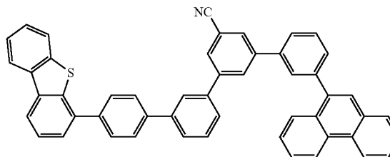
compound 1-14
