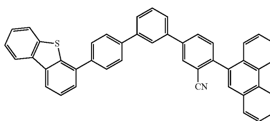
compound 1-12
