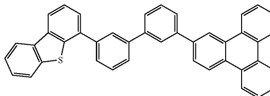
compound I-12
