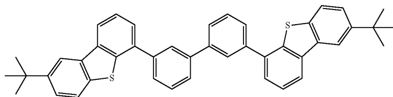
compound I-7
