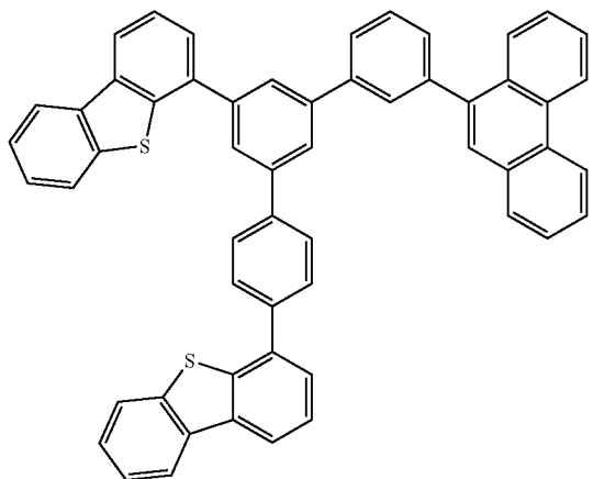
compound 1-21
