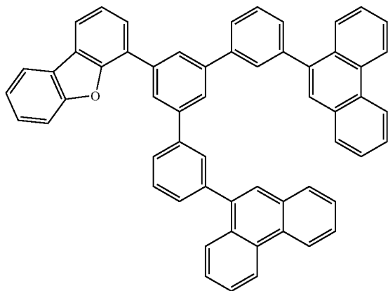
compound 1-19
