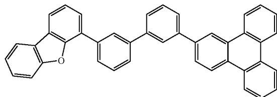
compound I-11
