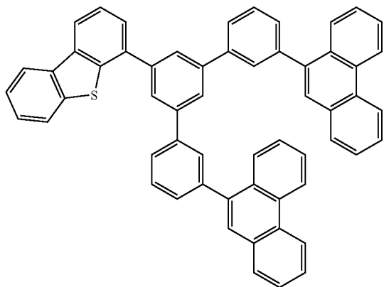
compound 1-19
