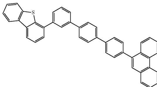
compound 1-7
