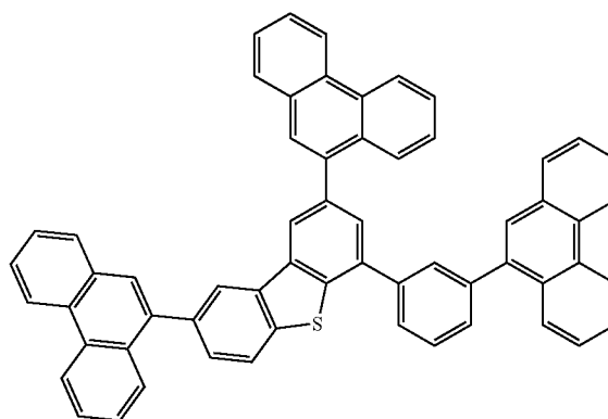
compound 1-26
