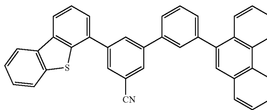
compound 1-10
