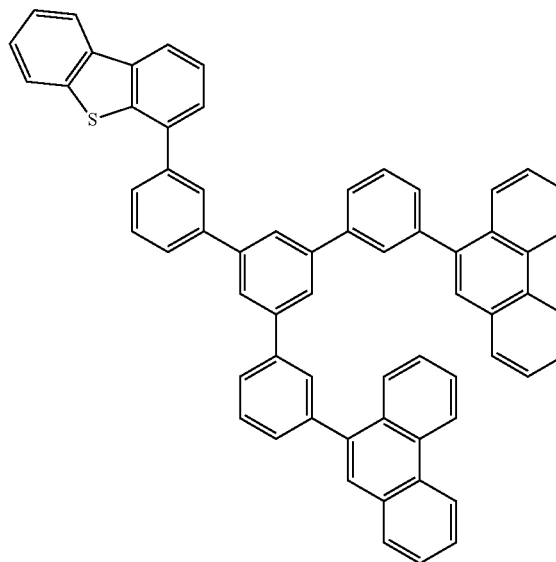
compound 1-22
