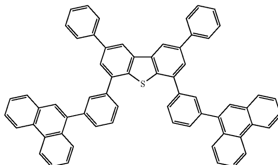
compound 1-24
