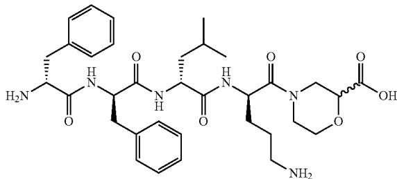
Compound (90): D-Phe-D-Phe-D-Leu-D-Orn-[R/S-2-carboxymorpholine]-OH:
