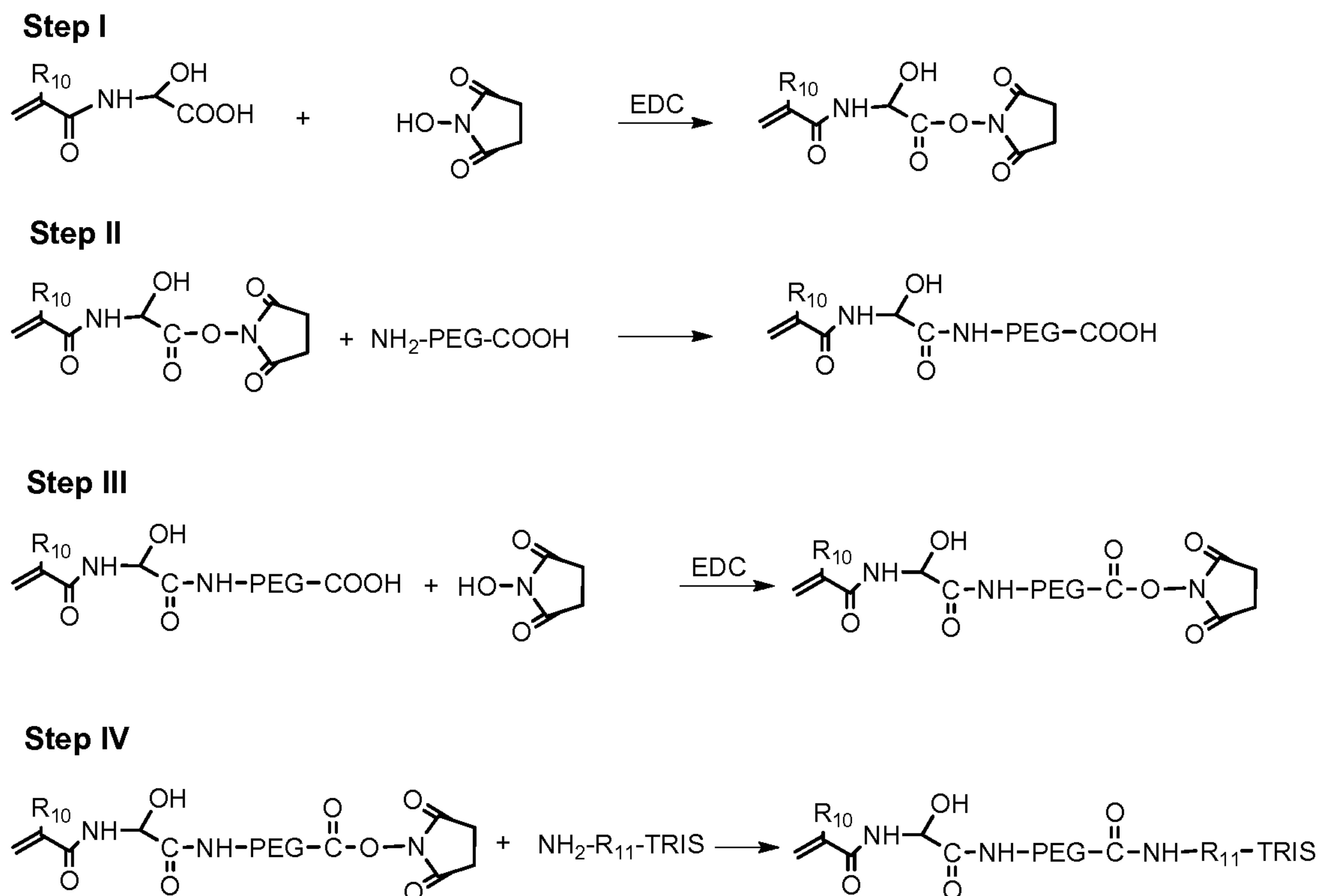
Scheme IV
