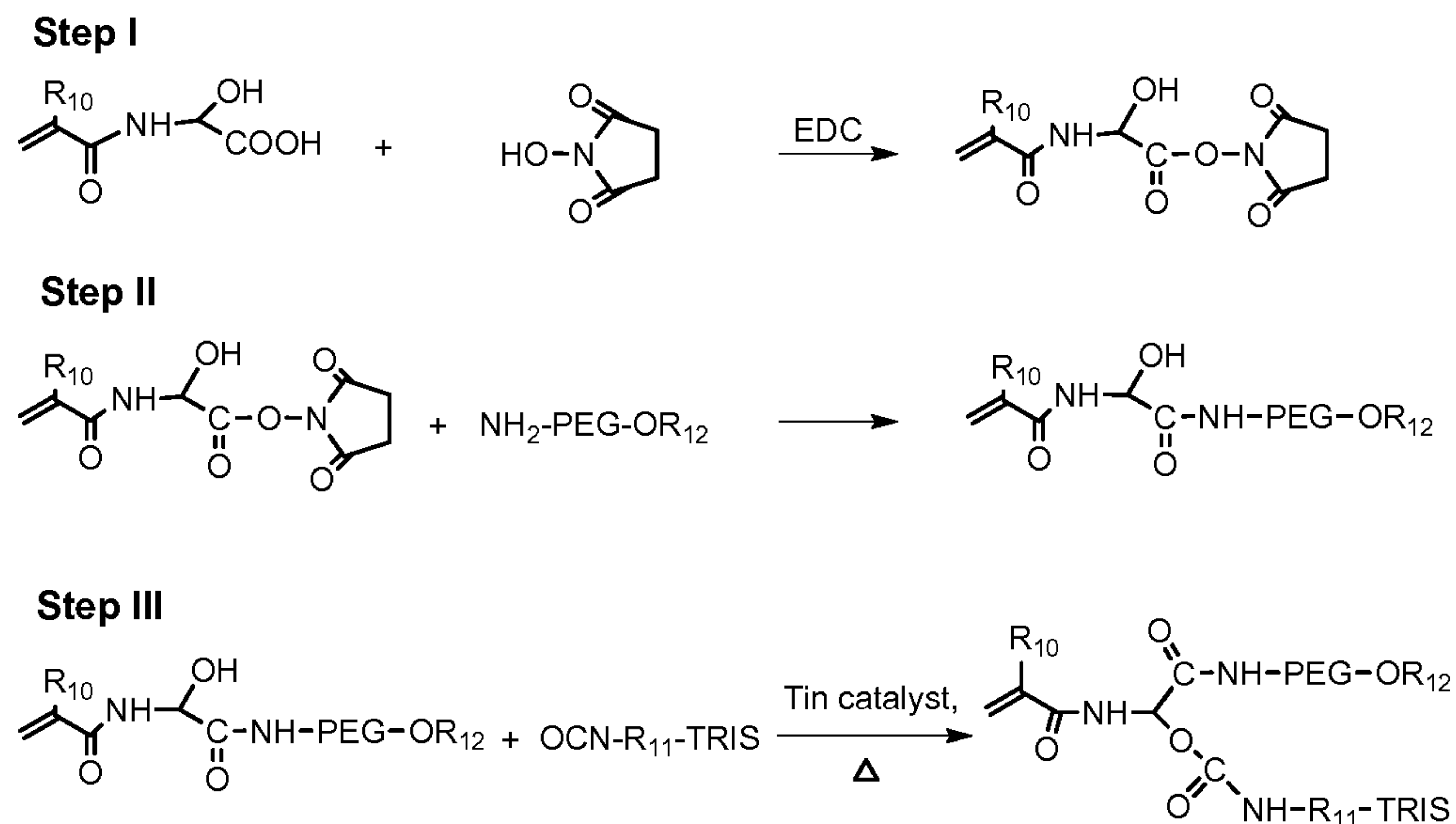
Scheme I
