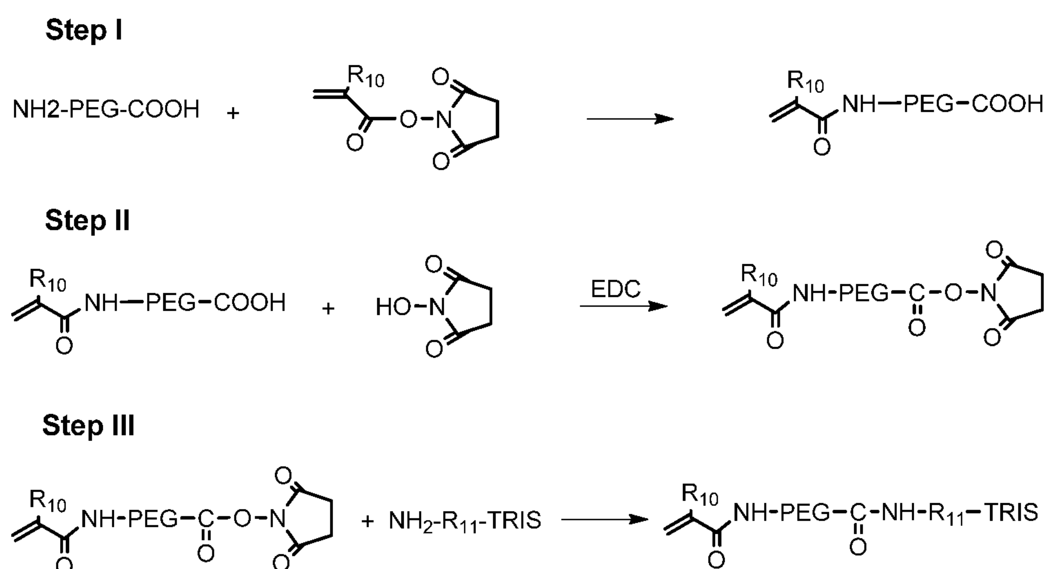
Scheme III
