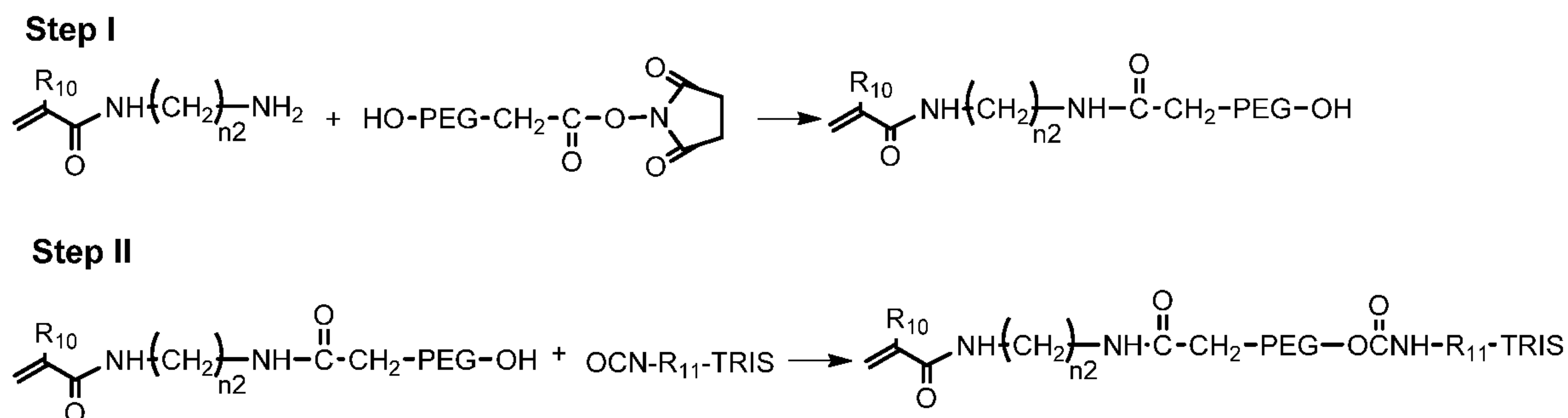
Scheme V
