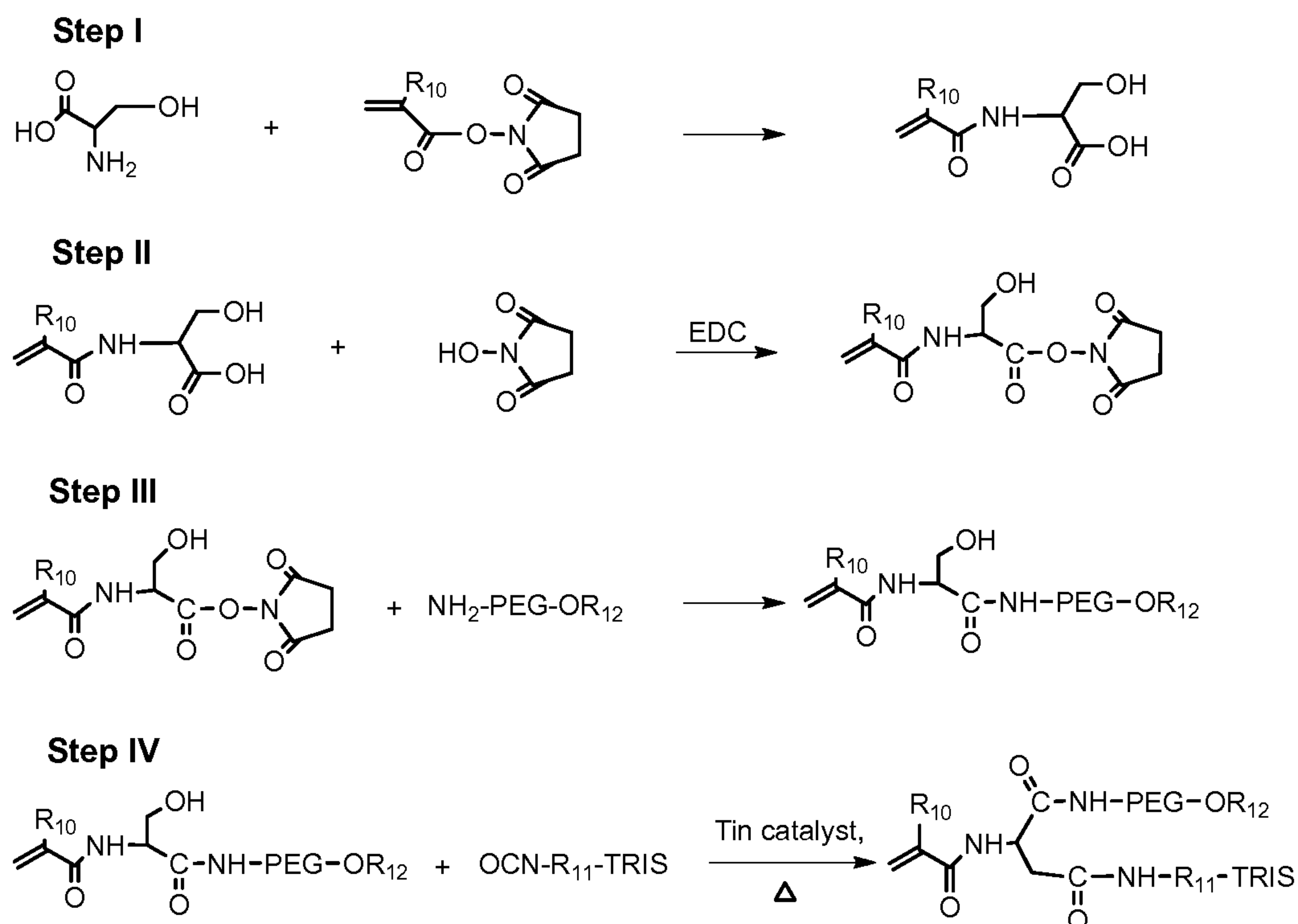
Scheme II
