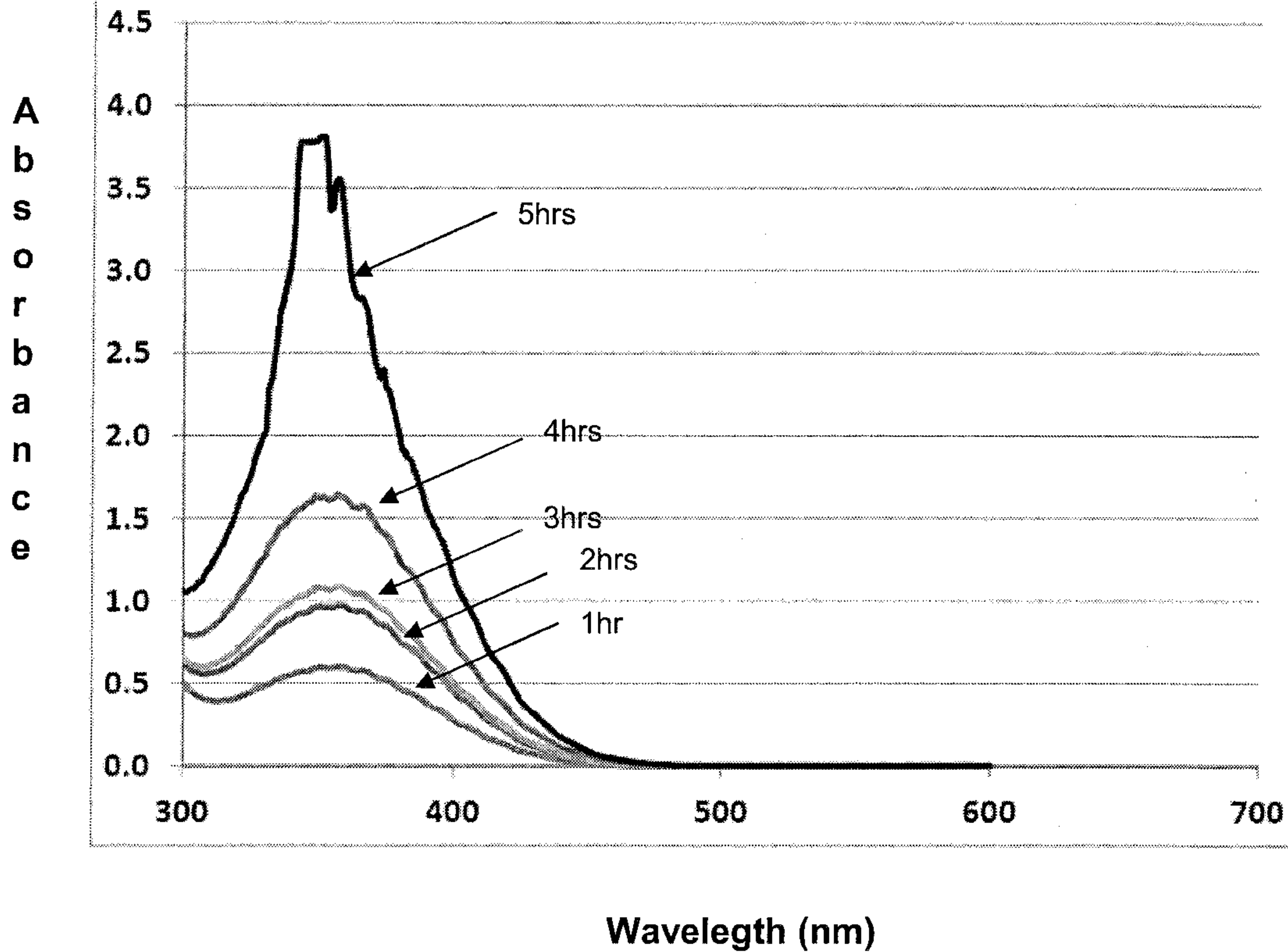
Increase in Concentration of Chlorine Dioxide (Peak Height) as a Function of Time
