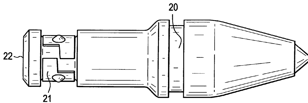
Typical Cutting Bit (Bullet Bit)
