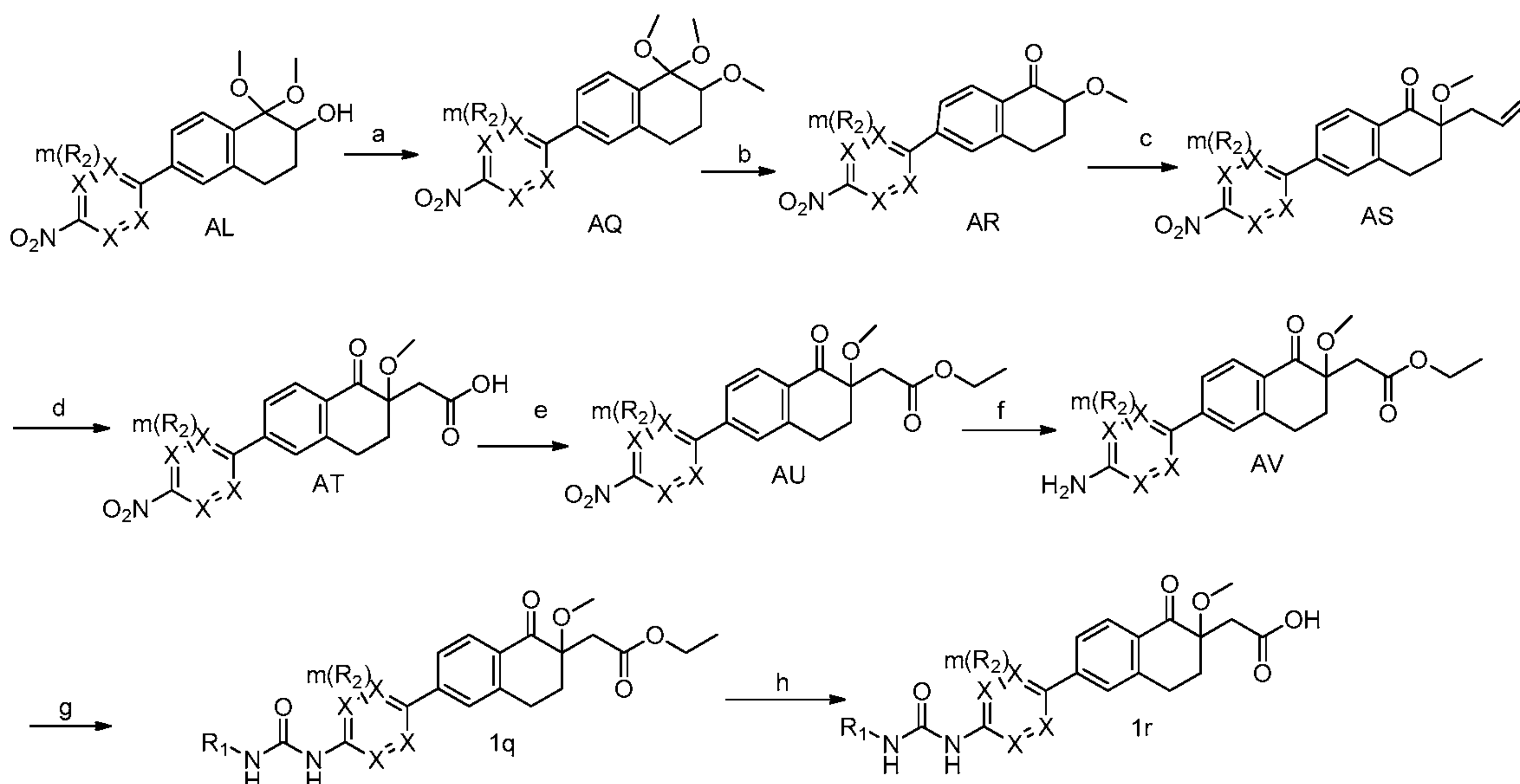
Scheme 13. Reagents and conditions: a) \text{NaH} , \text{MeI} , \text{THF} , \text{RT} ; b) 3\text{N HCl} , \text{EtOH} , \text{RT} ; c) Allyl bromide, \text{TBAI} , \text{KOH} , \text{toluene} , \text{RT} ; d) \text{KMnO}_4 , \text{NaIO}_4 , \text{RT} ; e) \text{MeSO}_3\text{H} , \text{EtOH} , \text{RT} ; f) \text{Fe-NH}_4\text{Cl} , \text{EtOH-H}_2\text{O} , 90^\circ\text{C} ; g) \text{R}_1\text{NCO} , \text{Et}_3\text{N} , \text{THF} , \text{RT} ; h) \text{LiOH} , \text{THF-H}_2\text{O} , \text{RT} , 12\text{h} .
