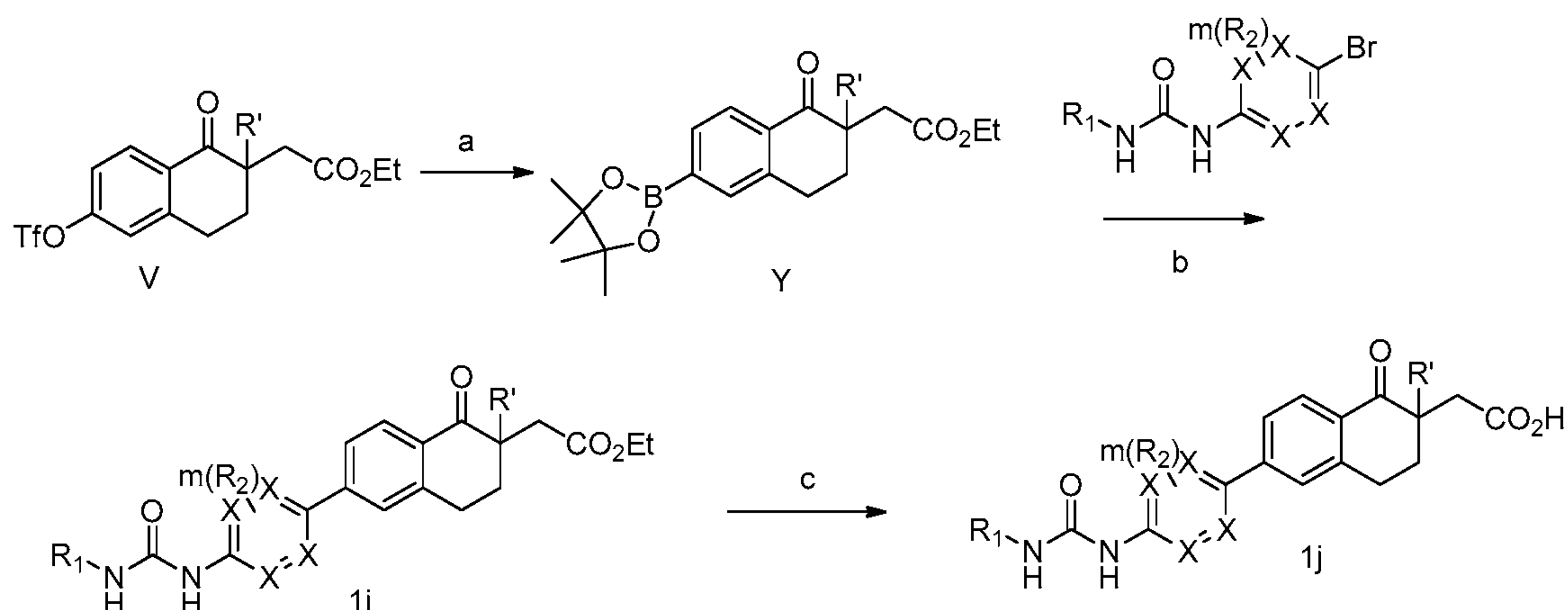
Scheme 6. Reagents and conditions: a) 4,4,4',4',5,5,5',5'-octamethyl-2,2'-bi(1,3,2-dioxaborolane), PdCl 2 (dppf), KOAc, Dioxane, 100 °C; b) Pd(PPh 3 ) 4 , Cs 2 CO 3 , Dioxane-H 2 O, 80 °C; c) LiOH, EtOH-H 2 O, RT.
