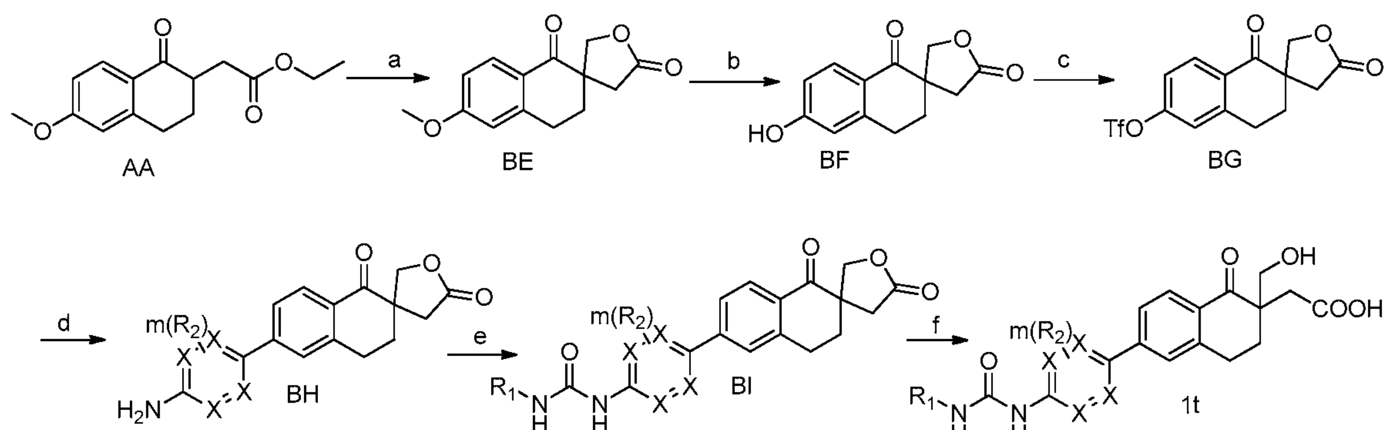
Scheme 15. Reagents and conditions: a) HCHO, 2N NaOH, THF, RT; b) Aq HBr, 100 °C; c) Tf 2 O, Py, CH 2 Cl 2 , RT; d) Pd(PPh 3 ) 4 , Cs 2 CO 3 , Dioxane-H 2 O, 80 °C; e) R 1 NCO, Et 3 N, THF, RT; f) LiOH, THF-H 2 O, RT;
