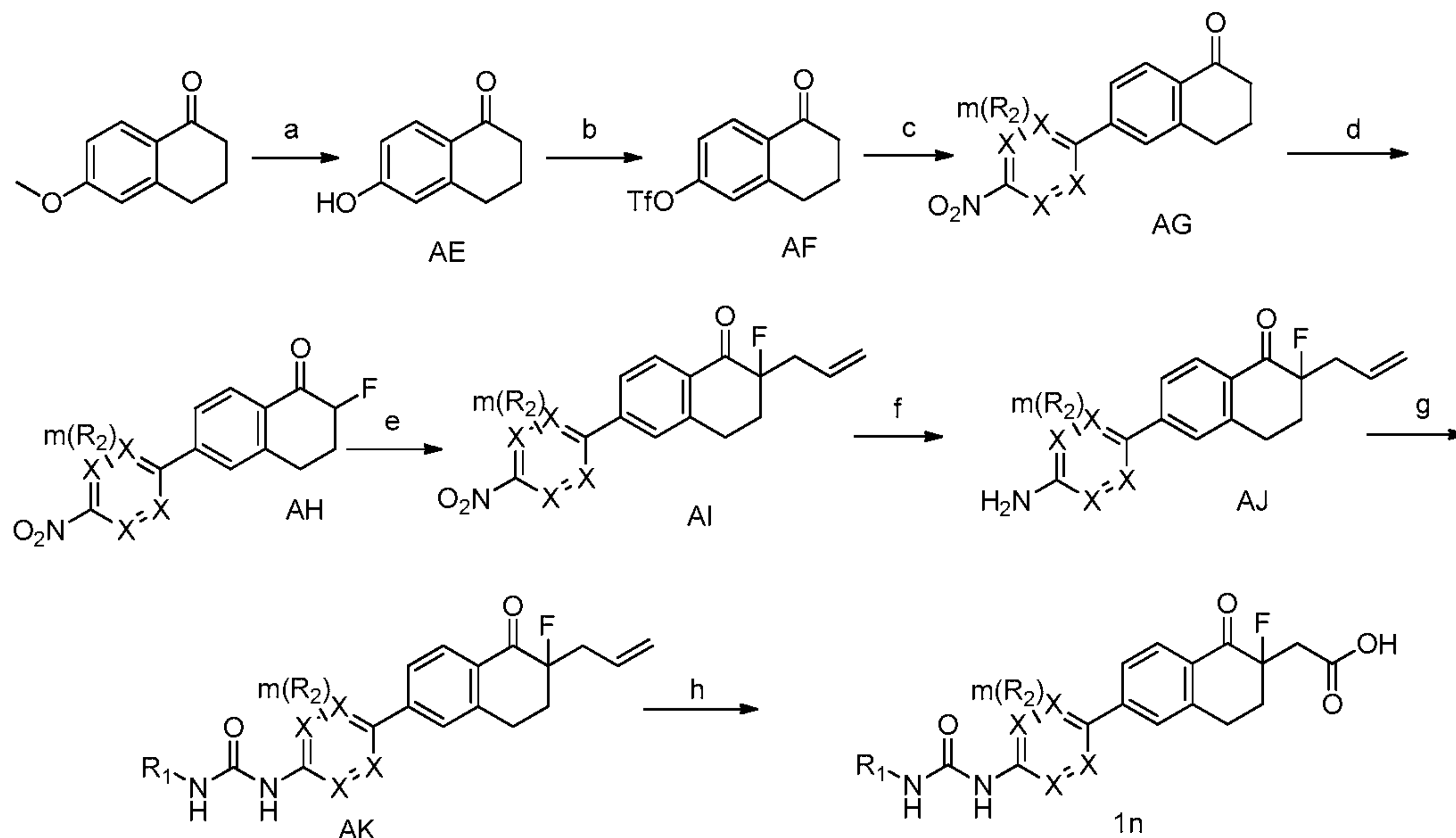
Scheme 11. Reagents and conditions: a) Aq HBr Reflux; b) \text{ Tf}_2\text{O} , DMAP, Py, RT; c) Substituted aryl/heteroaryl boronic acid or ester, \text{Pd(PPh}_3)_4 , \text{Cs}_2\text{CO}_3 , Dioxane-H 2 O, 80 °C; d) select Fluor, MeOH, 80 °C; e) Allyl bromide, TBAI, KOH, RT; f) \text{Fe/NH}_4\text{Cl} , EtOH, H 2 O, Reflux; g) \text{R}_1\text{NCO} , \text{Et}_3\text{N} , THF, RT; h) \text{KMnO}_4 , \text{NaIO}_4 , acetone-H 2 O, RT.
