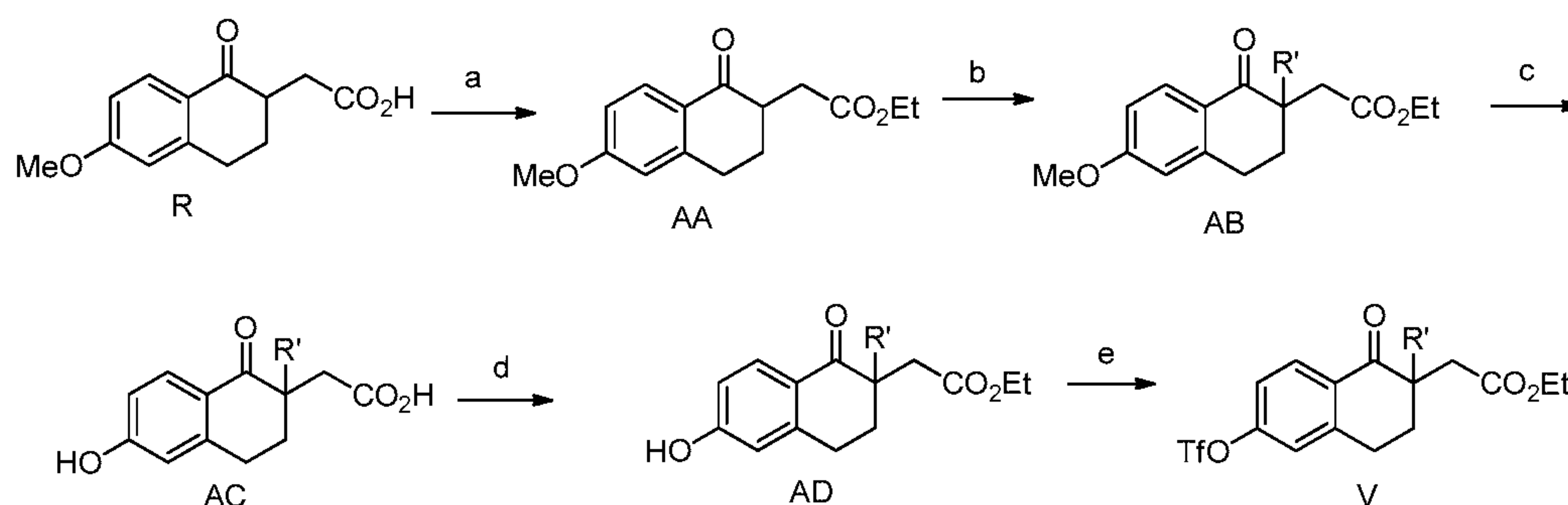
Scheme 8. Reagents and conditions: a) \text{MeSO}_3\text{H} , EtOH, RT; b) \text{R}'\text{-X} , NaH, DMF, RT; c) Aq. HBr, 100^\circ\text{C} ; d) \text{MeSO}_3\text{H} , EtOH, RT; e) \text{Tf}_2\text{O} , \text{CH}_2\text{Cl}_2 , \text{Et}_3\text{N} , RT.
