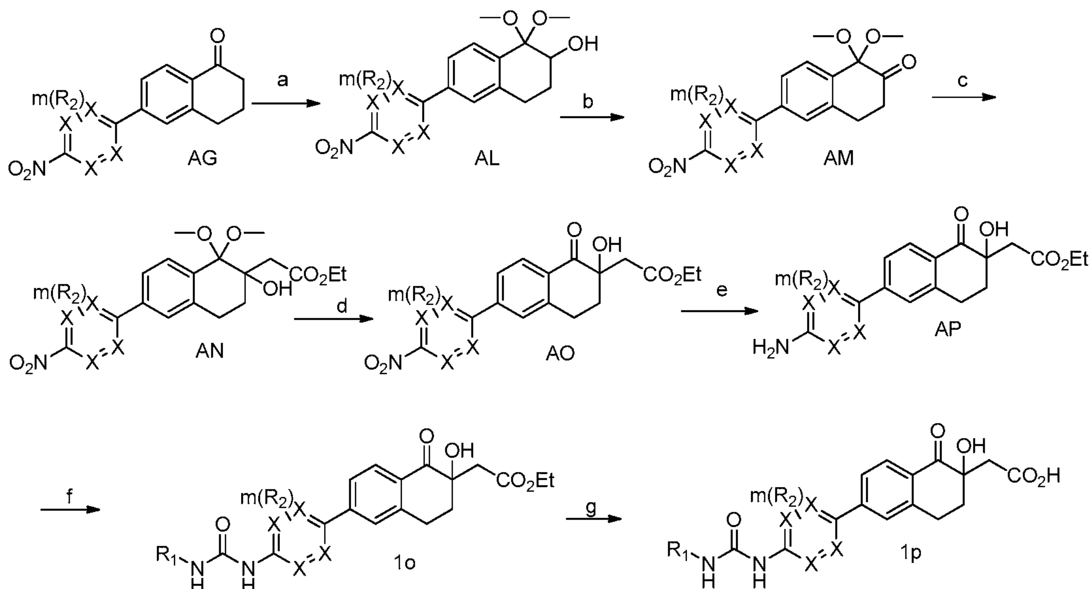
Scheme 12. Reagents and conditions: a) \text{PhI}(\text{OAc})_2 , \text{KOH} , \text{MeOH} , \text{RT} ; b) Pyridinium dichromate, \text{AcOH} , \text{CH}_2\text{Cl}_2 , \text{RT} ; c) \text{LiHMDS} , \text{EtOAc} , \text{THF} , 0^\circ\text{C} to \text{RT} ; d) 3\text{N HCl} , \text{MeOH} , \text{RT} ; e) \text{Pd/C} , \text{H}_2 , \text{EtOH} , \text{RT} ; f) \text{R}_1\text{NCO} , \text{Et}_3\text{N} , \text{THF} , \text{RT} ; g) \text{LiOH} , \text{MeOH-THF-H}_2\text{O} , \text{RT} .
