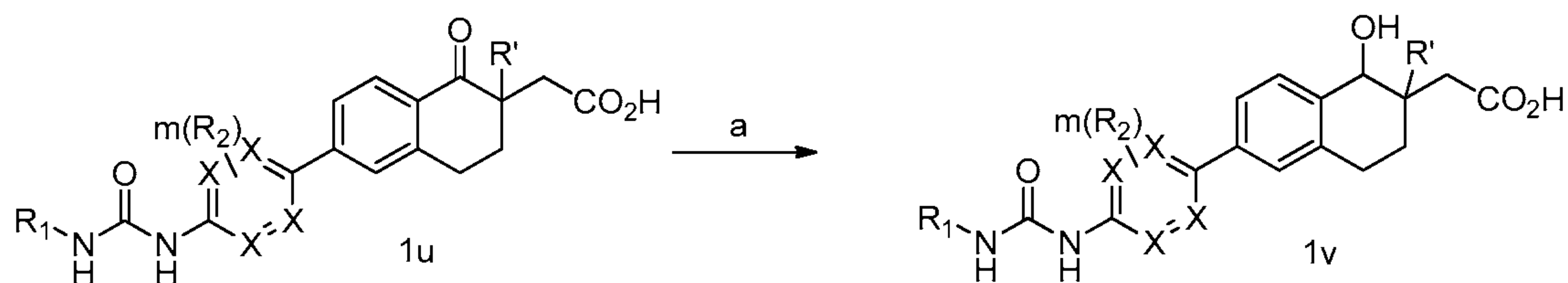
Scheme 16. Reagents and conditions: a) NaBH 4 , MeOH, RT.
