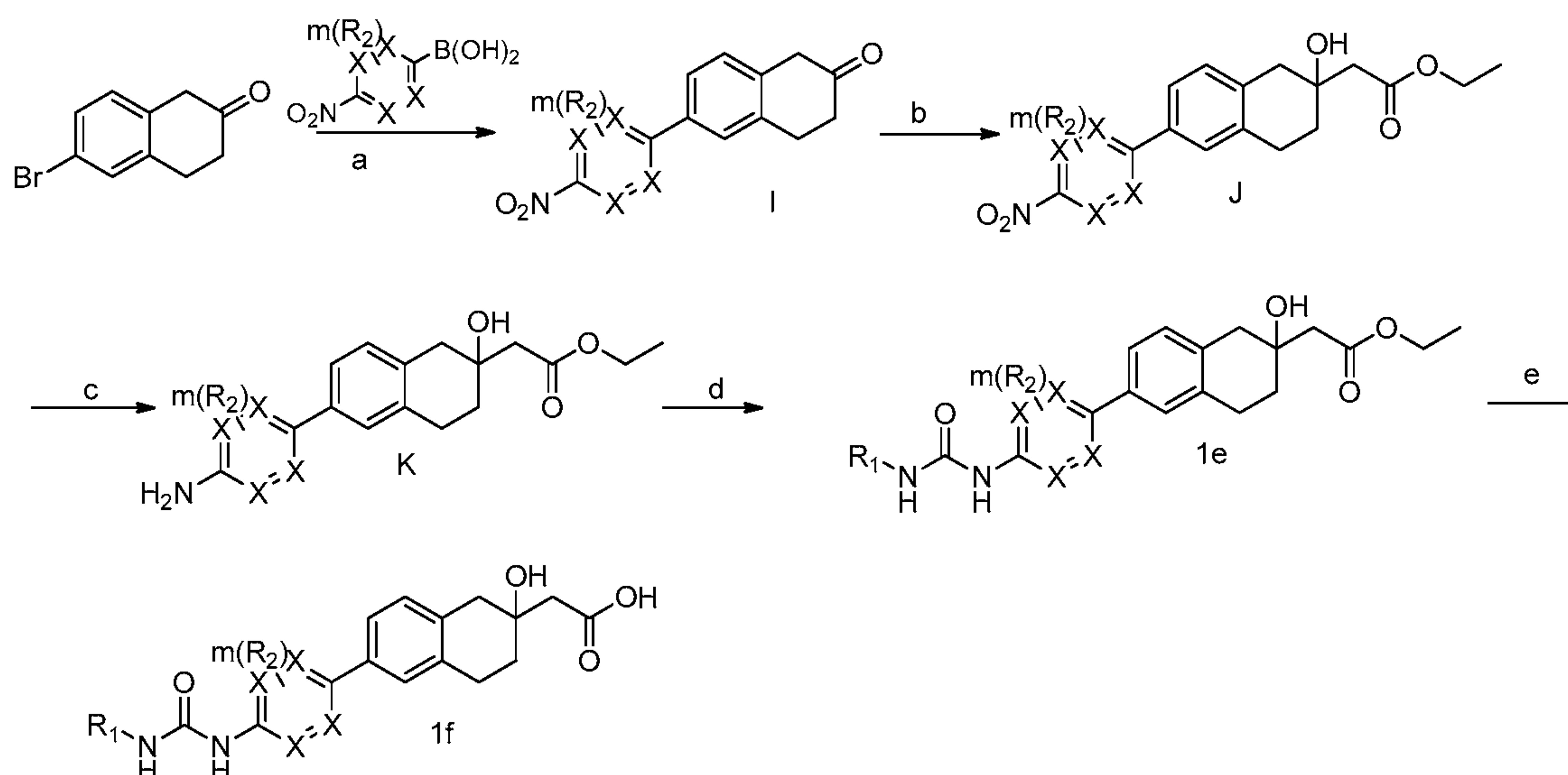
Scheme 3. Reagents and conditions: a) Pd(PPh 3 ) 4 , Cs 2 CO 3 , Dioxane-H 2 O, 80 °C; b) EtOAc, LiHMDS, THF, -78 °C to RT; c) Pd/C, MeOH, H 2 , RT; d) R 1 NCO, Et 3 N, THF, RT; e) NaOH, MeOH-THF-H 2 O, RT.
