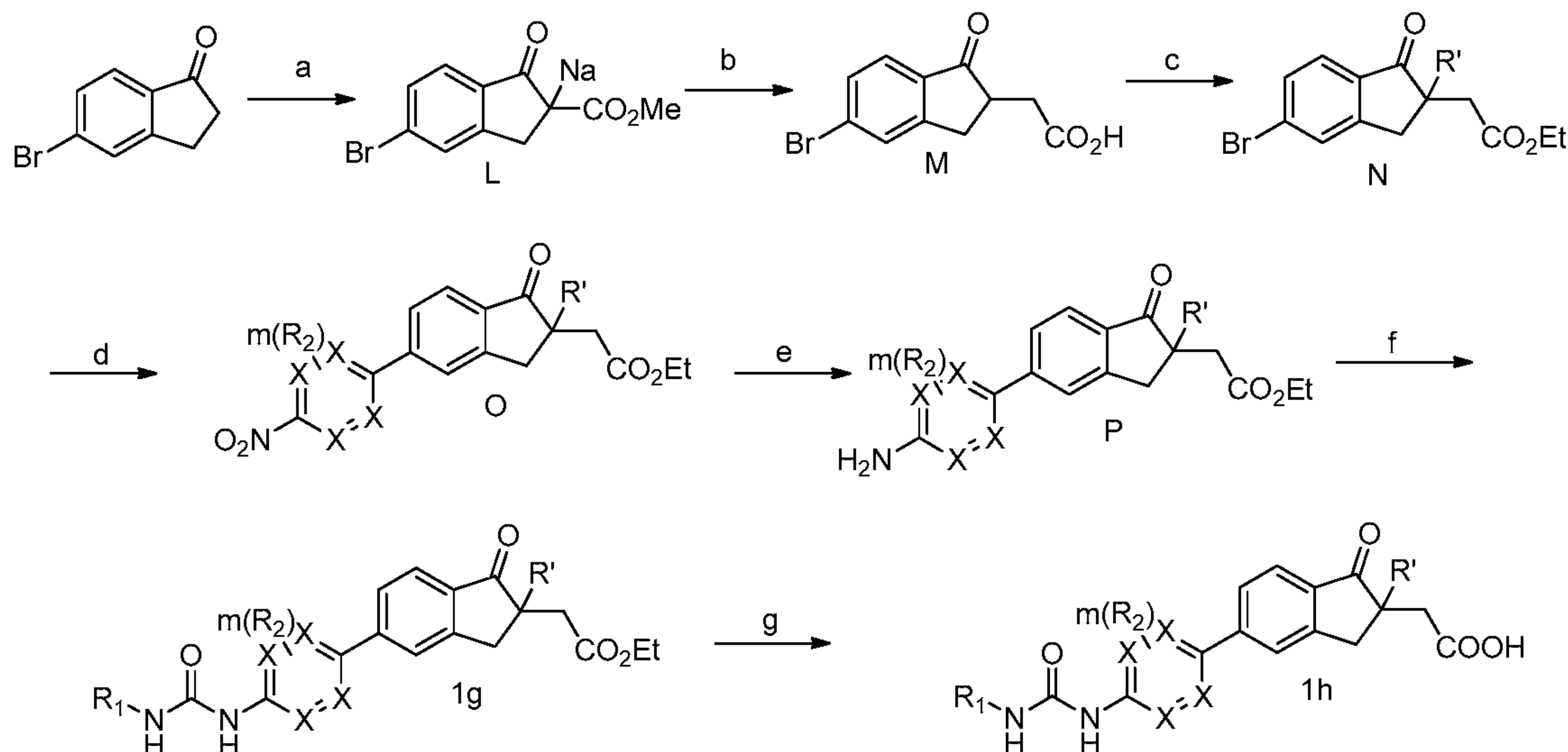
Scheme 4. Reagents and conditions: a) CO(OMe)_2 , NaH, THF, 75 °C; b) BrCH_2COOEt , THF, 75 °C; c) NaH, R'-X , DMF, RT; d) substituted boronic acid/ester, Pd(PPh_3)_4 , Cs_2CO_3 , Dioxane- H_2O , 80 °C; e) Fe/NH_4Cl , EtOH- H_2O , 85 °C; f) R_1NCO , Et_3N , THF, RT; g) LiOH, Dioxane- H_2O , RT.
