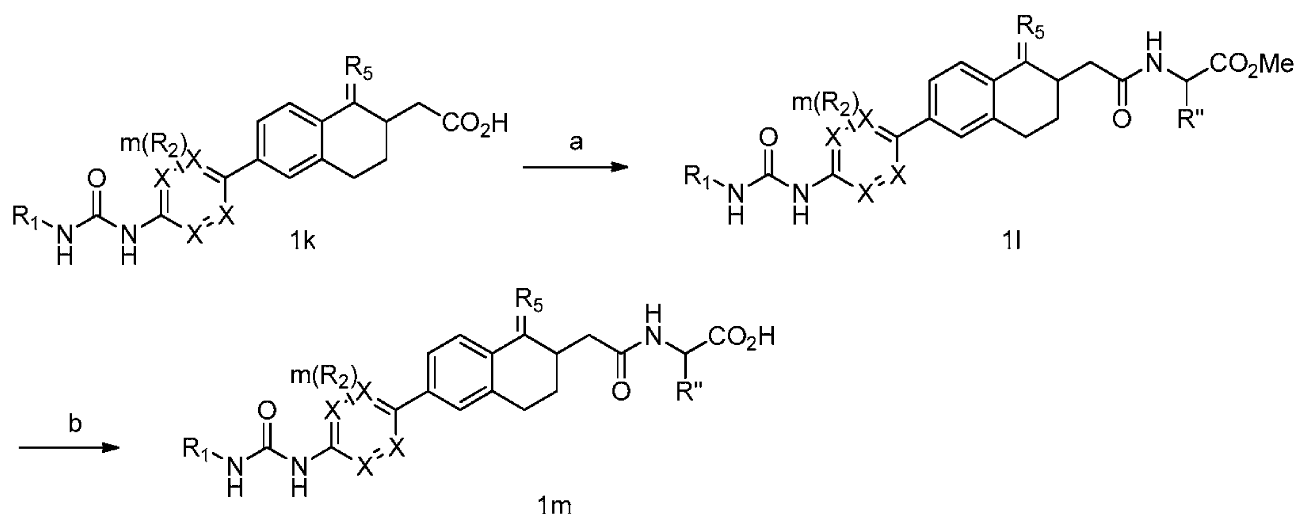
Scheme 10. Reagents and conditions: a) HATU, THF, amino acid methyl ester ( \text{NH}_2\text{-CH(R'')CO}_2\text{Me} ), RT; b) LiOH, THF-H 2 O, RT.
