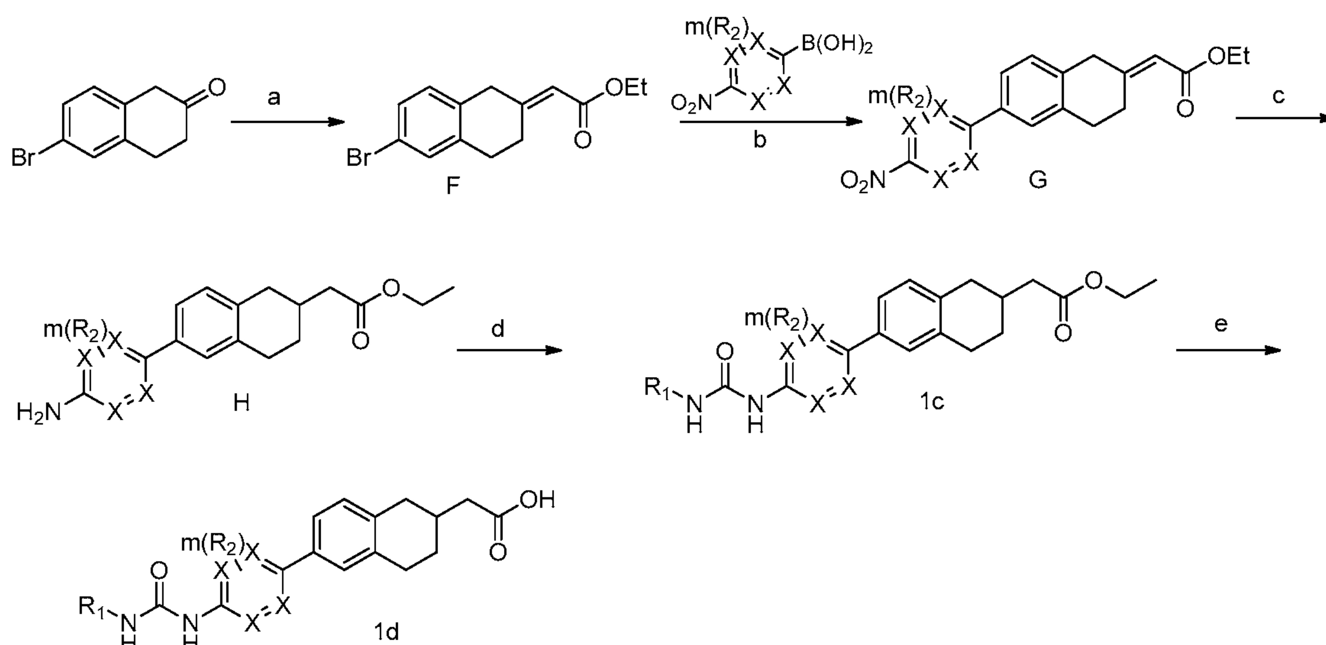
Scheme 2. Reagents and conditions: a) Ph 3 P=CHCO 2 Et, NaH, DMF, RT; b) Pd(PPh 3 ) 4 , Cs 2 CO 3 , Dioxane-H 2 O, 80 °C; c) Pd/C, MeOH, H 2 , RT; d) R 1 NCO, Et 3 N, THF, RT; e) LiOH, THF-H 2 O, RT.
