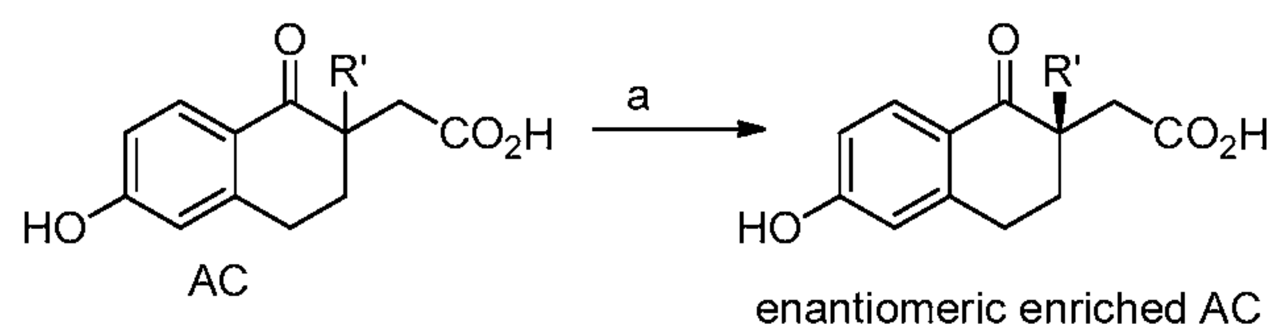
Scheme 9. Reagents and conditions: a) Cinchonidine, IPA- \text{H}_2\text{O} , 80^\circ\text{C} – RT, 24h then 6N HCl.
