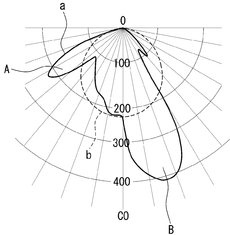
FIG. 12 Prior Art
