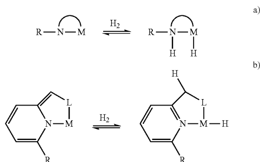
MLC in (a) metal-amide- metal-amine ligand transformation. (b) aromatization-dearomatization of pyridine based ligands.
