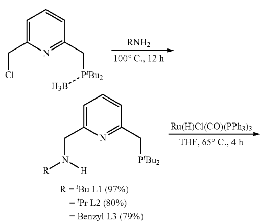
Scheme 28. Synthesis of PNN-H ligands and their corresponding Ru (II) complexes.
