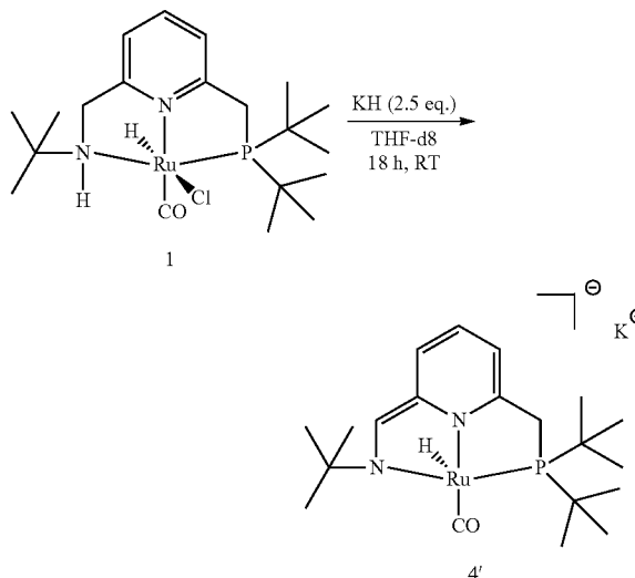
Scheme 29. Preparation of the monoanionic complex 4' by double deprotonation of 1.
