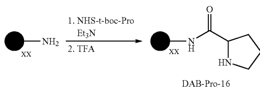
Scheme 7. Preparation of DAB-Pro-16.
