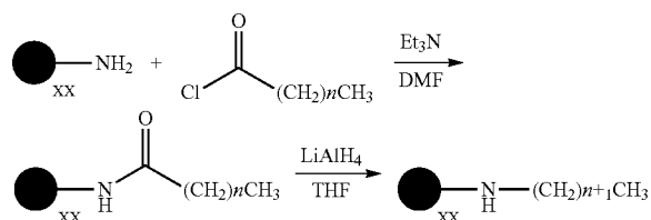
Scheme 3. General procedure for dendrimers with lipophilic tails.
