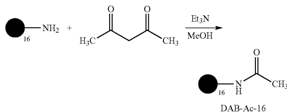
Scheme 6. Preparation of DAB-Ac-16.
