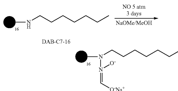
Scheme 5. Preparation of DAB-C7-16 diazeniumdiolate.
