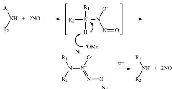
Scheme 1. Synthesis and NO-release from N-diazoniumdiolates.
