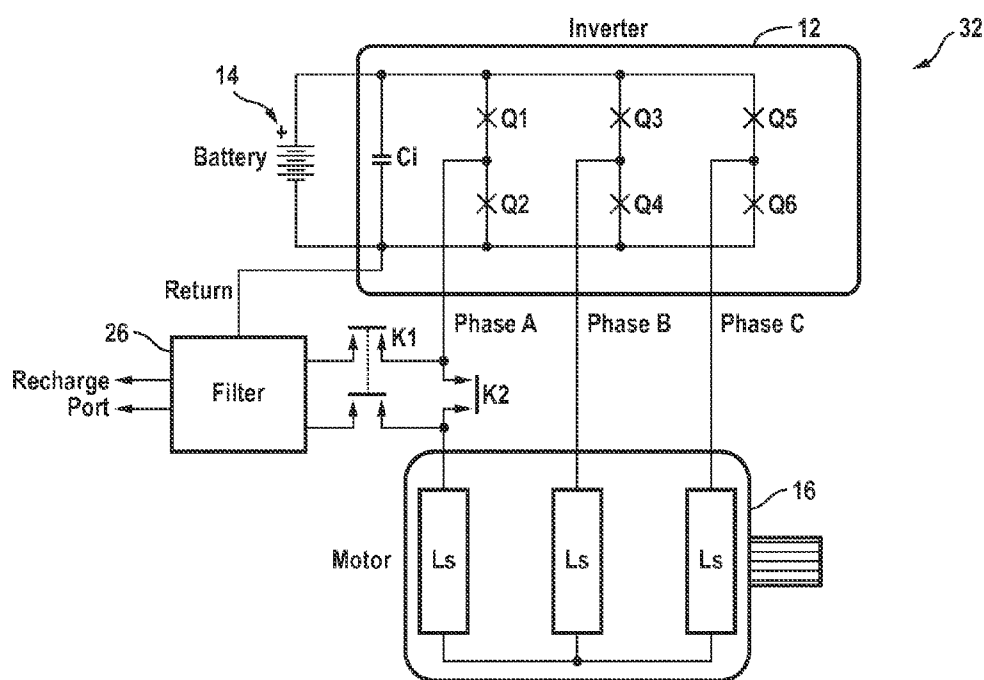
FIG. 3 (Prior Art)
