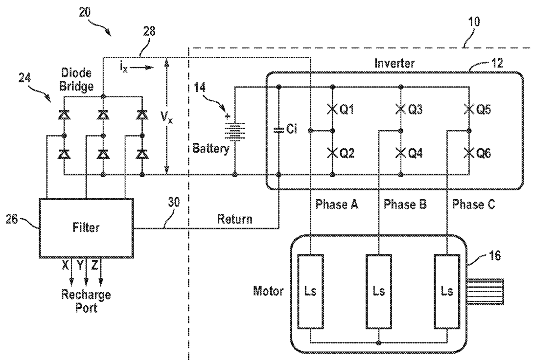
FIG. 2 (Prior Art)
