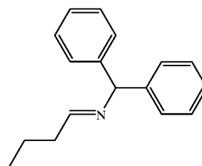
N-Propylidene-1,1-diphenylmethanimine (8h) Light yellow oil.
