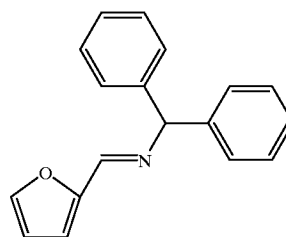
N-(Furan-2-ylmethylidene)-1,1-diphenylmethanimine (8g) 14 White crystal,
