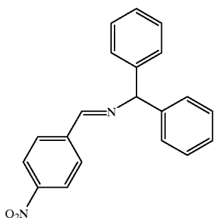
N-(4-Nitrobenzylidene)-1,1-diphenylmethanimine (8c) 15 Off-white crystal.
