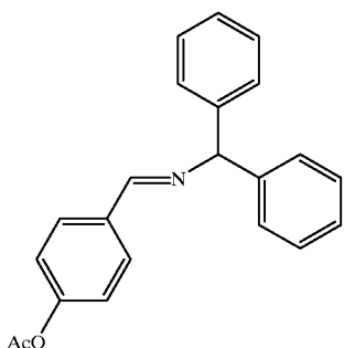
N-(4-Acetoxybenzylidene)-1,1-diphenylmethanimine (8d) 16 White crystal.
