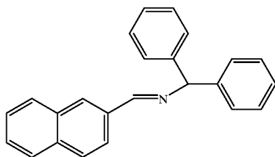
N-(2-Naphthylidene)-1,1-diphenylmethanimine (8f) White crystal.
