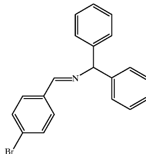
N-(4-Bromobenzylidene)-1,1-diphenylmethylamine (8b) 15 White crystal.
