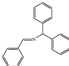
N-Benzylidene-1,1-diphenylmethylamine (8a) 14 White crystal.
