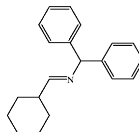
N-(Cyclohexylmethylidene)-1,1-diphenylmethanimine (8i) 14 White crystal.
