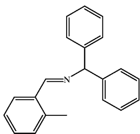
N-(o-Tolylbenzylidene)-1,1-diphenylmethanimine (8e) White crystal.
