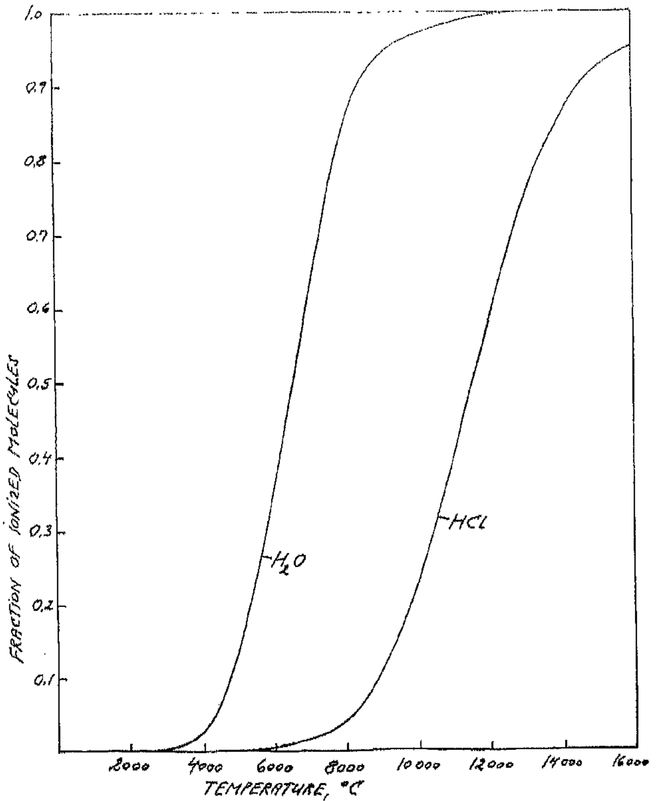
The thermal ionization of water vapor and hydrogen chloride vapor at atmospheric pressure.
