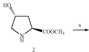
Scheme 1. Synthesis of compounds 10-48.
