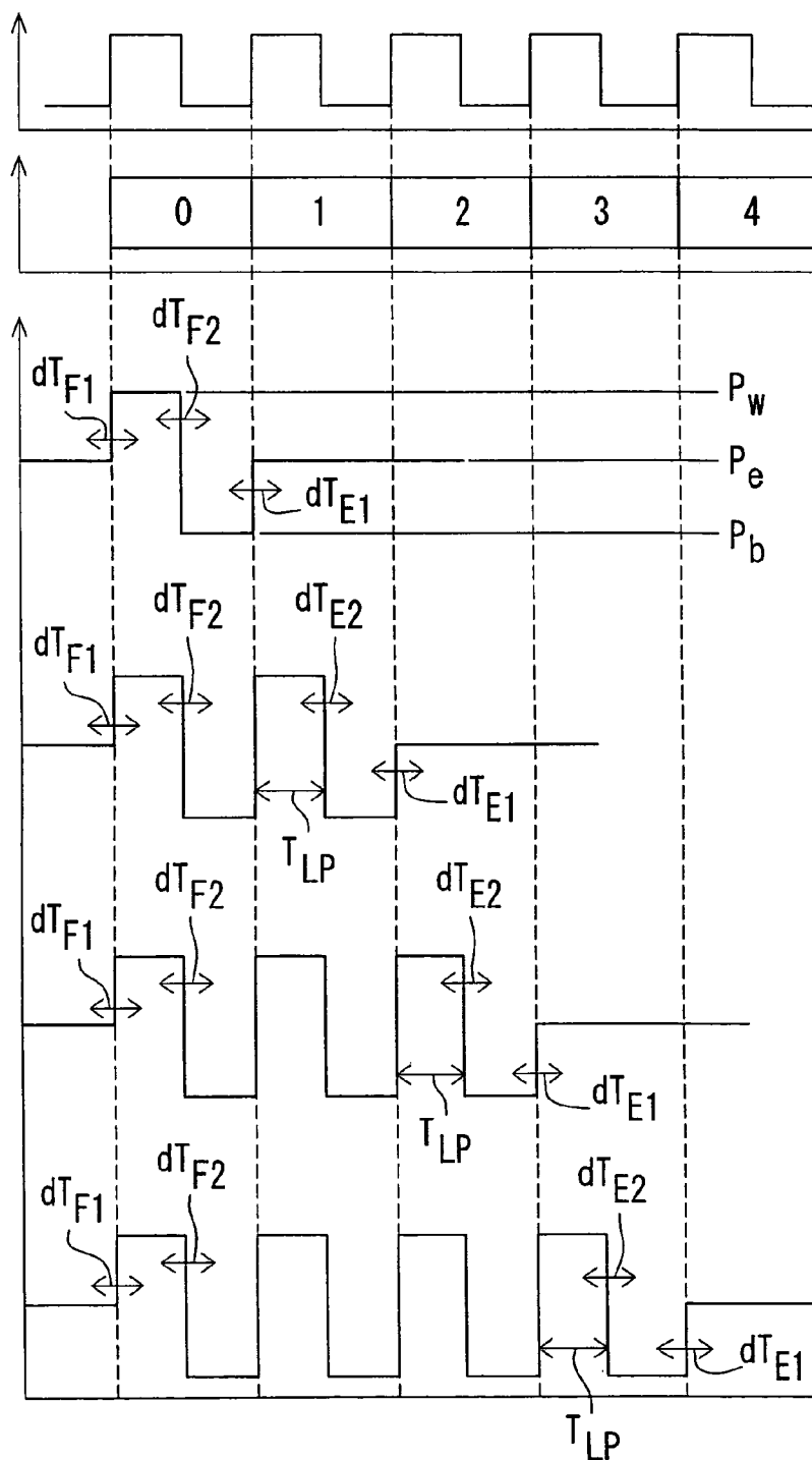
Fig. 9A 128 REFERENCE-TIME SIGNAL
