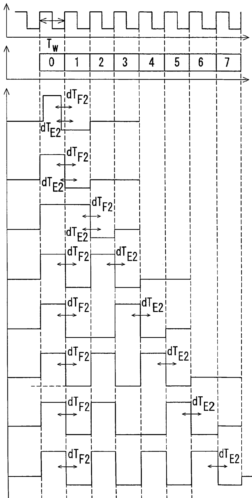
Fig. 10A 128 REFERENCE-TIME SIGNAL
