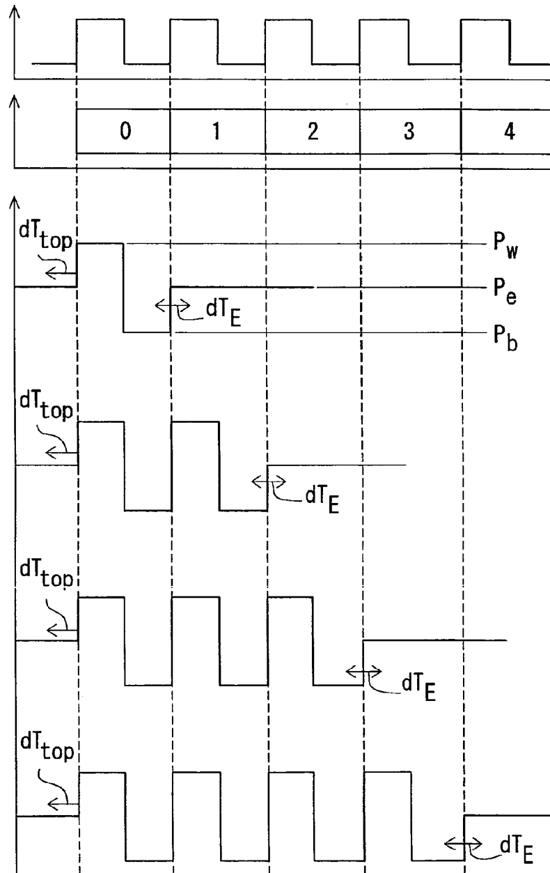
Fig. 14B 205 COUNT SIGNAL
