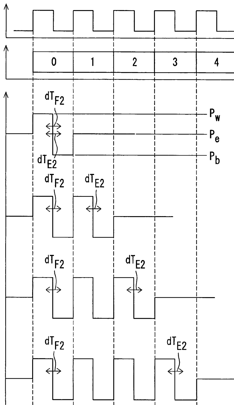
Fig. 3A 128 REFERENCE-TIME SIGNAL
