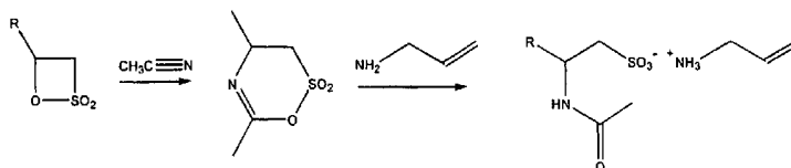
Scheme VII: 2-Acetamidoalkyl-1-Sulfonic Acid Allyl Amine Salts
