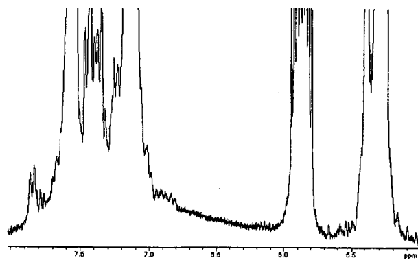
Figure I: Partial ^1\text{H} NMR Spectrum of ADDBS
