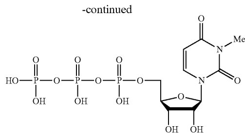
NTP of compound 44 C_{10}H_{17}N_2O_{15}P_3 Exact Mass: 497.98
