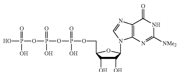
NTP of compound 50 C_{12}H_{20}N_5O_{14}P_3 Exact Mass: 551.02
