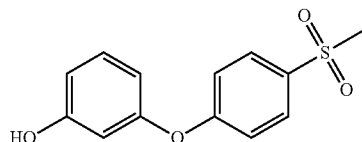
Intermediate 15: 3-(4-Methanesulfonyl-phenoxy)-phenol
