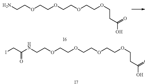
1-iodo-2-oxo-6,9,12,15-tetraoxa-3-azaocetadecan-18-oic acid (17)
