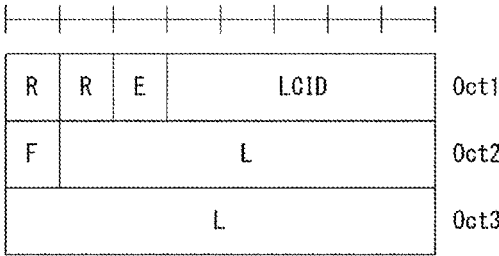
(b) R/R/E/LCID/F/L sub-header with 15-bit L field
