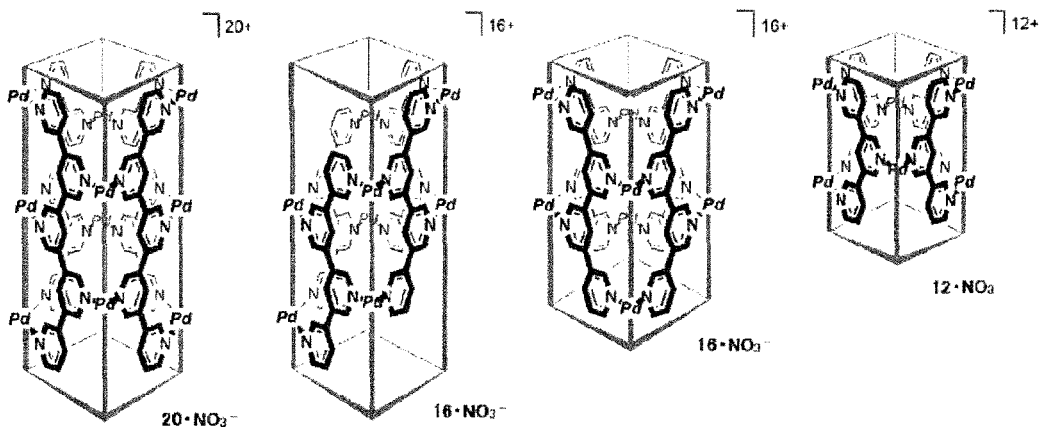
Tube-type metal complex (palladium)
