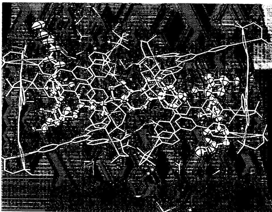
Methyl cholate
