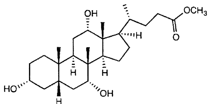
Methyl cholate
