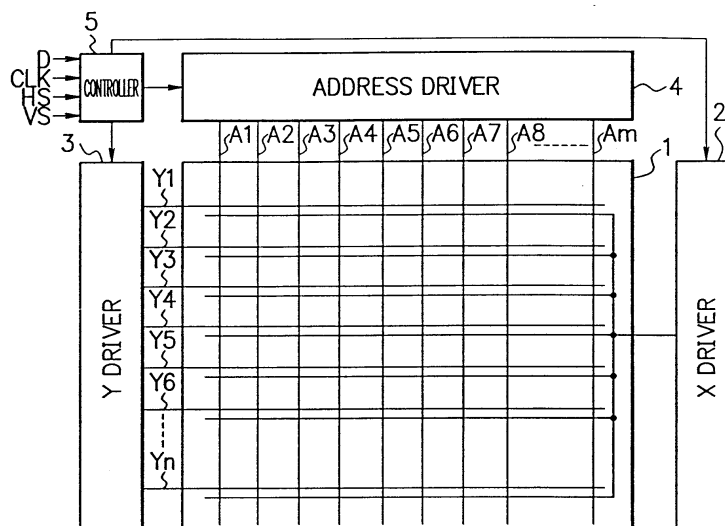
AC DRIVING TYPE PLASMA DISPLAY APPARATUS
