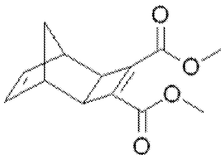
dimethyl exo-tricyclo(4.2.1.0(2.5)nona-3,7-diene)-3,4-dicarboxylate
