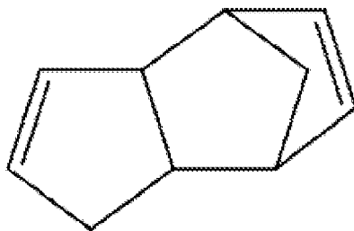
dicyclopentadiene
