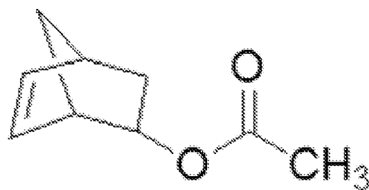
5-norbornene-2-yl acetate
