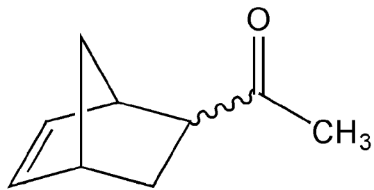
2-acetyl-5-norbornene
