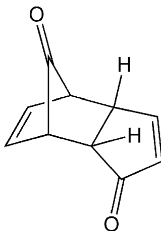
3a,4,7,7a-tetrahydro-4,7-methano-indene-1,8-dione
