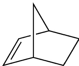
norbornene
