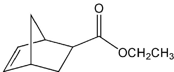
ethyl 5-norbornene-2-carboxylate
