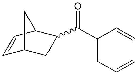
2-benzoyl-5-norbornene
