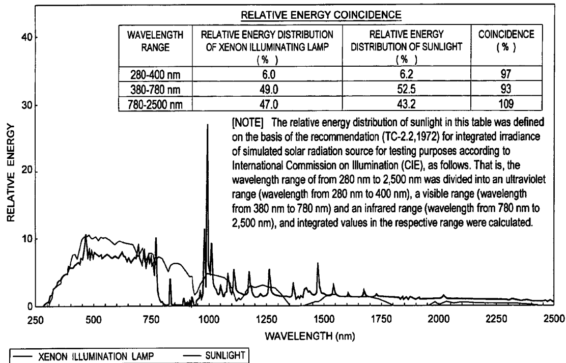
SPECTRAL DISTRIBUTION OF XENON ILLUMINATING LAMP AND SUNLIGHT
