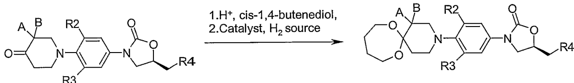
Scheme-7
