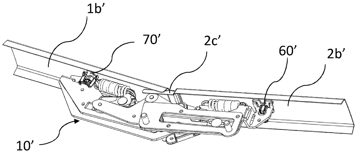
Fig. 2 (Prior art)
