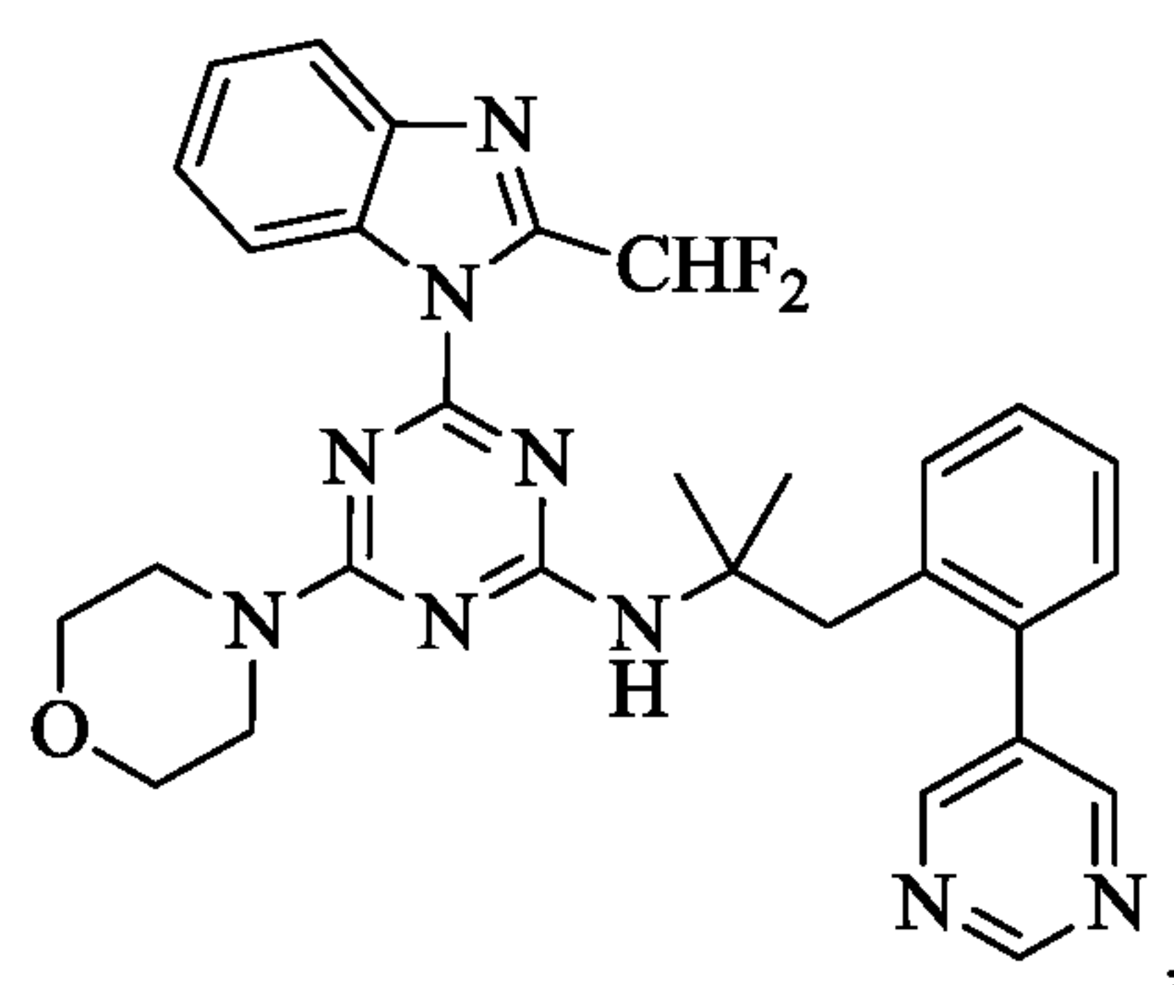
Compound XII
