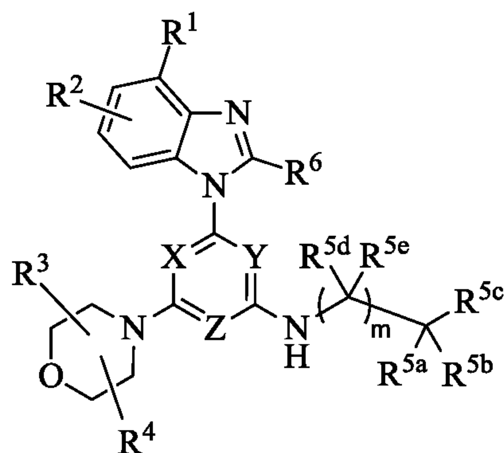
Formula (I)
