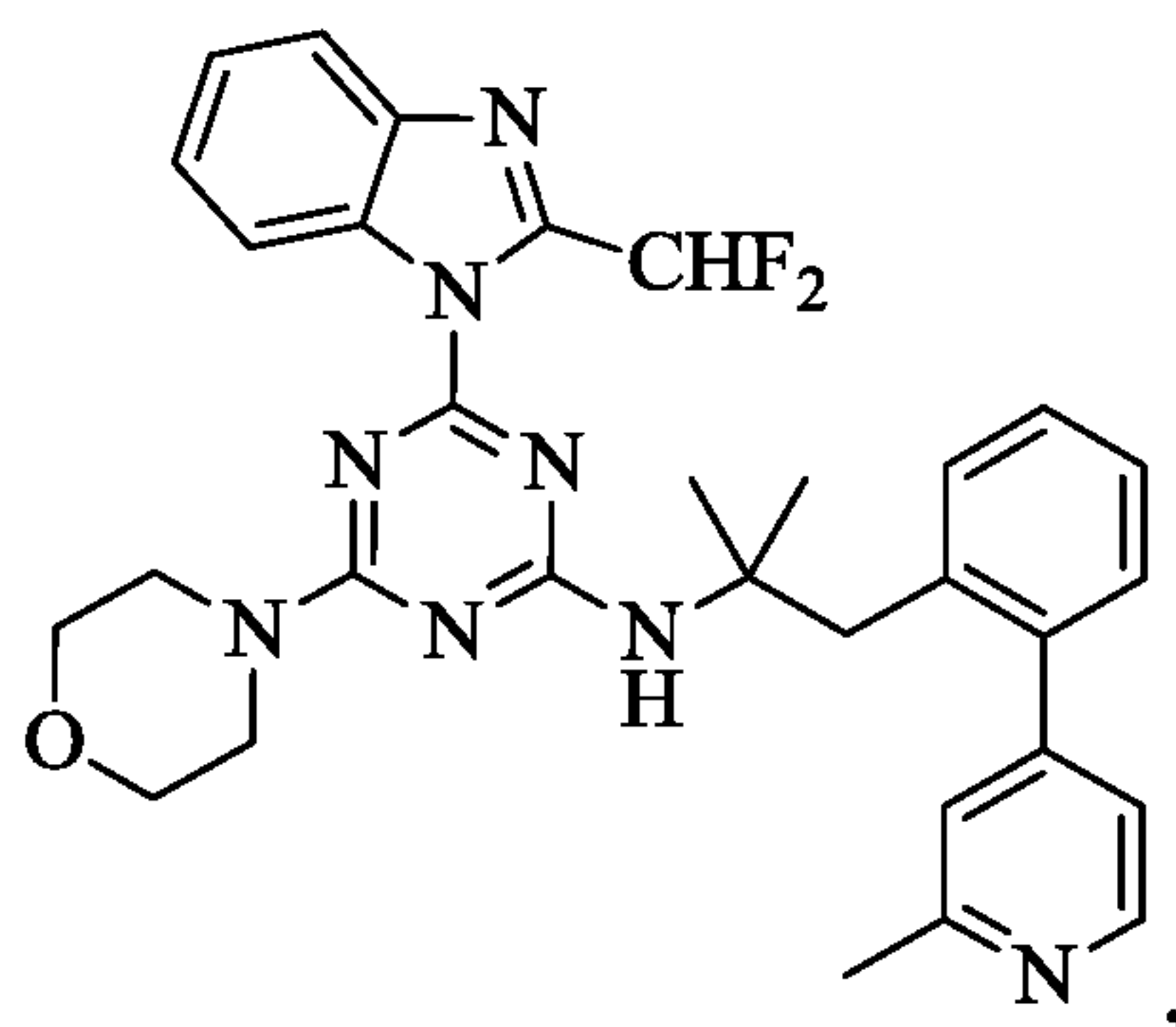
Compound IX
