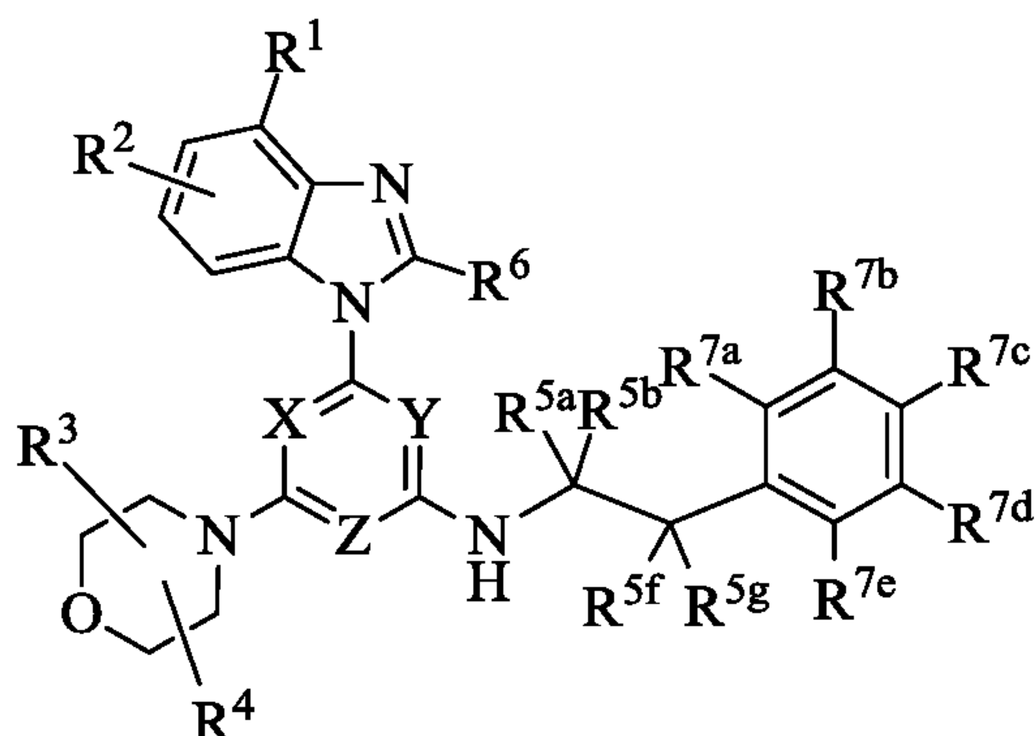
Formula (XI),
