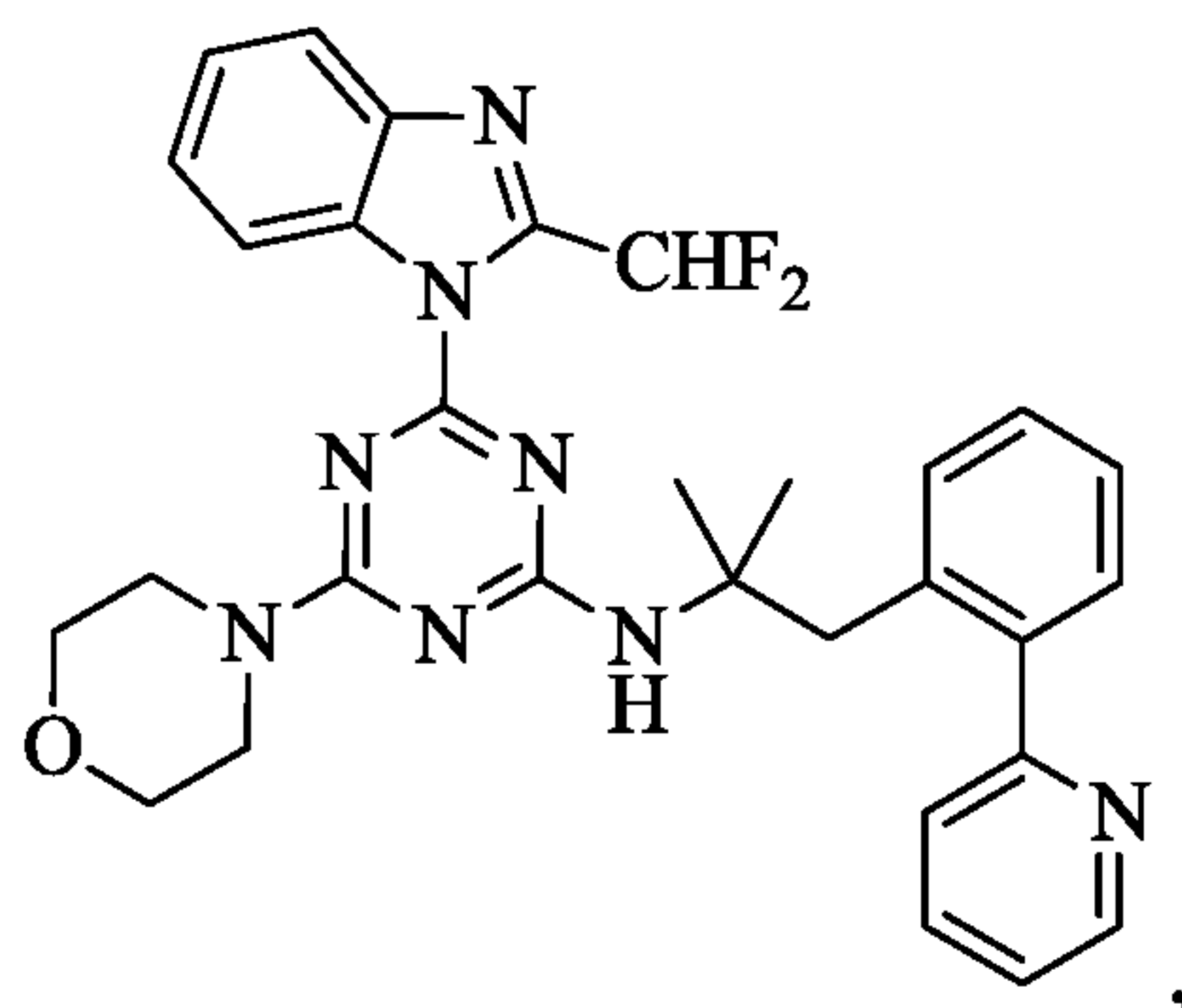
Compound VIII
