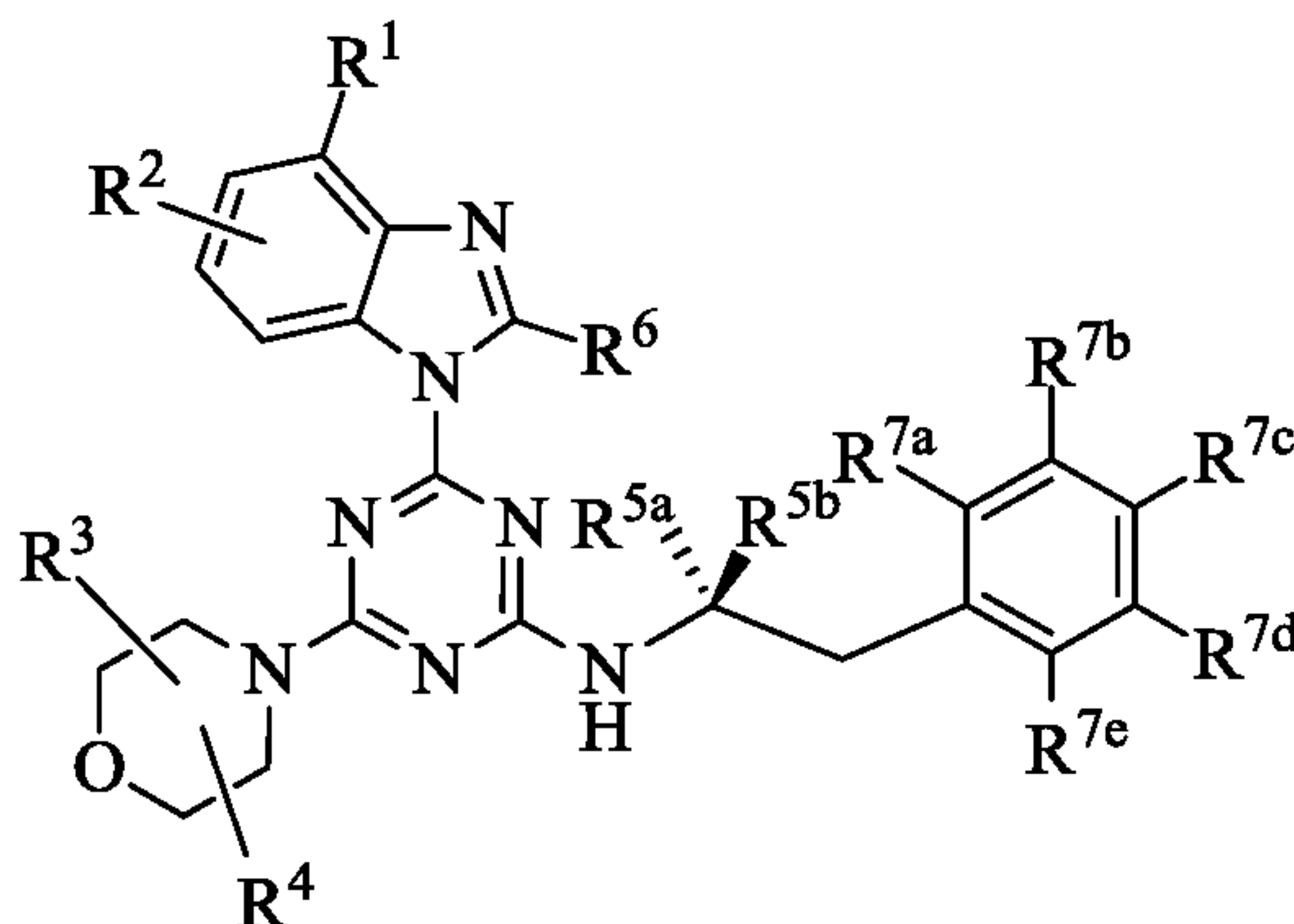
Formula (XVIb)
