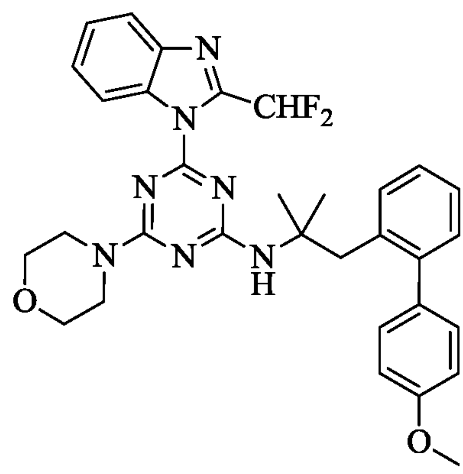
Compound XVI
