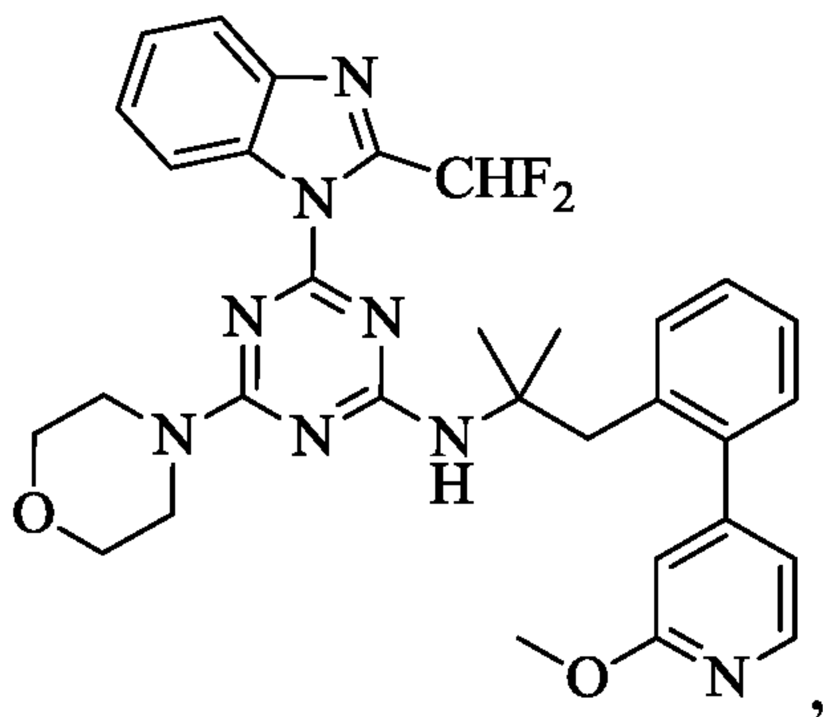
Compound VII
