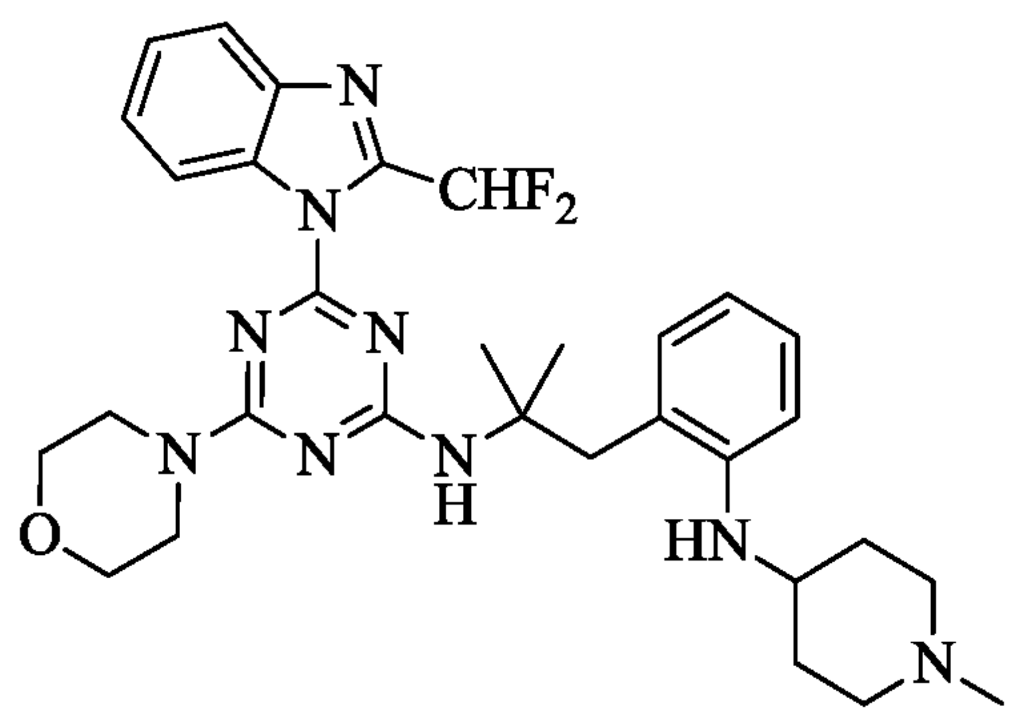
Compound V
