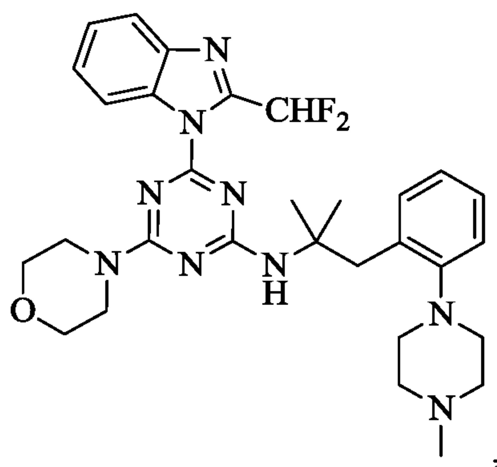
Compound II
