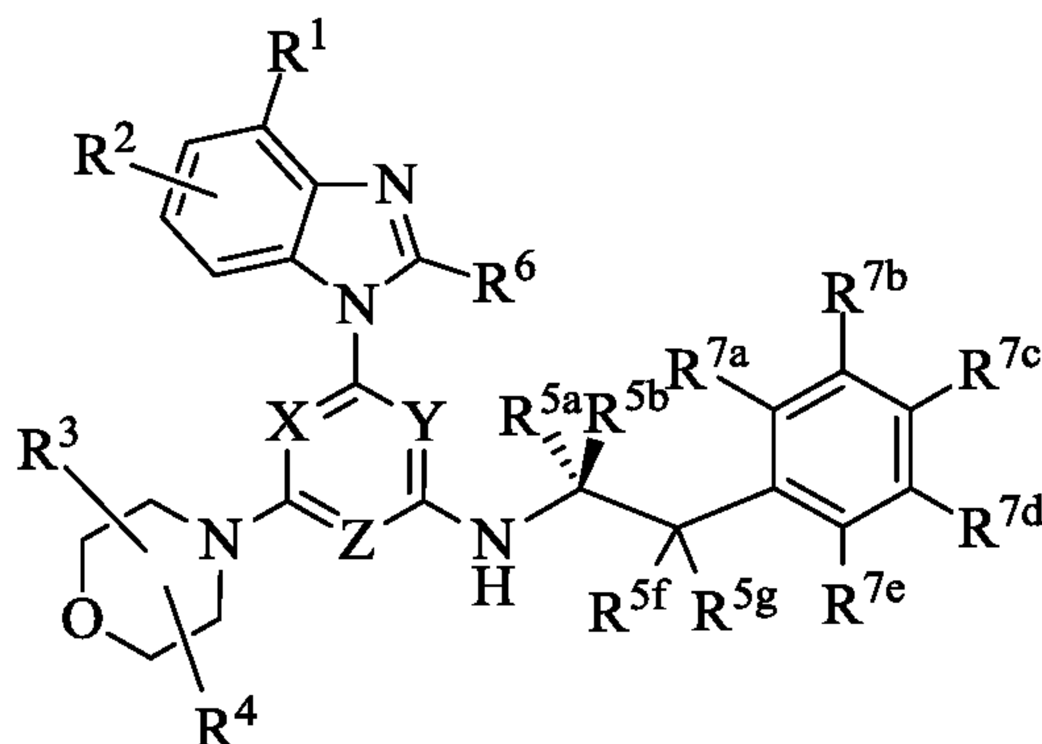
Formula (XIb),
