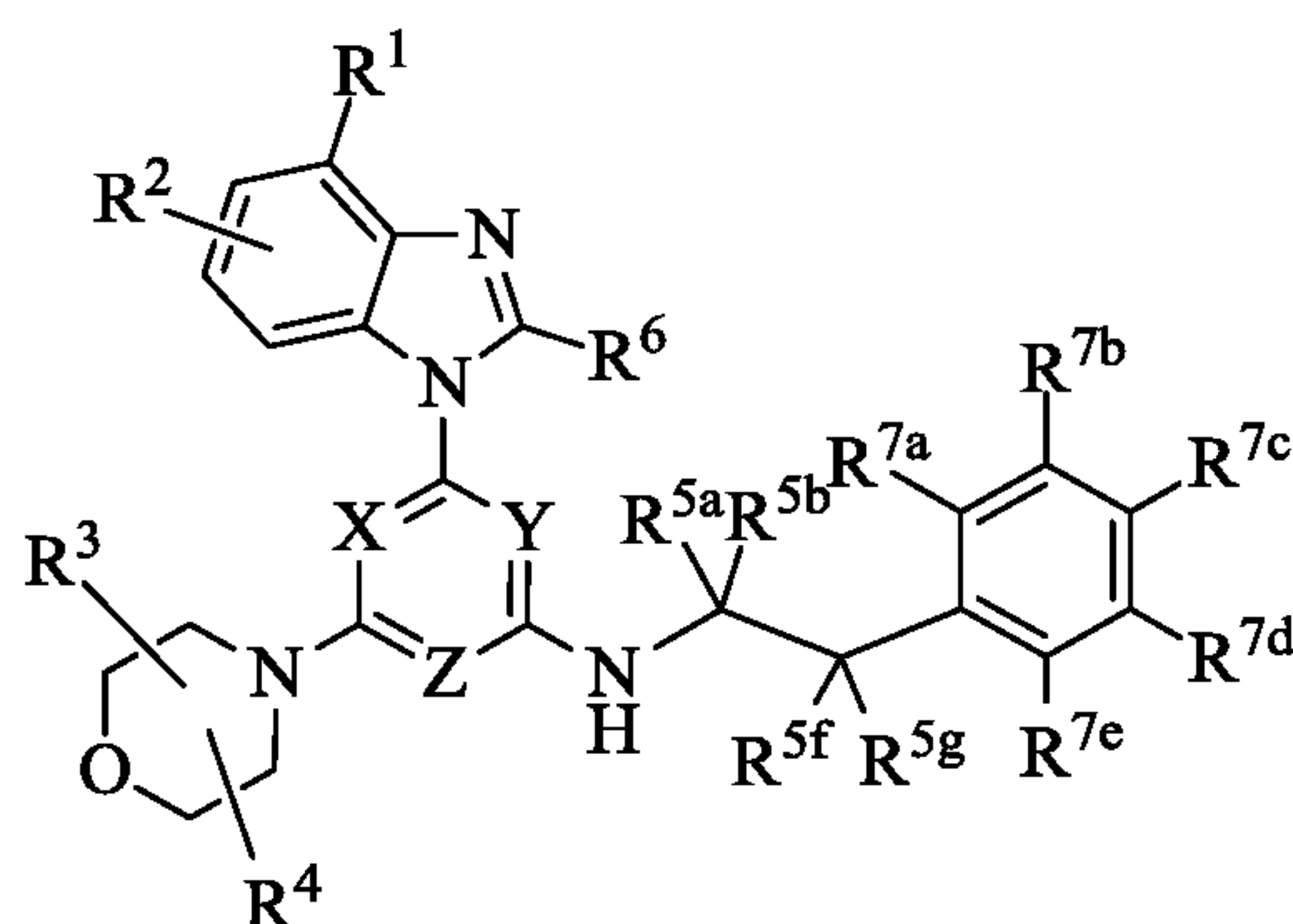
Formula (XI)
