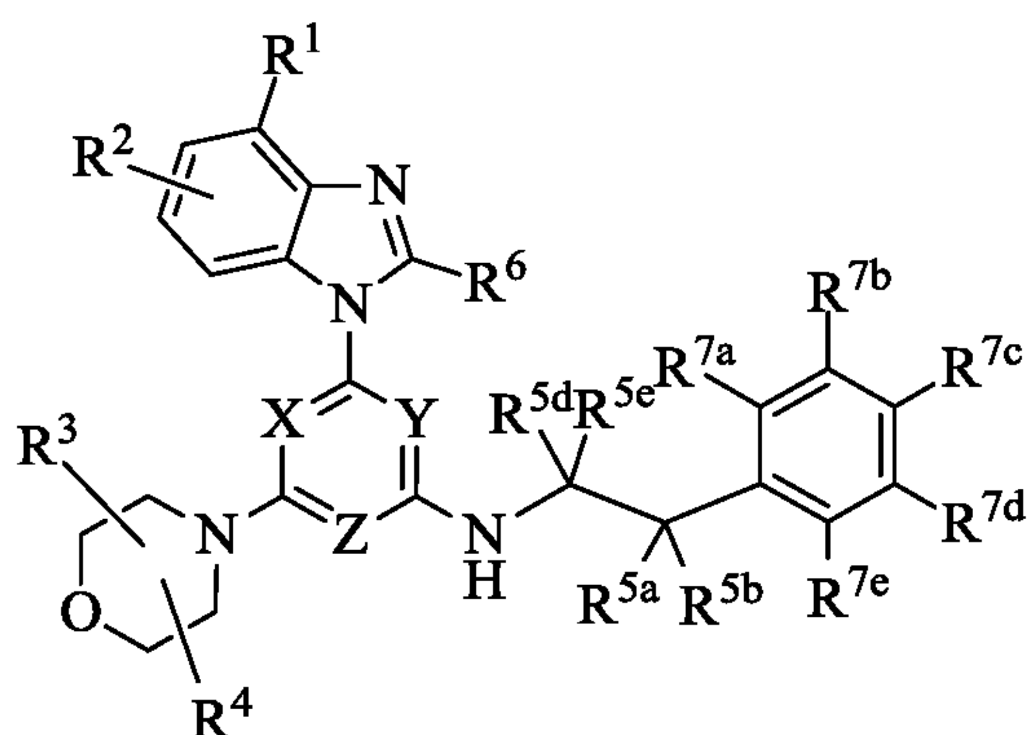
Formula (IX),
