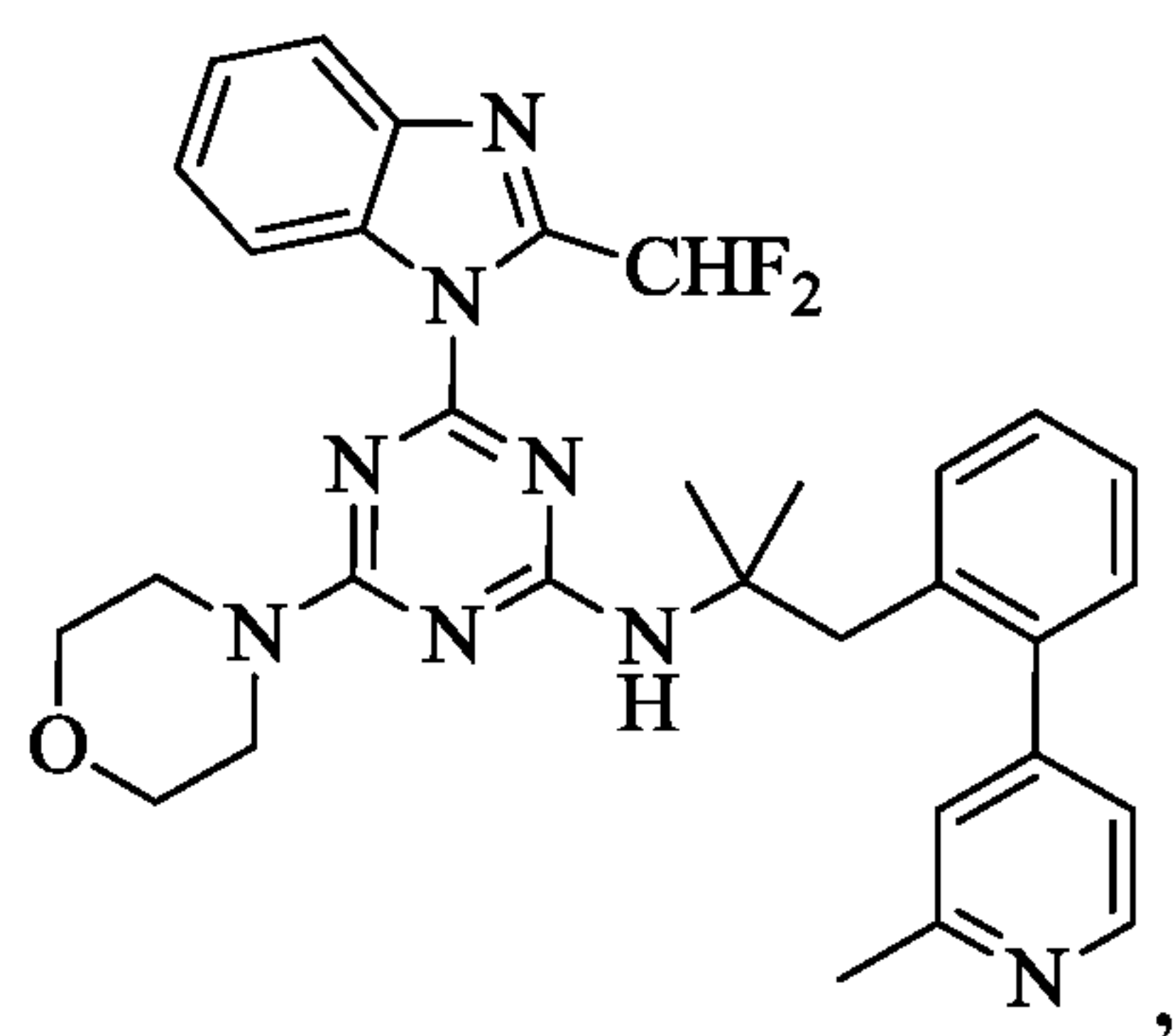
Compound IX
