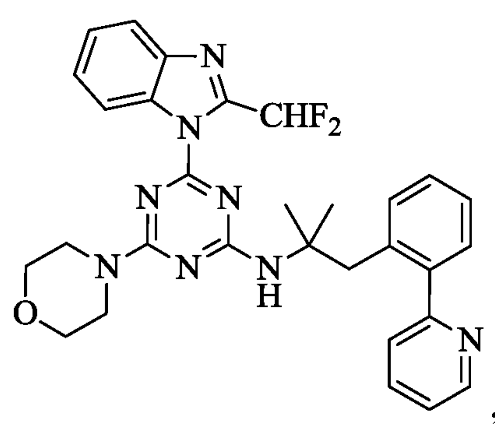
Compound VIII
