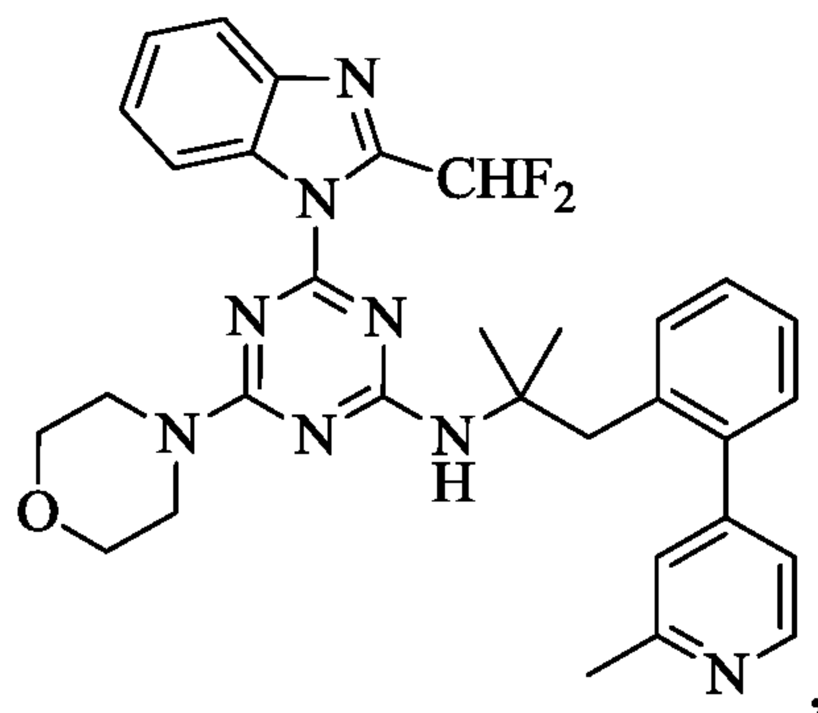
Compound IX
