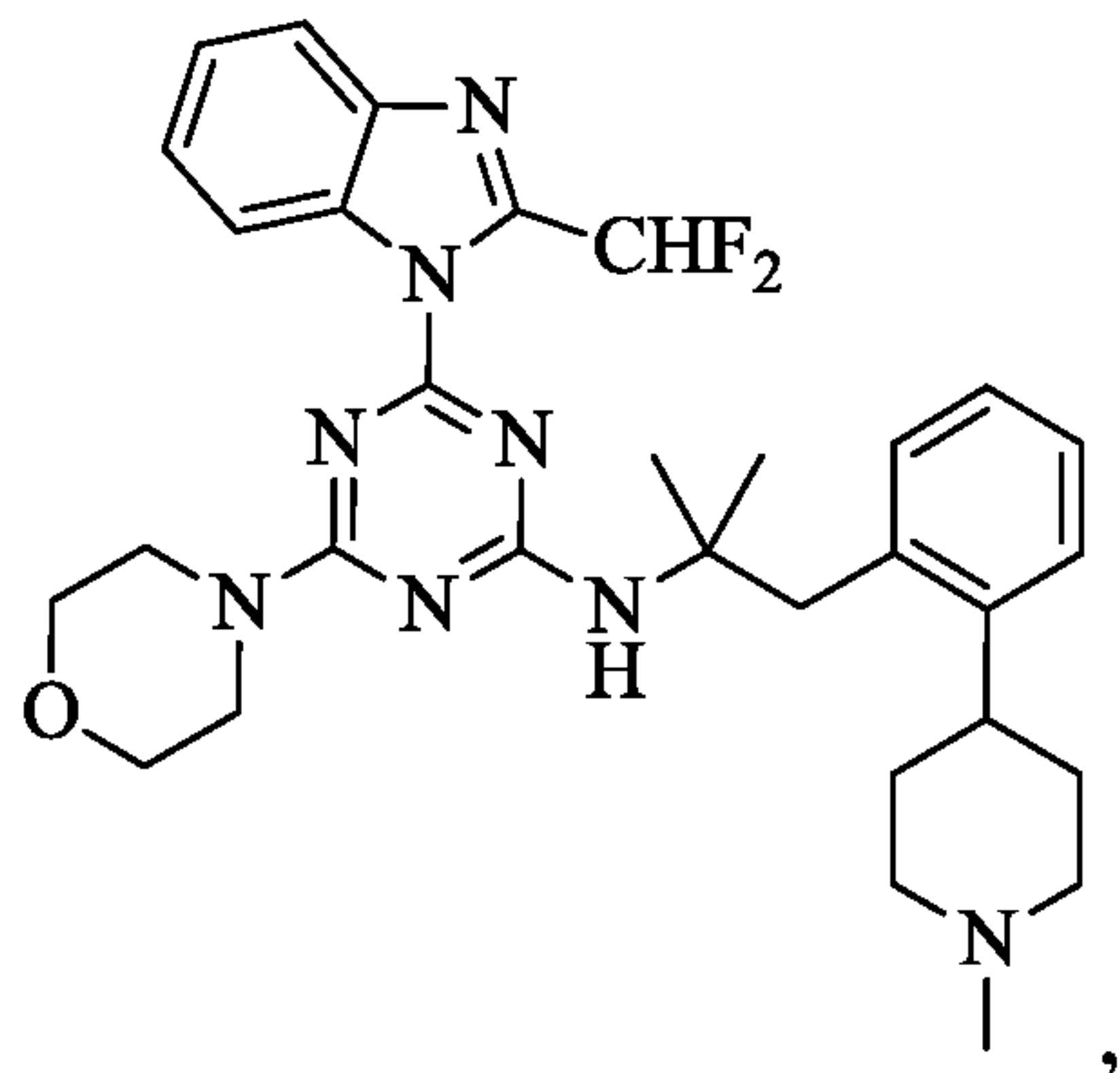
Compound I
