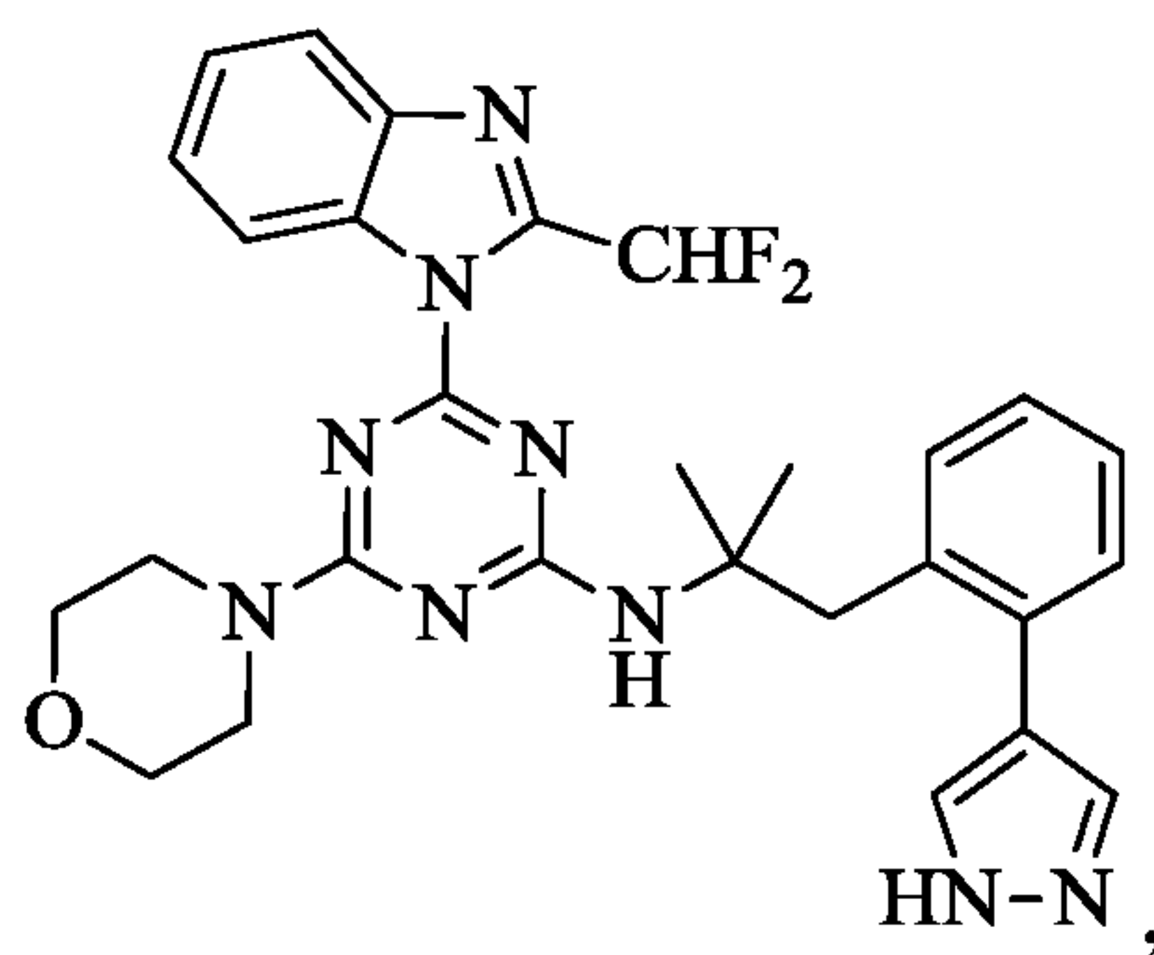
Compound X
