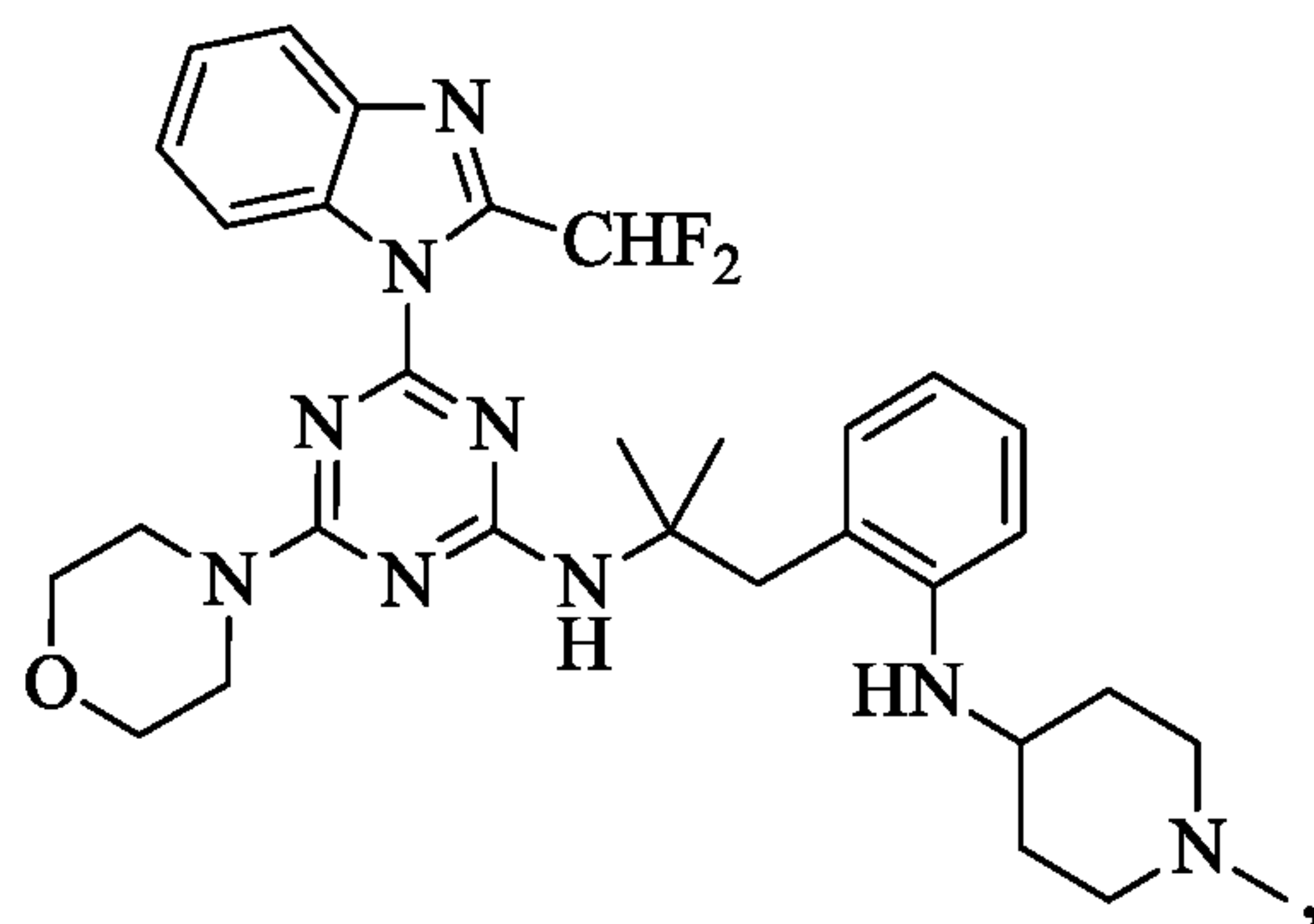
Compound V
