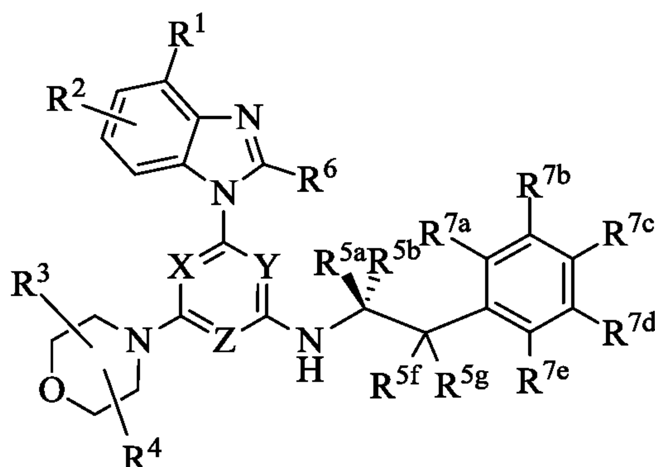
Formula (XIa),
