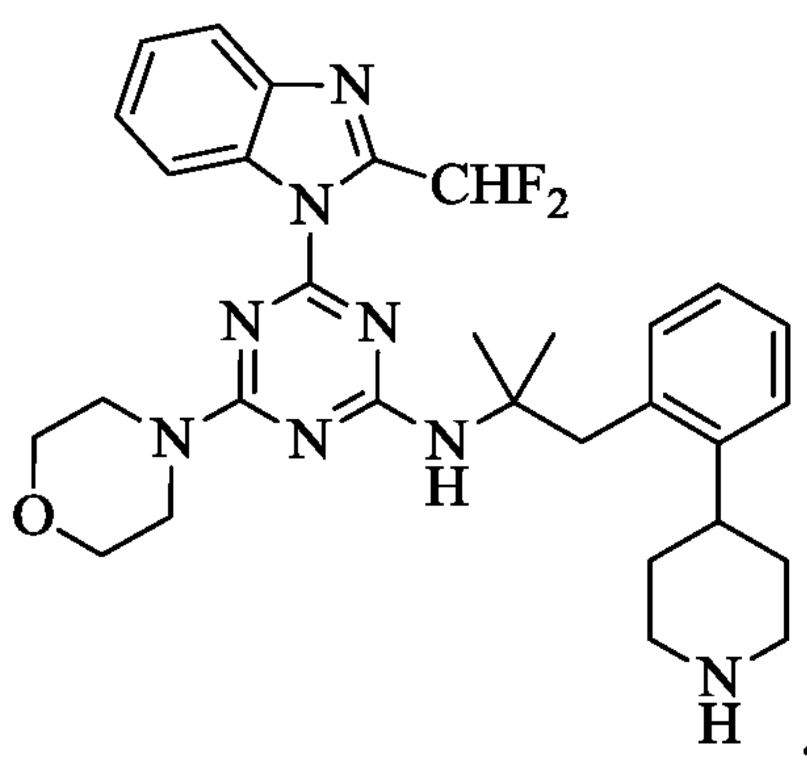
Compound III
