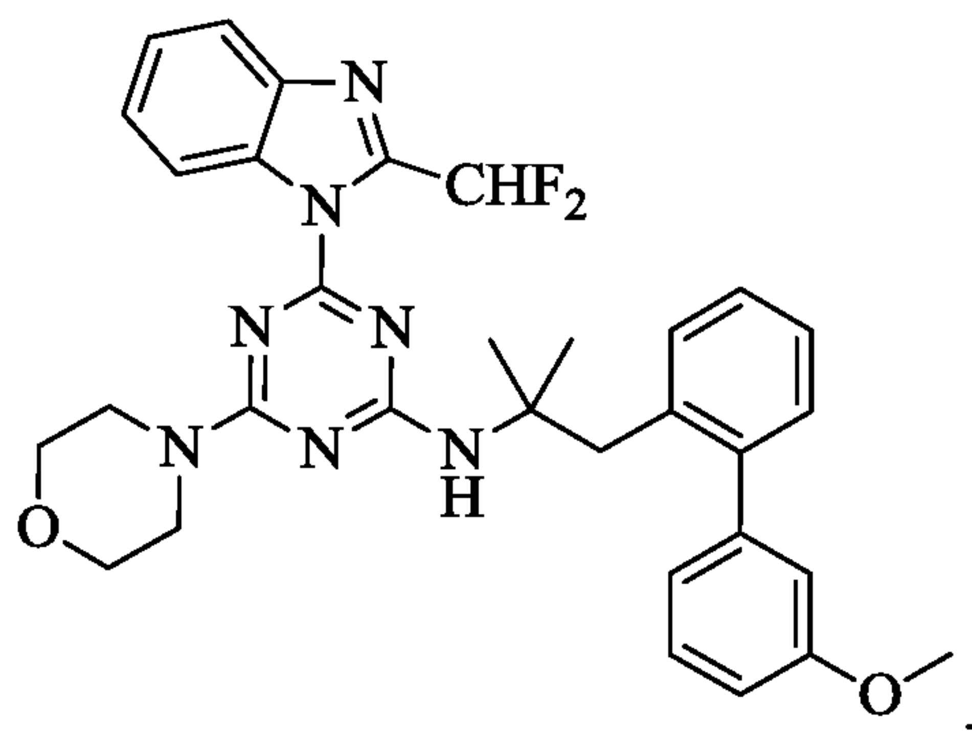
Compound XV
