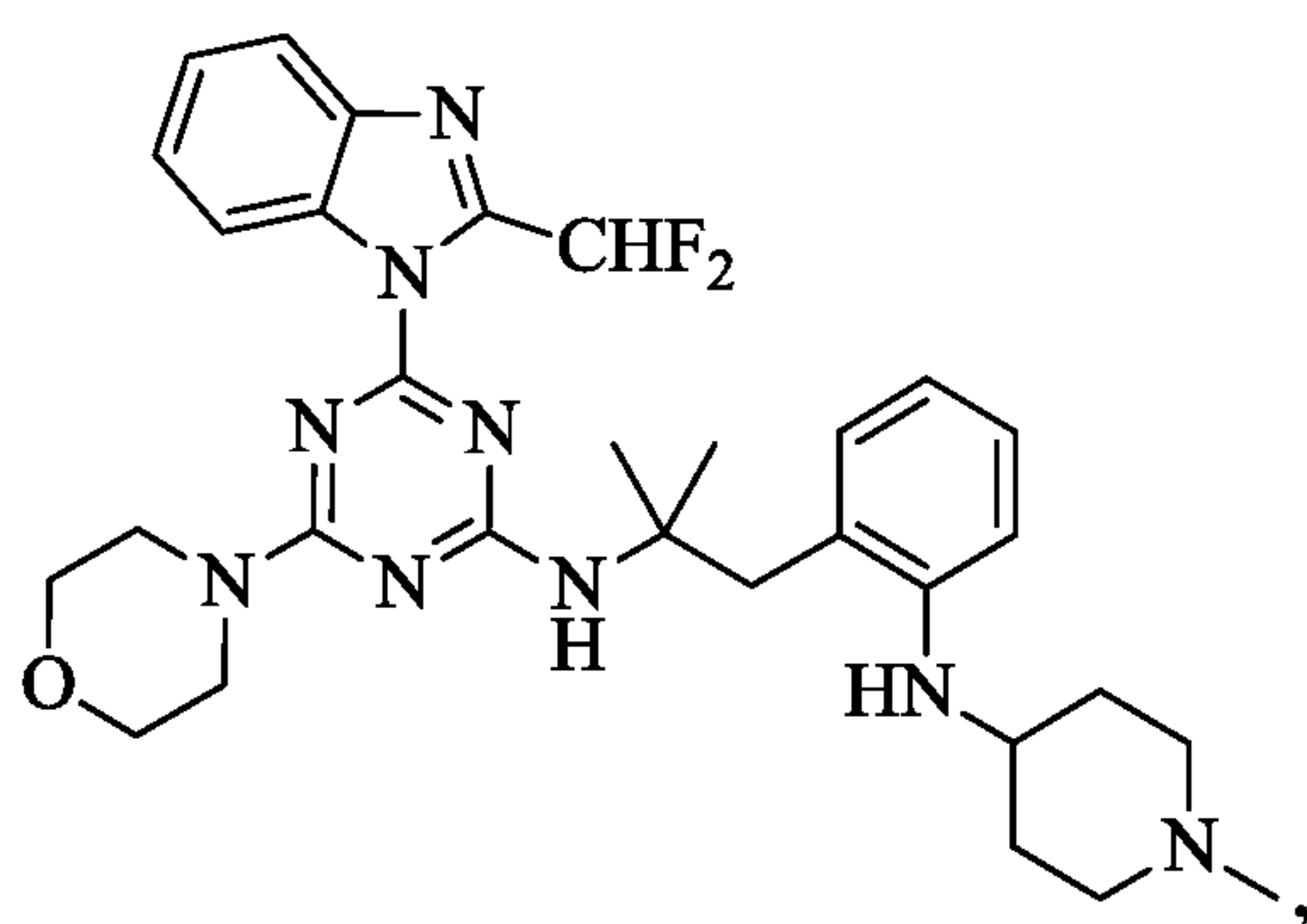
Compound V
