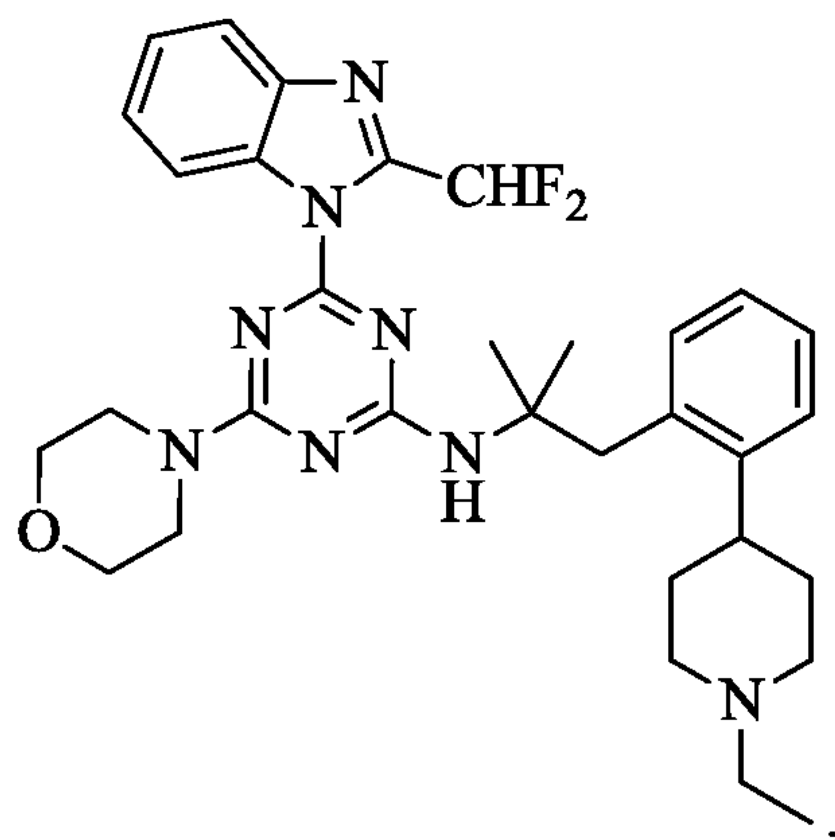
Compound IV
