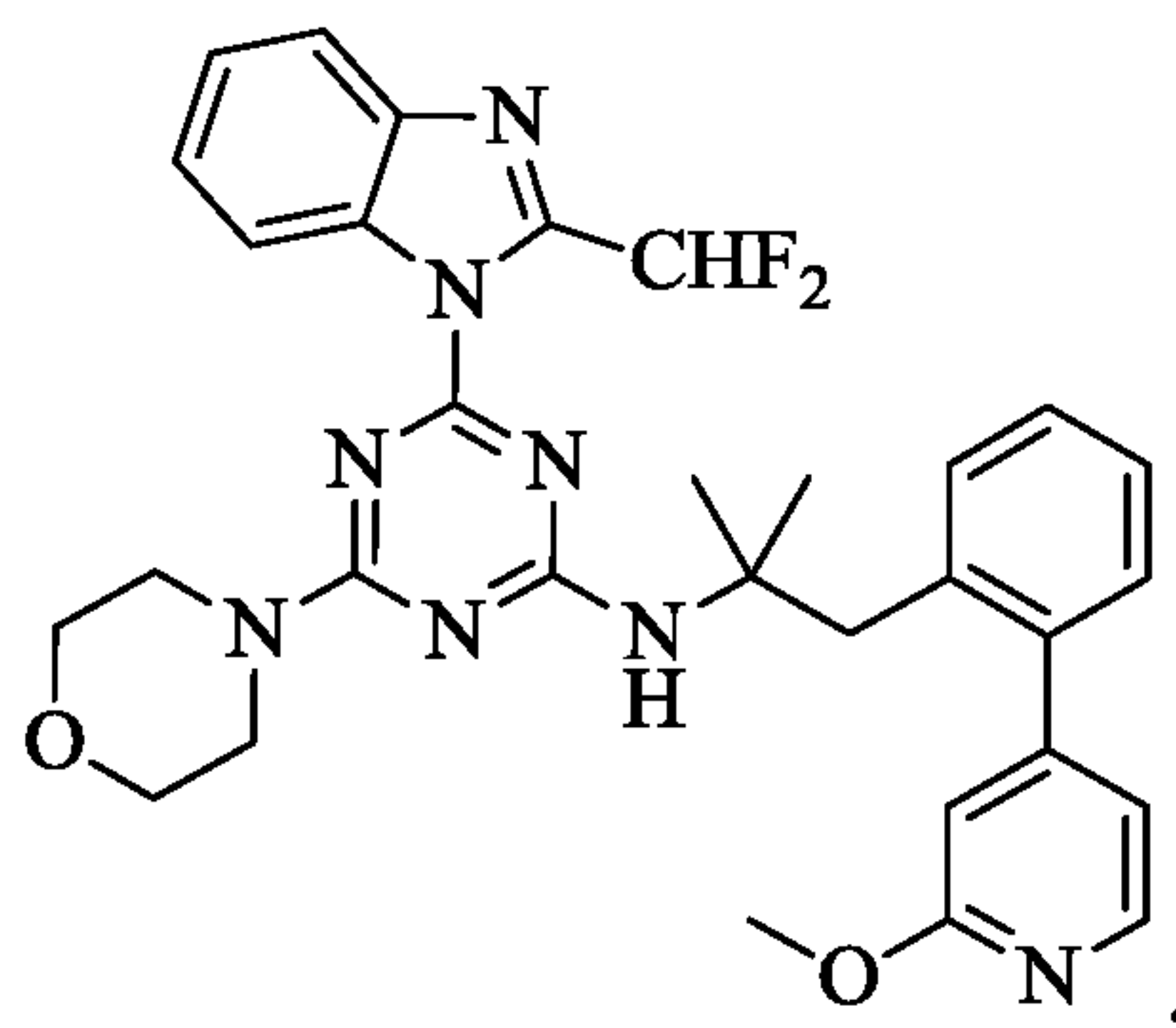
Compound VII
