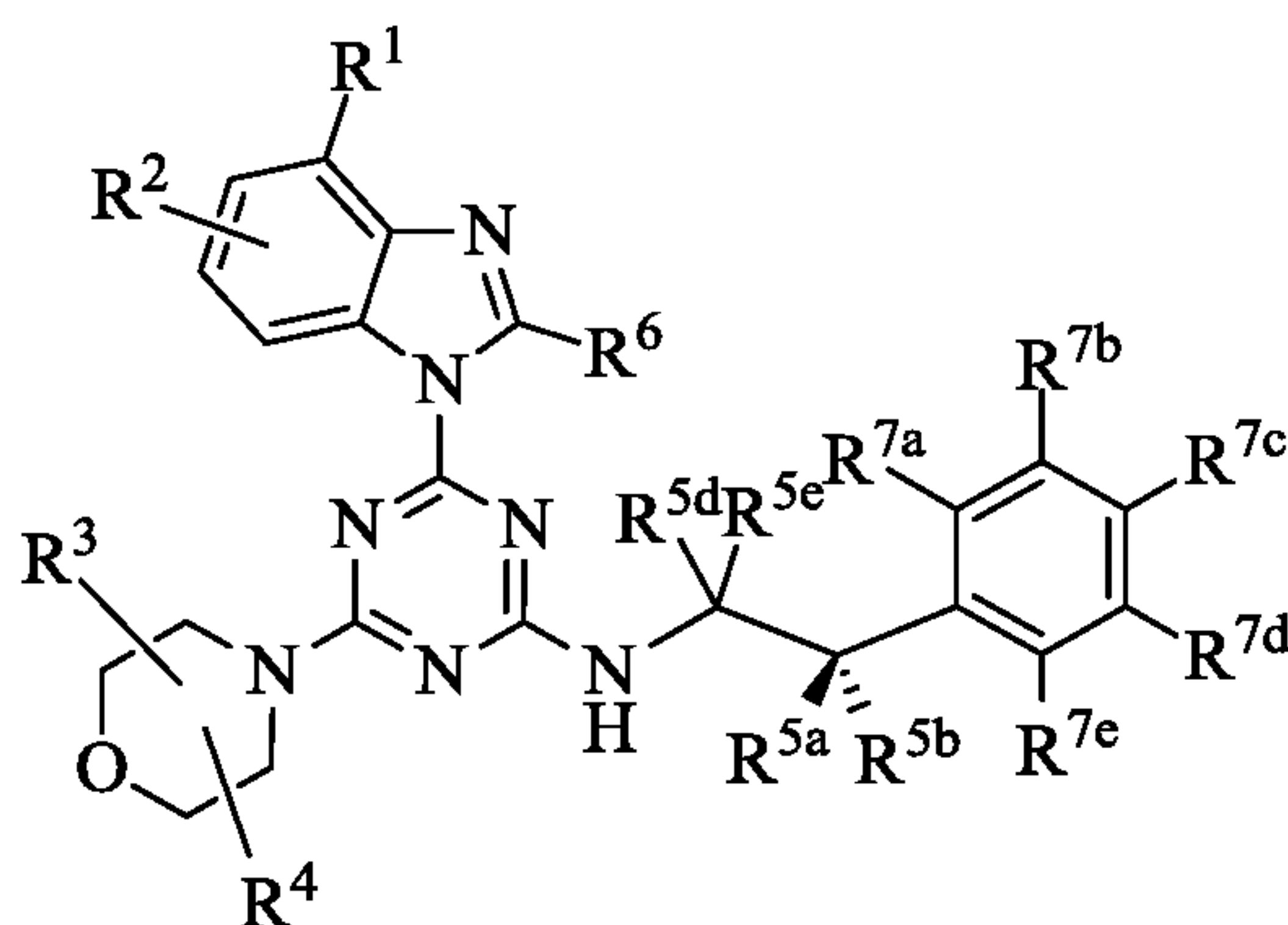
Formula (Xa),
