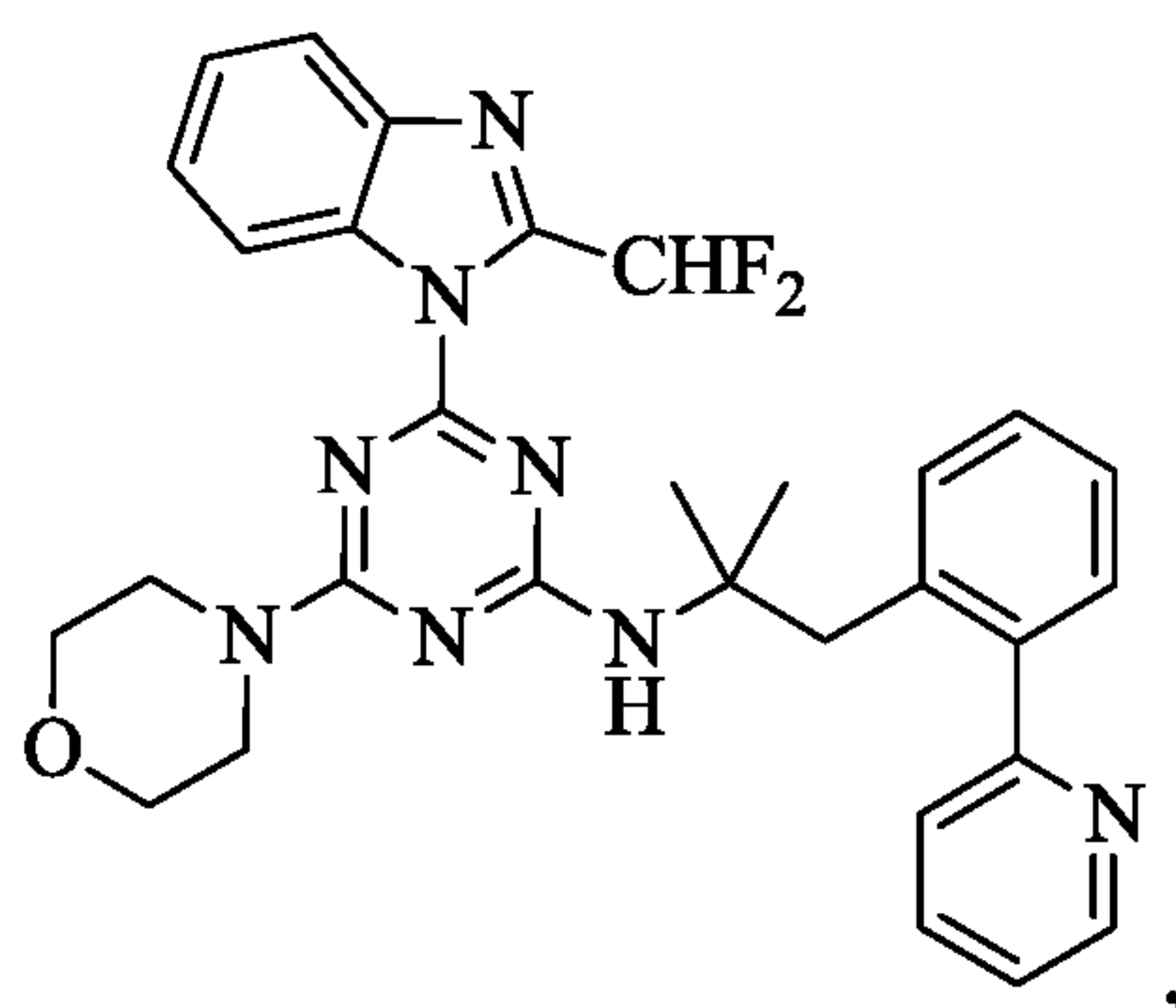
Compound VIII
