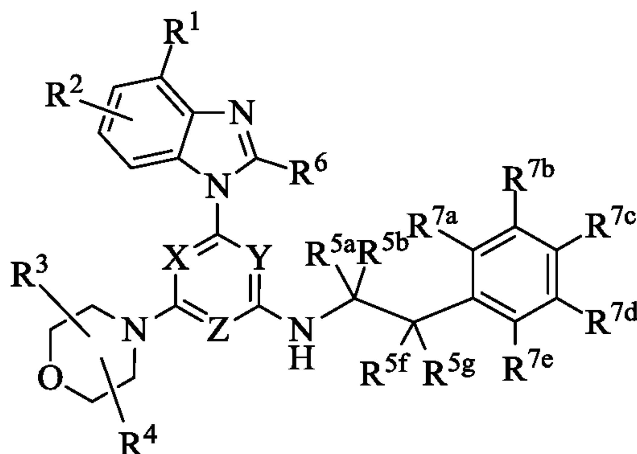
Formula (XI),
