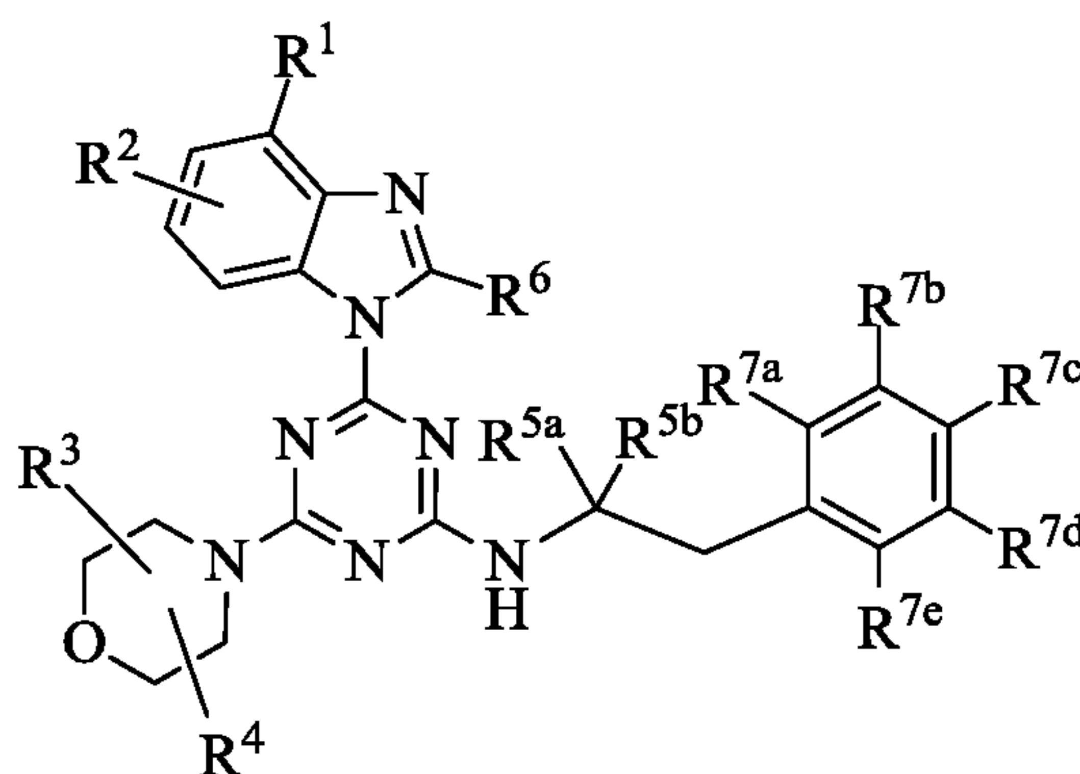
Formula (XVI),
