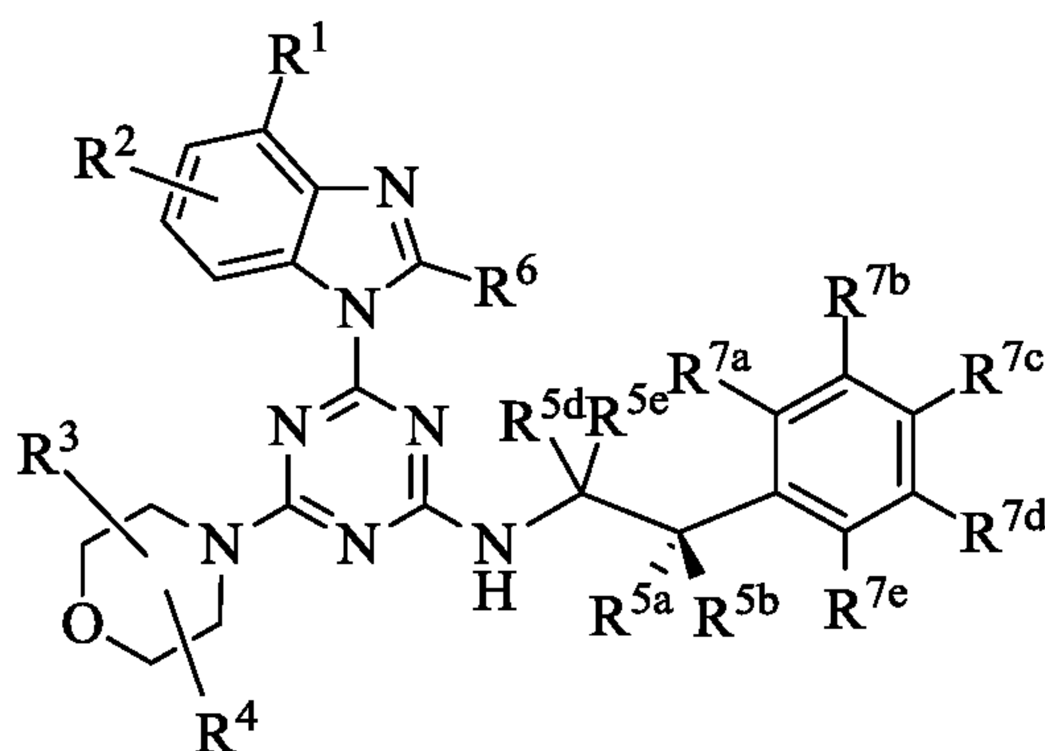
Formula (Xb),
