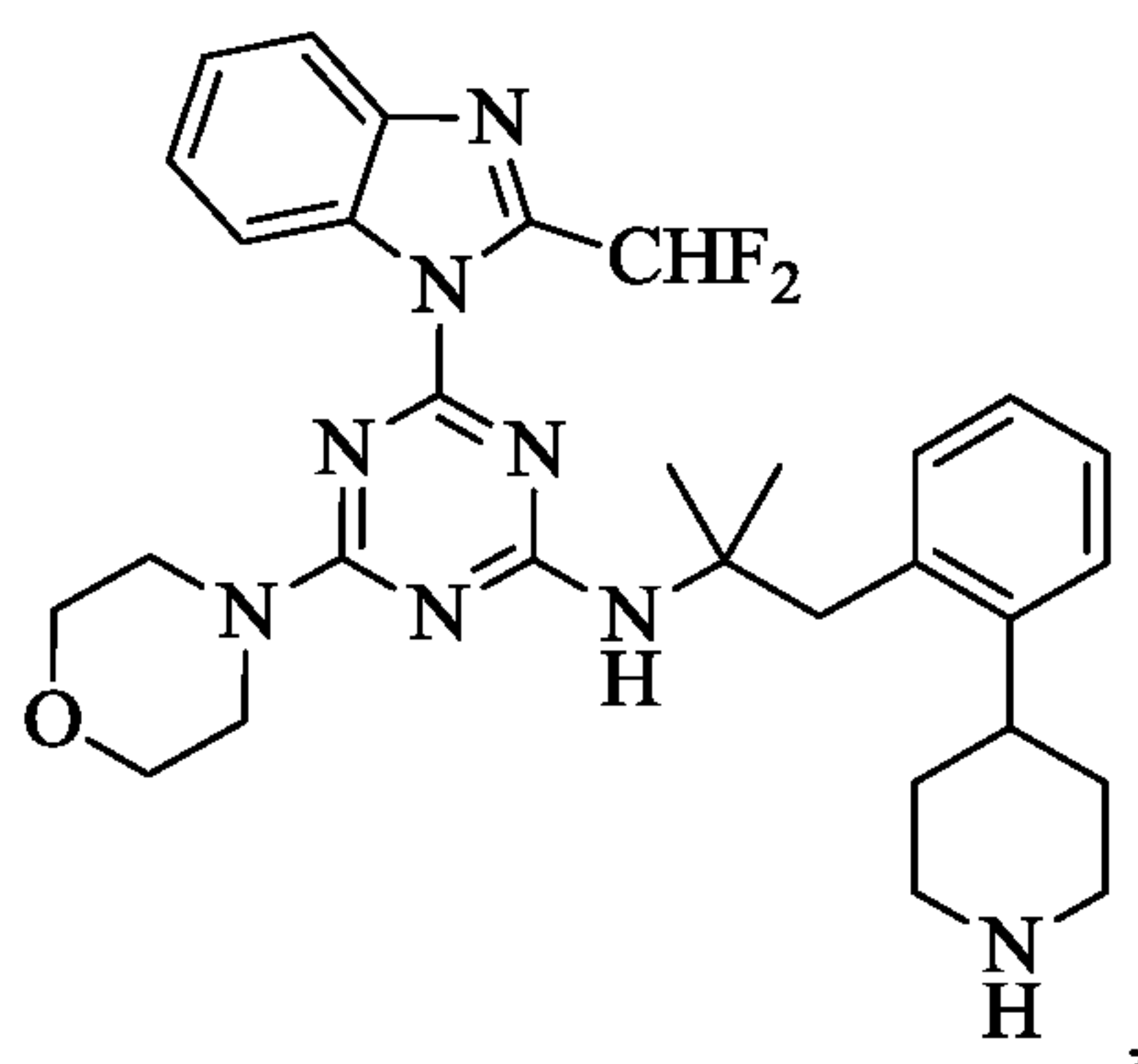
Compound III
