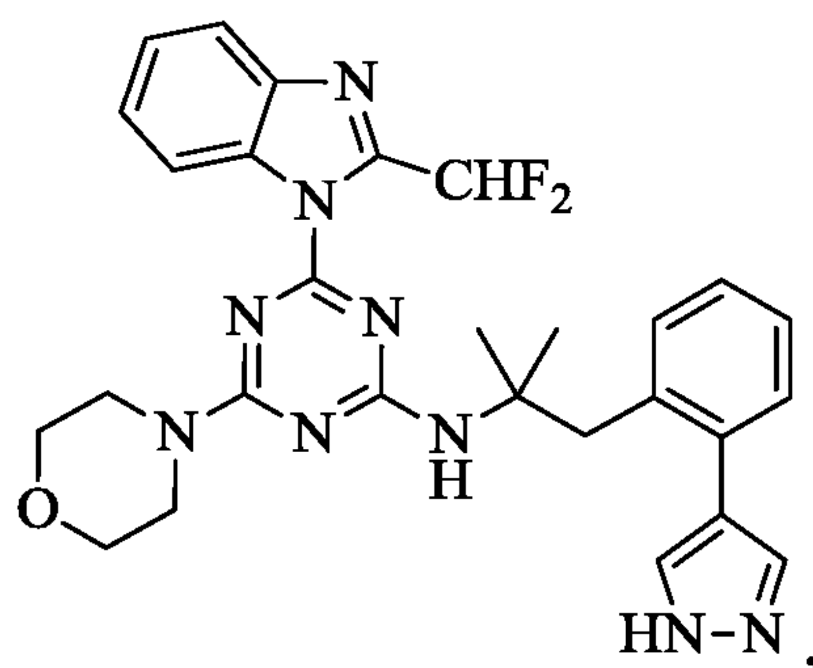
Compound X
