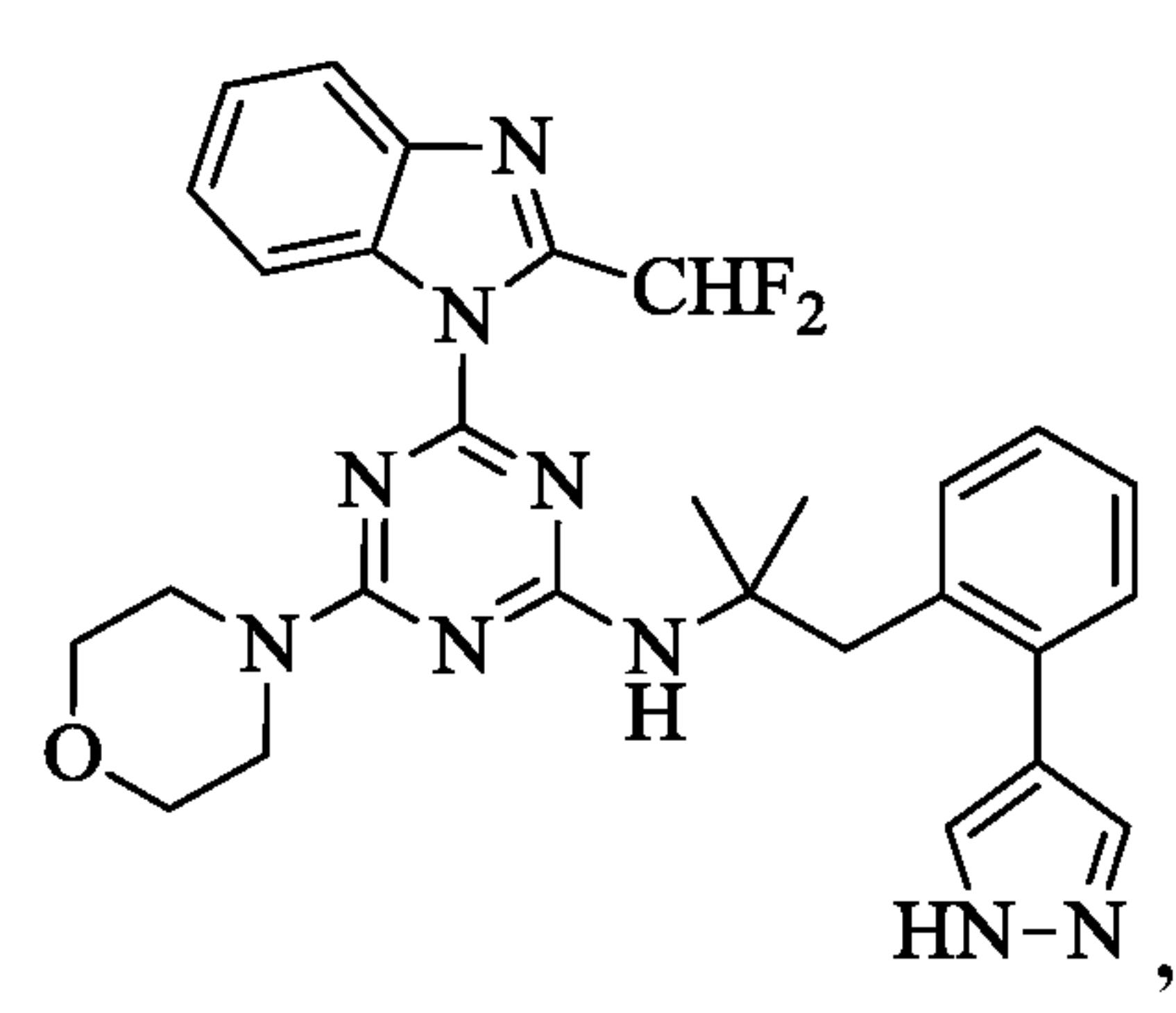
Compound X
