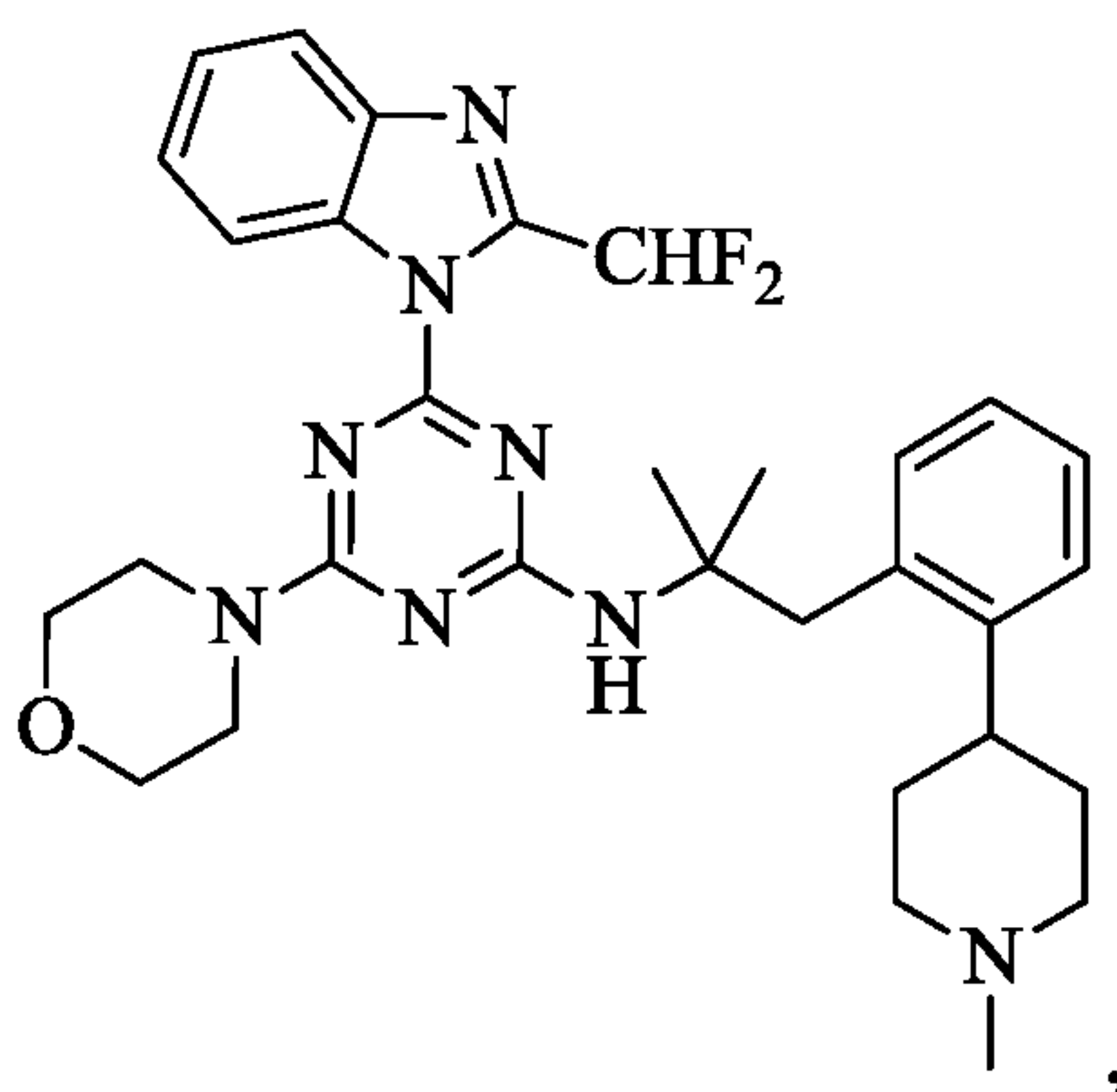
Compound I
