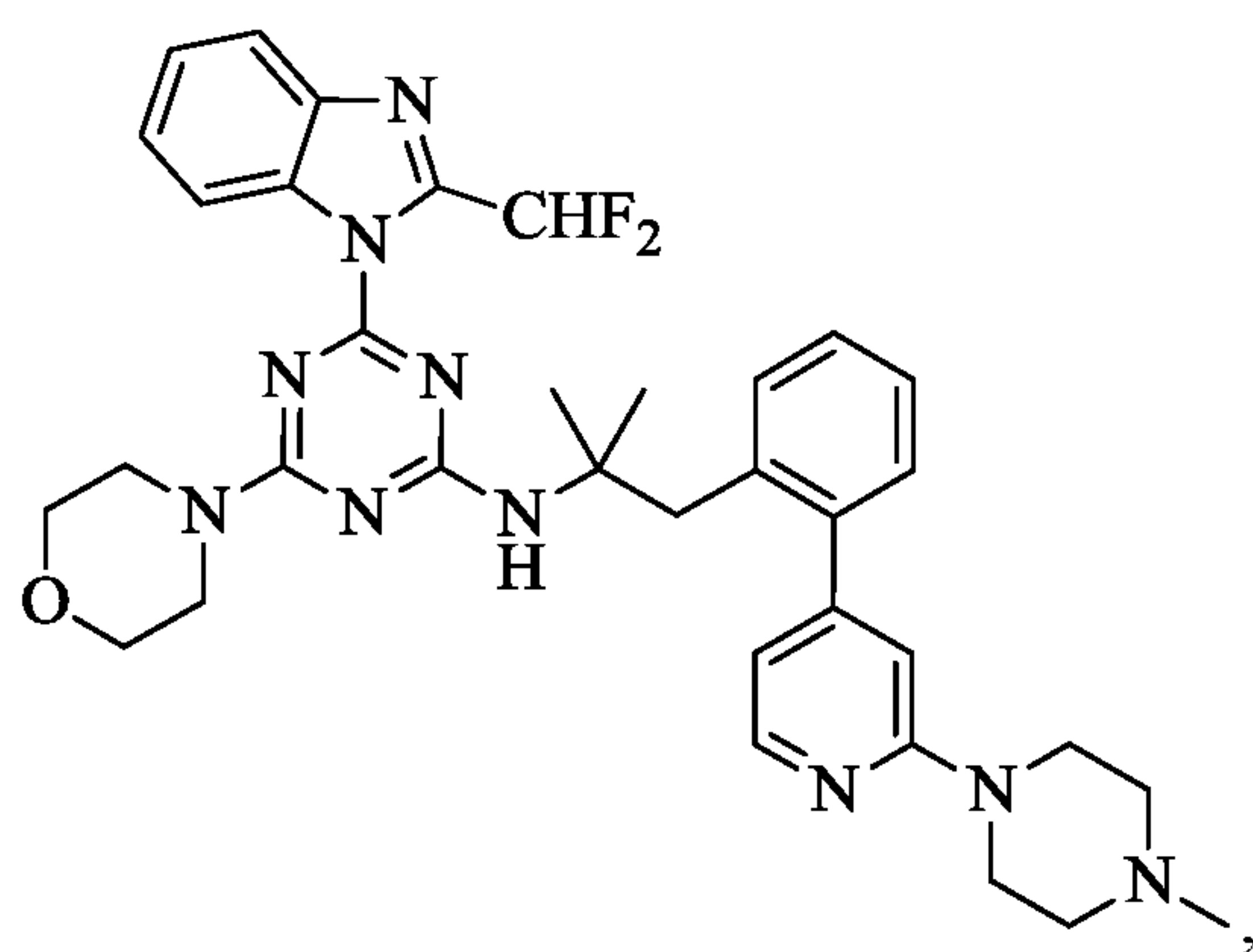
Compound XIII
