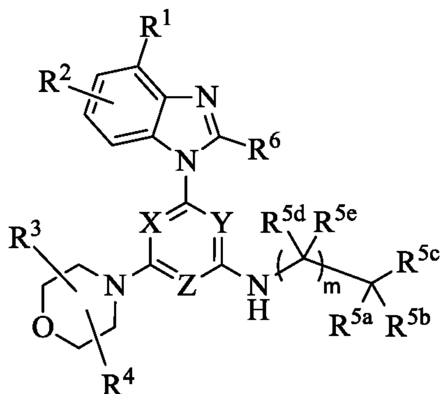
Formula (I),
