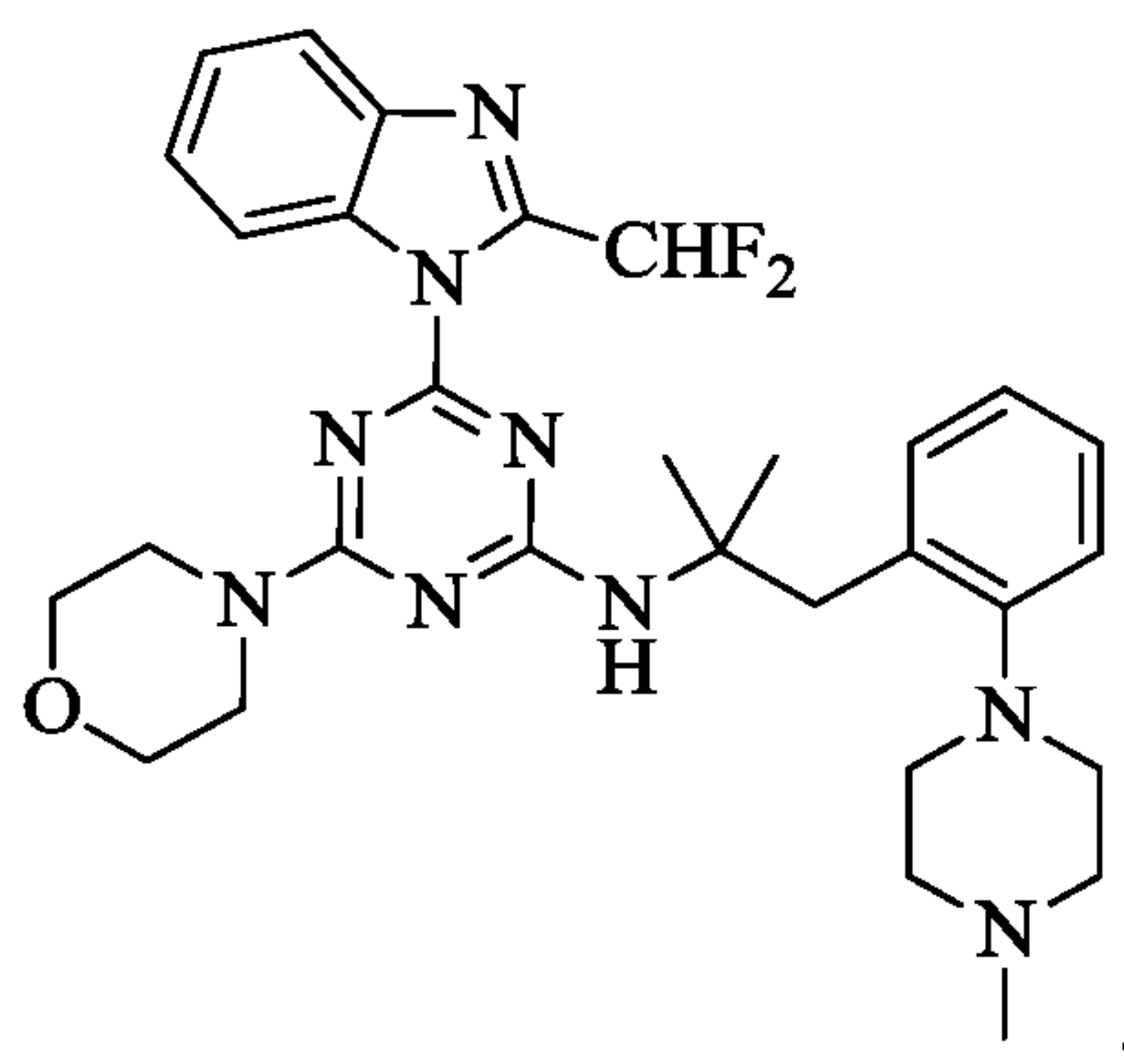
Compound II
