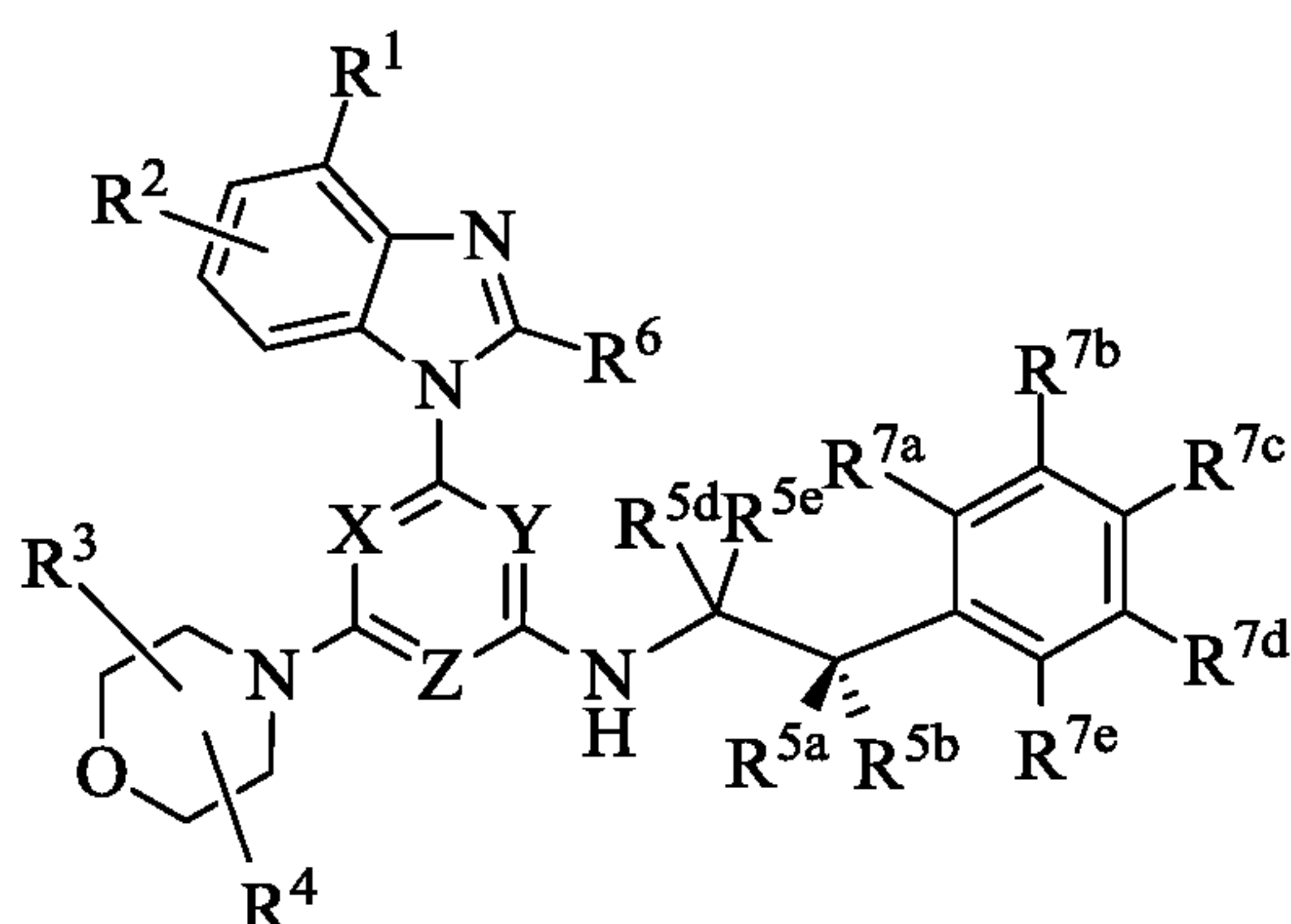
Formula (IXa),
