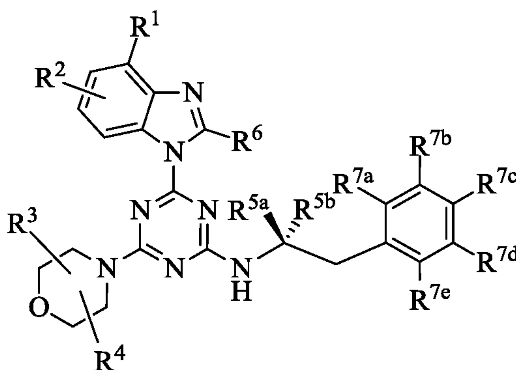
Formula (XVIa)
