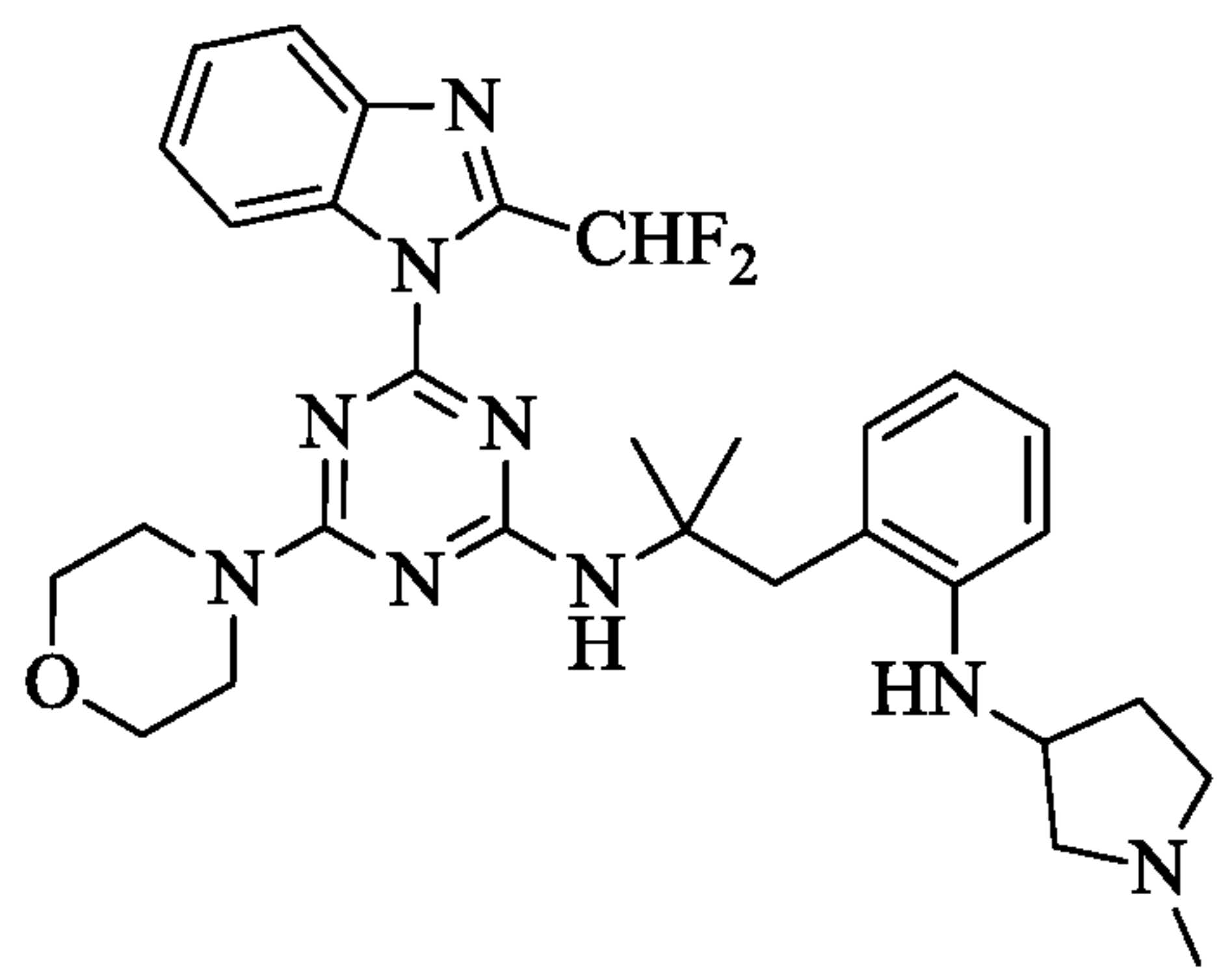
Compound VI
