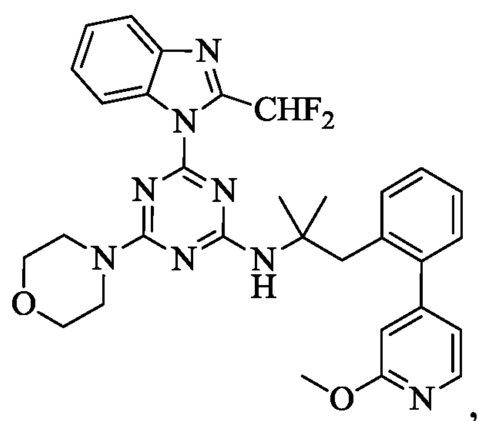
Compound VII
