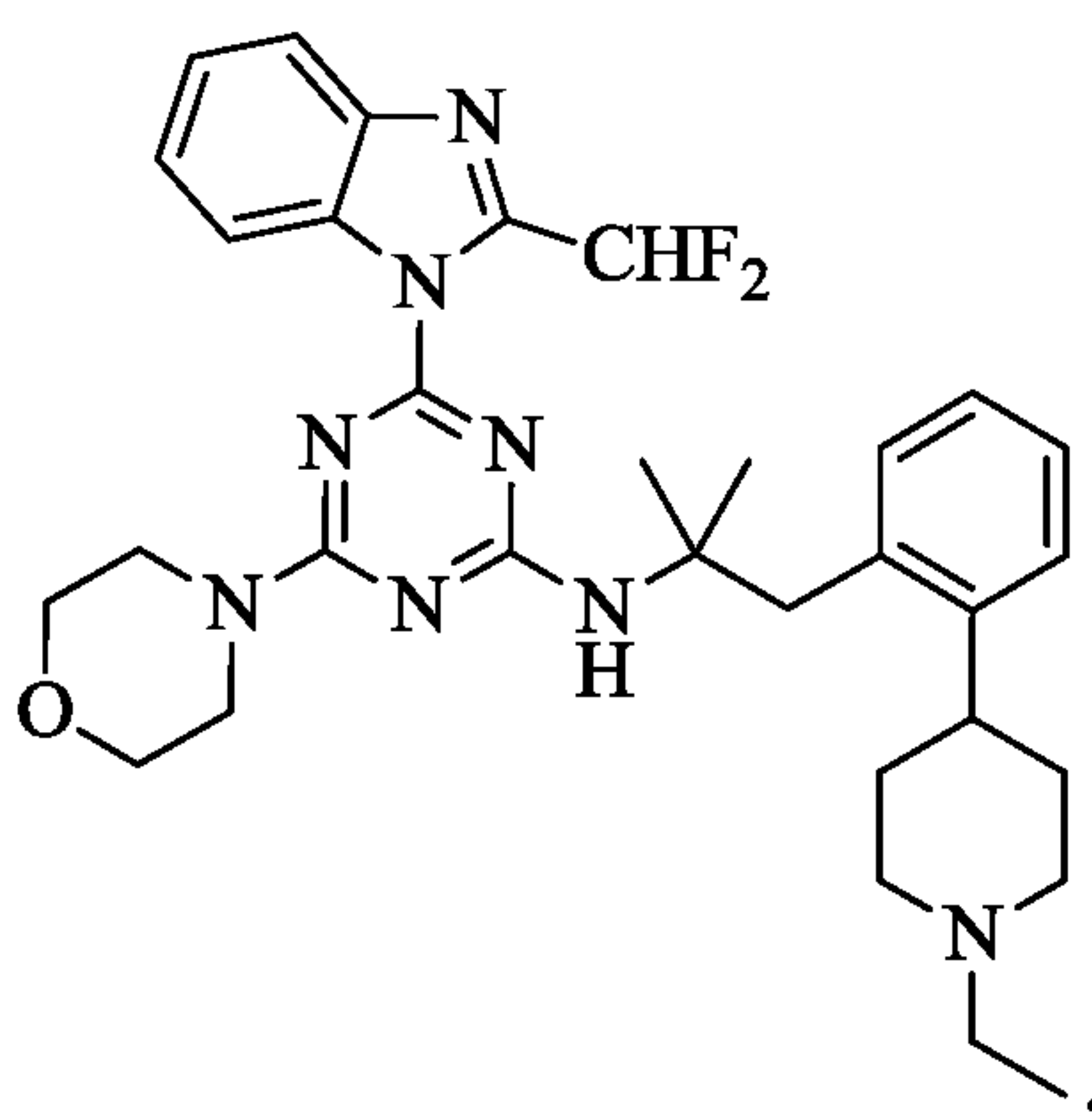
Compound IV
