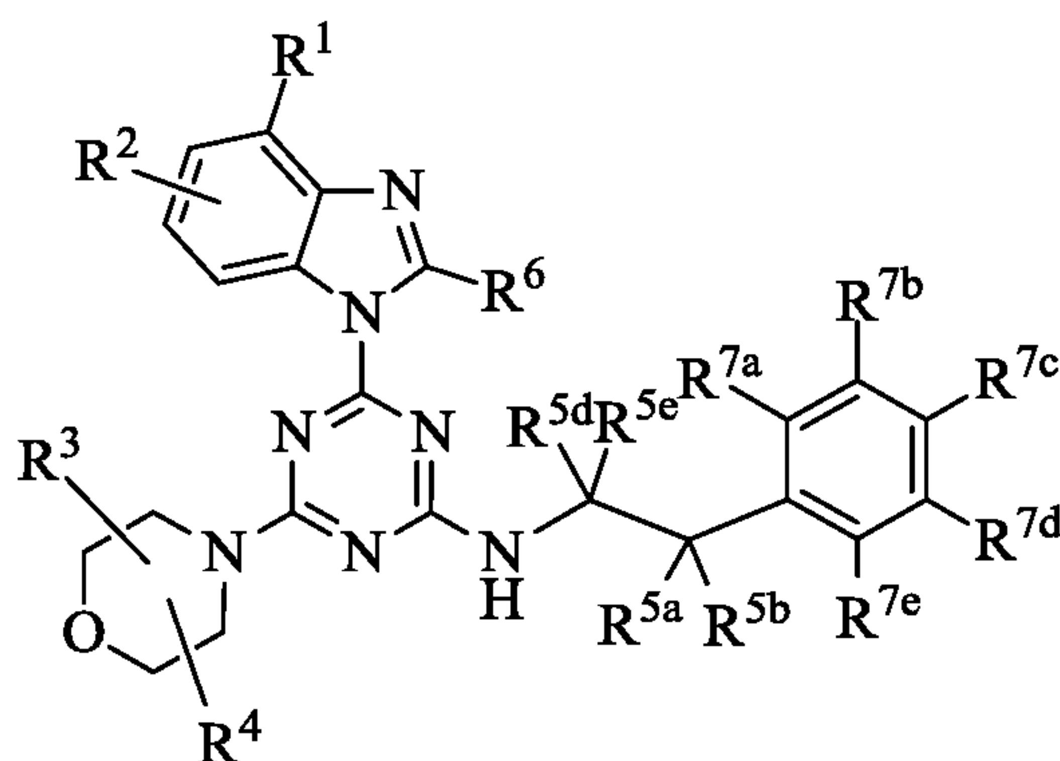
Formula (X),
