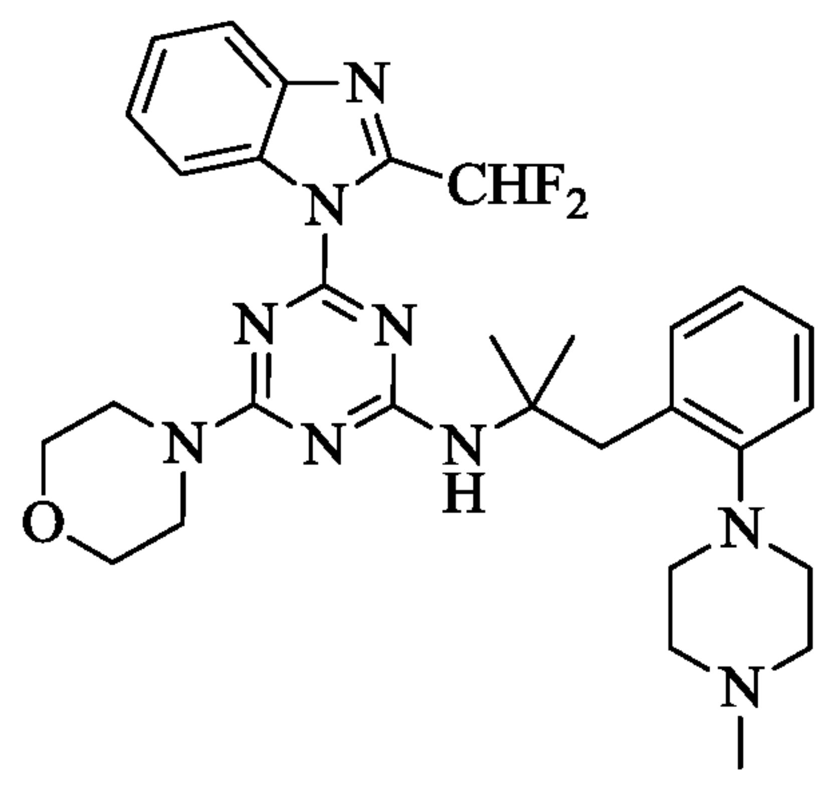
Compound II
