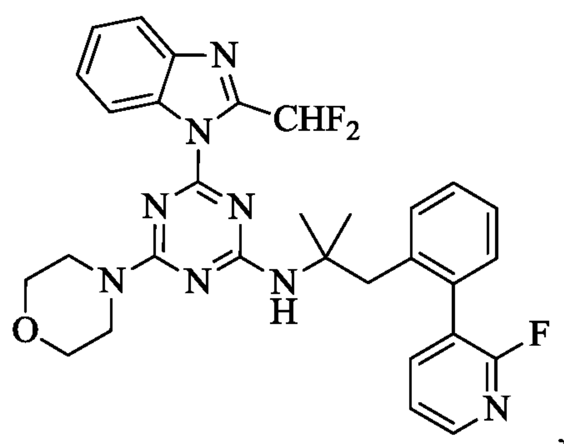
Compound XI
