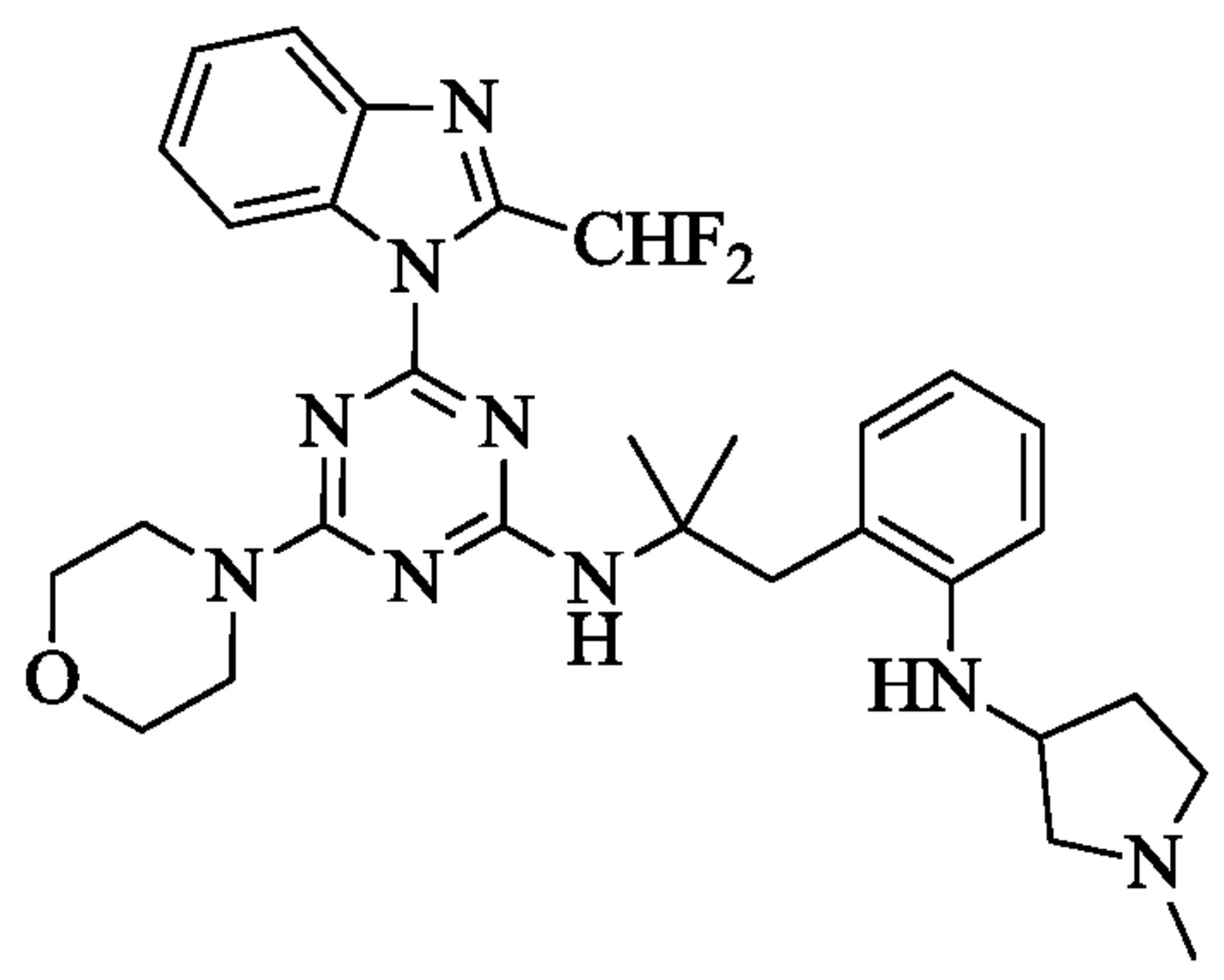
Compound VI
