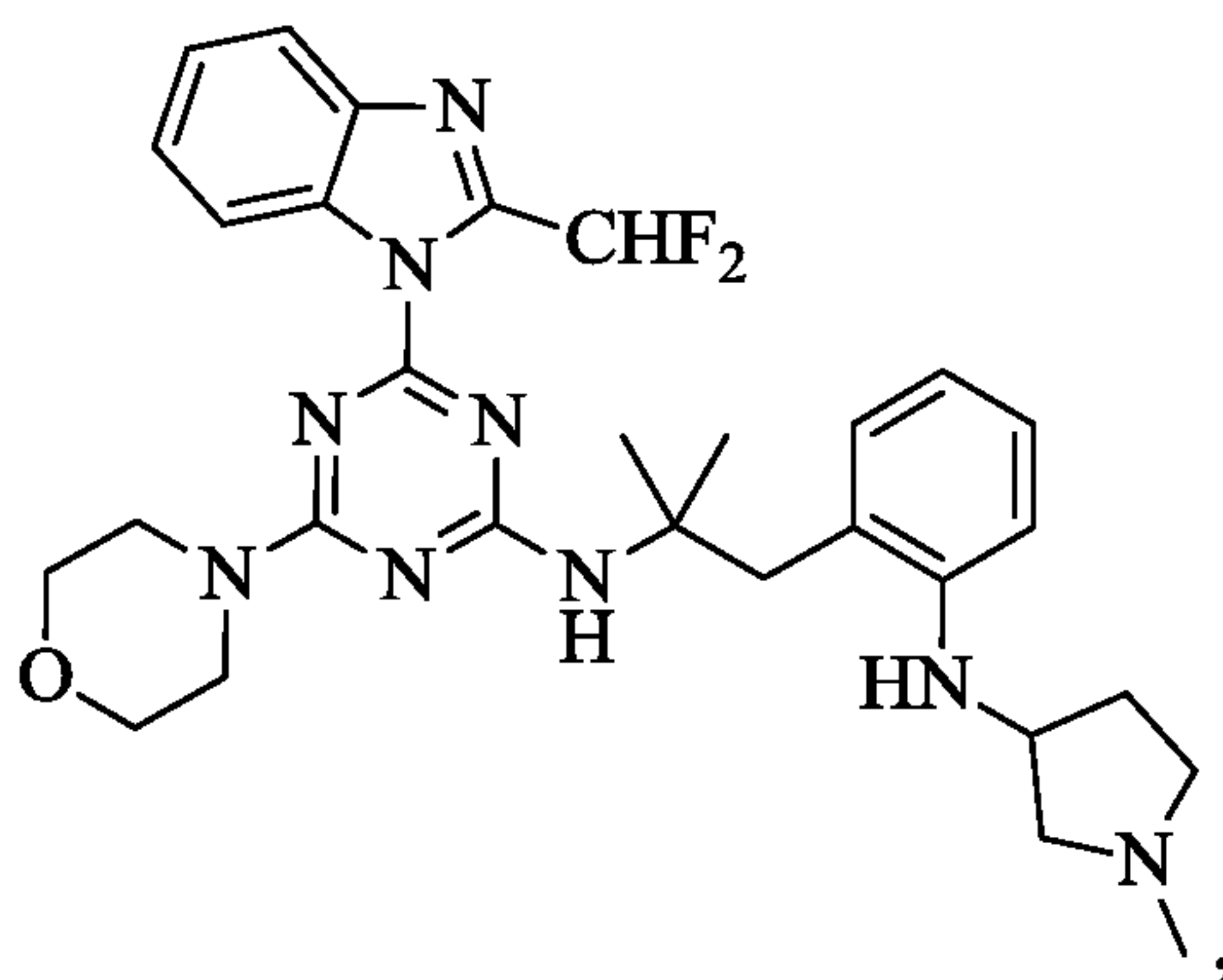
Compound VI
