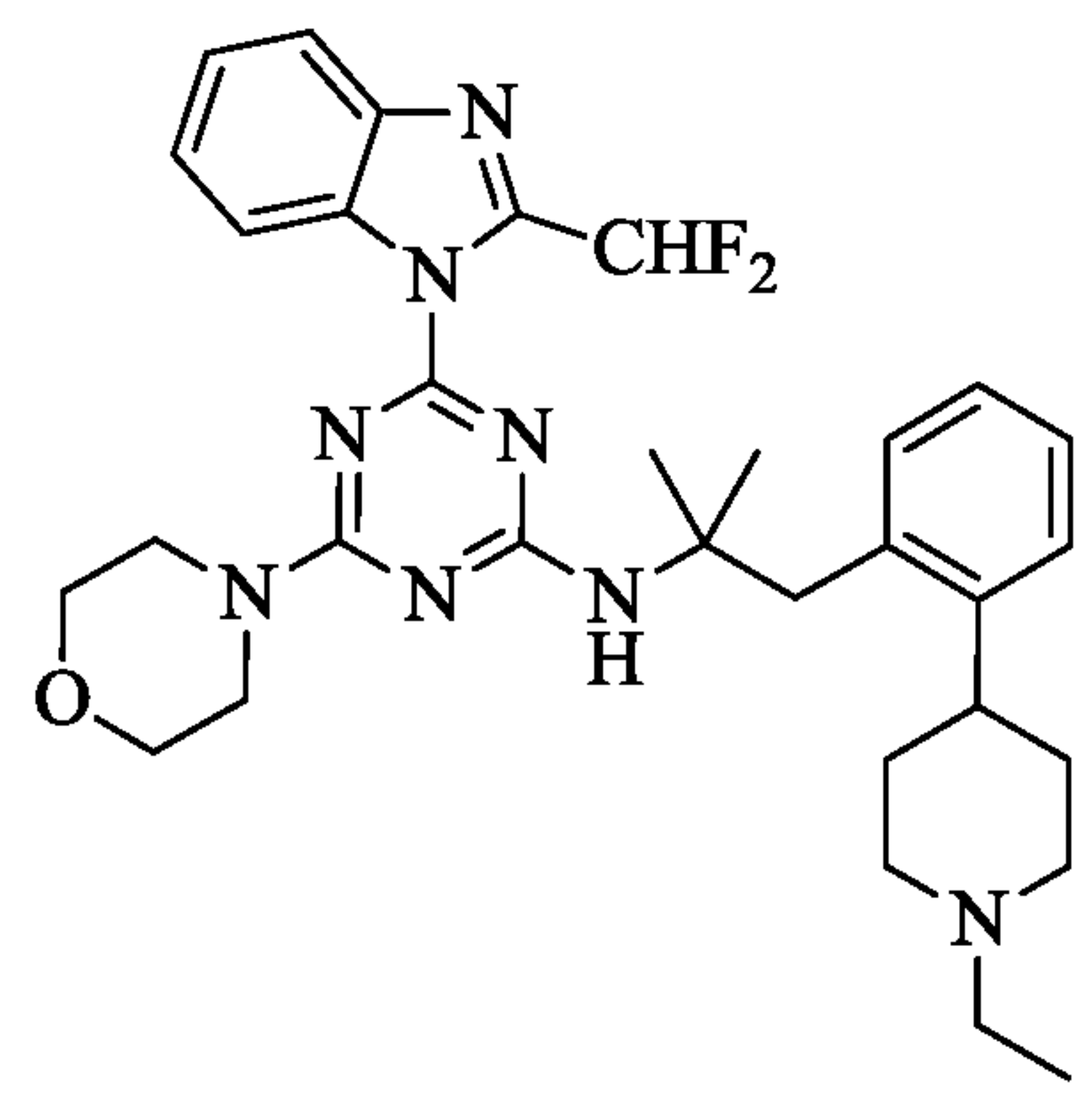
Compound IV
