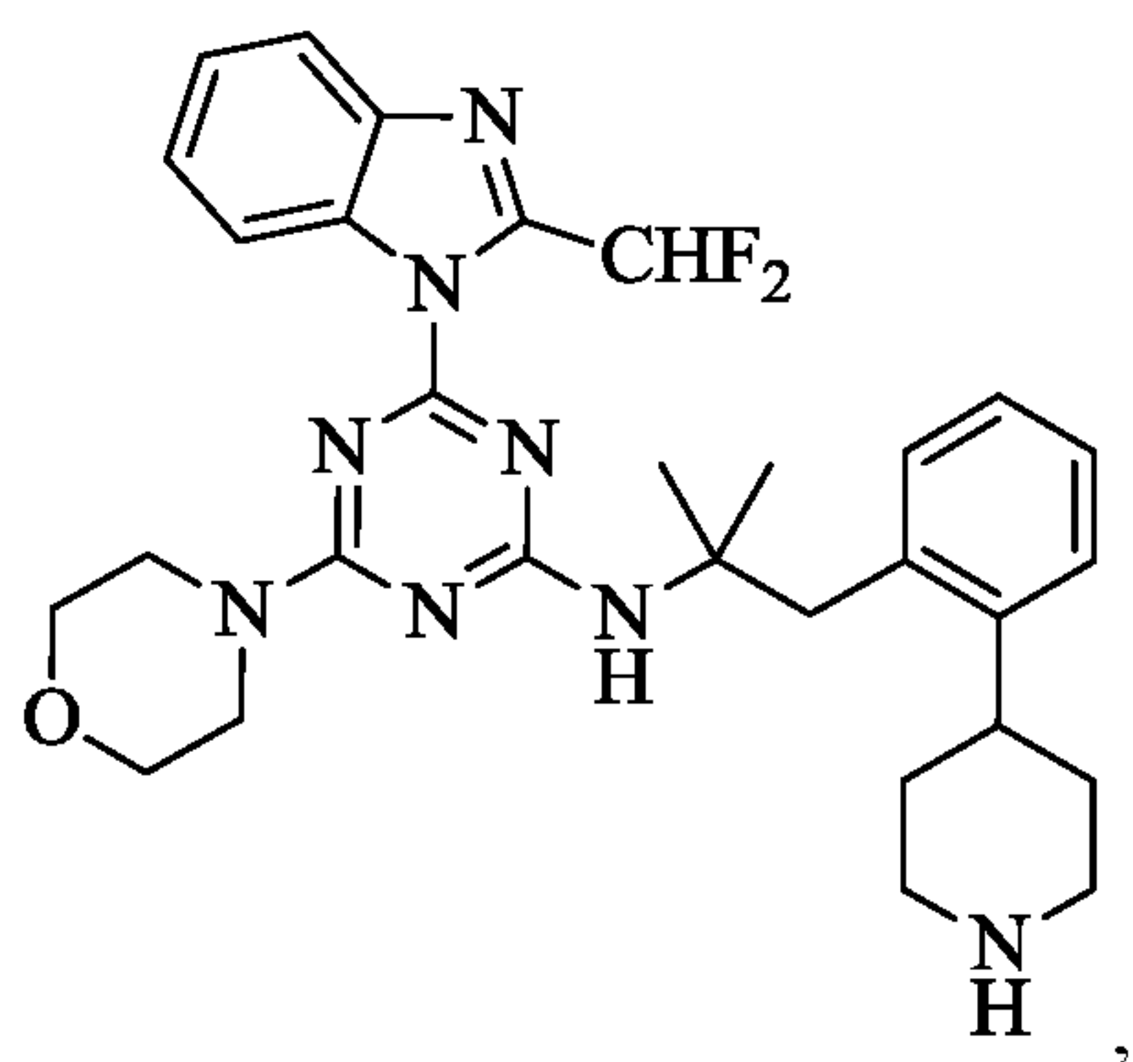
Compound III
