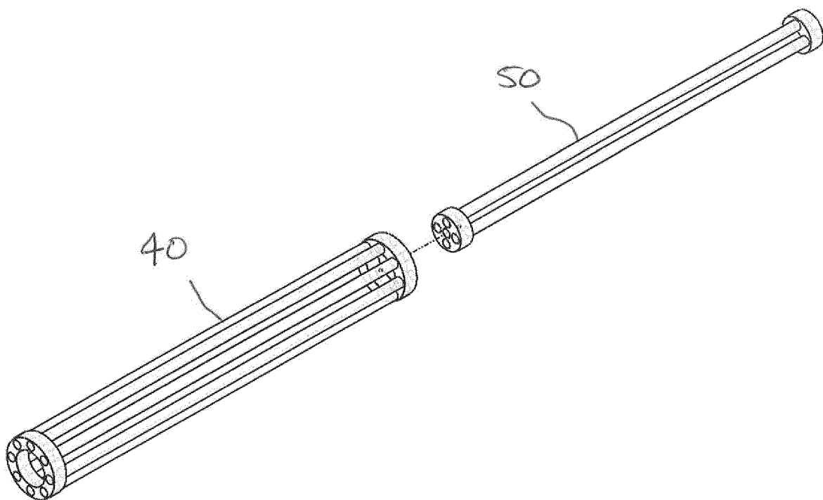
b) Expanded view of the bundle mount
