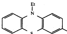
10-Ethylphenothiazine-3-yl group
