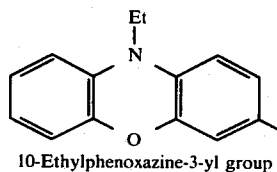
10-Ethylphenoxazine-3-yl group
