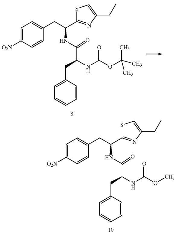
Scheme III
