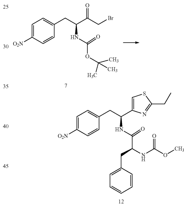
Scheme IV
