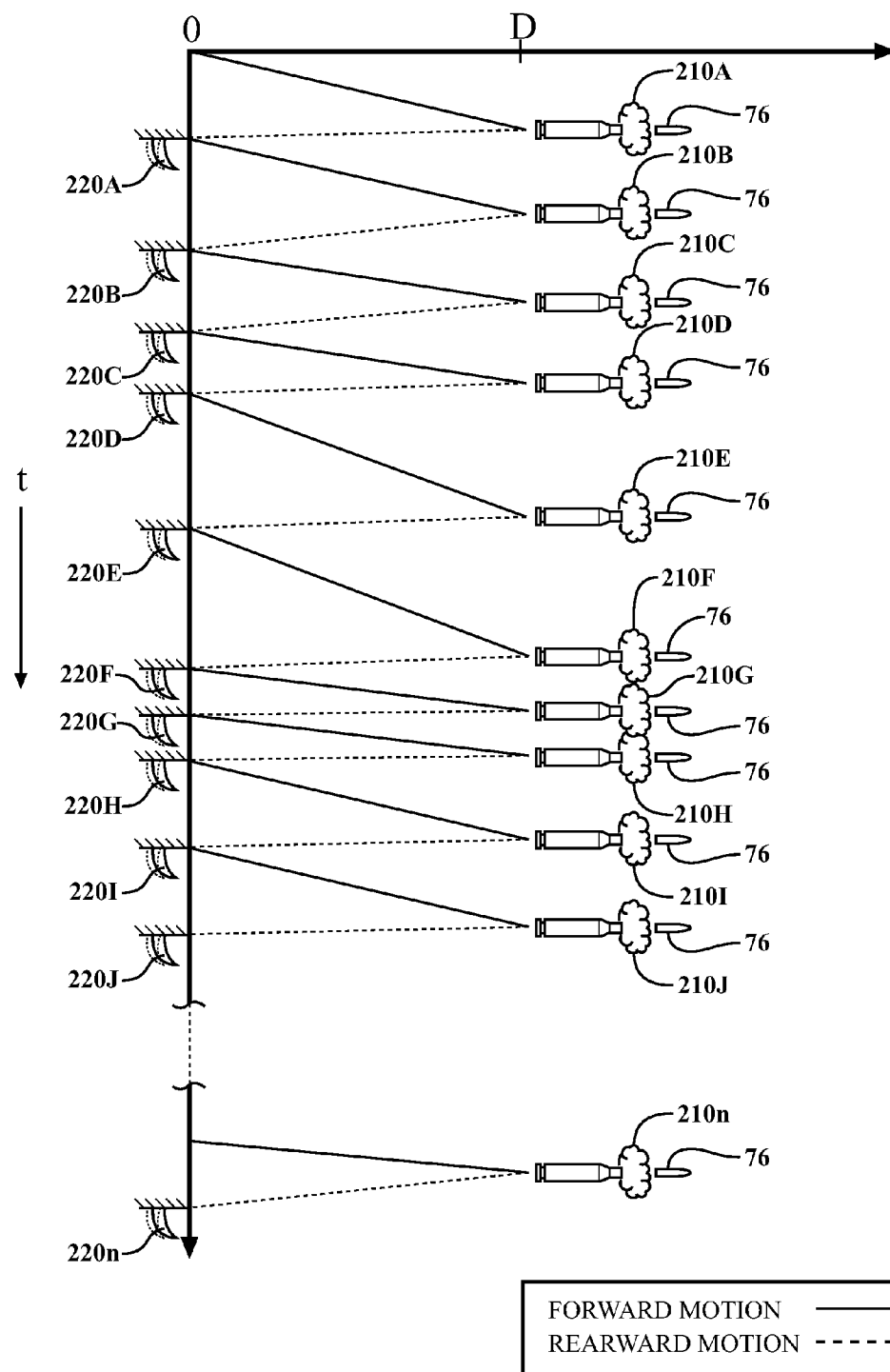
FIG. 12 FIRING UNIT DISPLACEMENT
