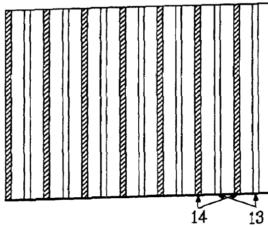
FIG. 2C Prior Art
