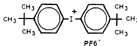
Thermal acid generator
