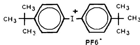
Thermal acid generator
