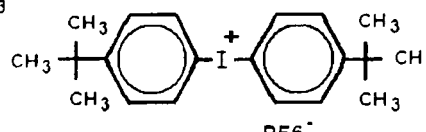
Thermal acid generator
