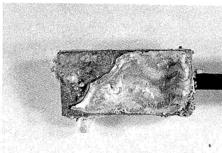
FIG. 2 CATHODE OF UNTREATED SOLID MO
