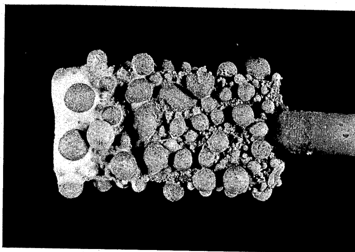
FIG. 1 CATHODE OF UNTREATED STEEL (ST37)
