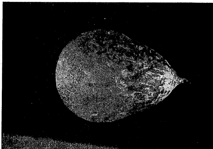
FIG. 6 CATHODE OF SOLID 70% MO, 30% W
