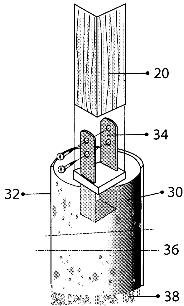
Fibre Tube Poured Concrete Footing
