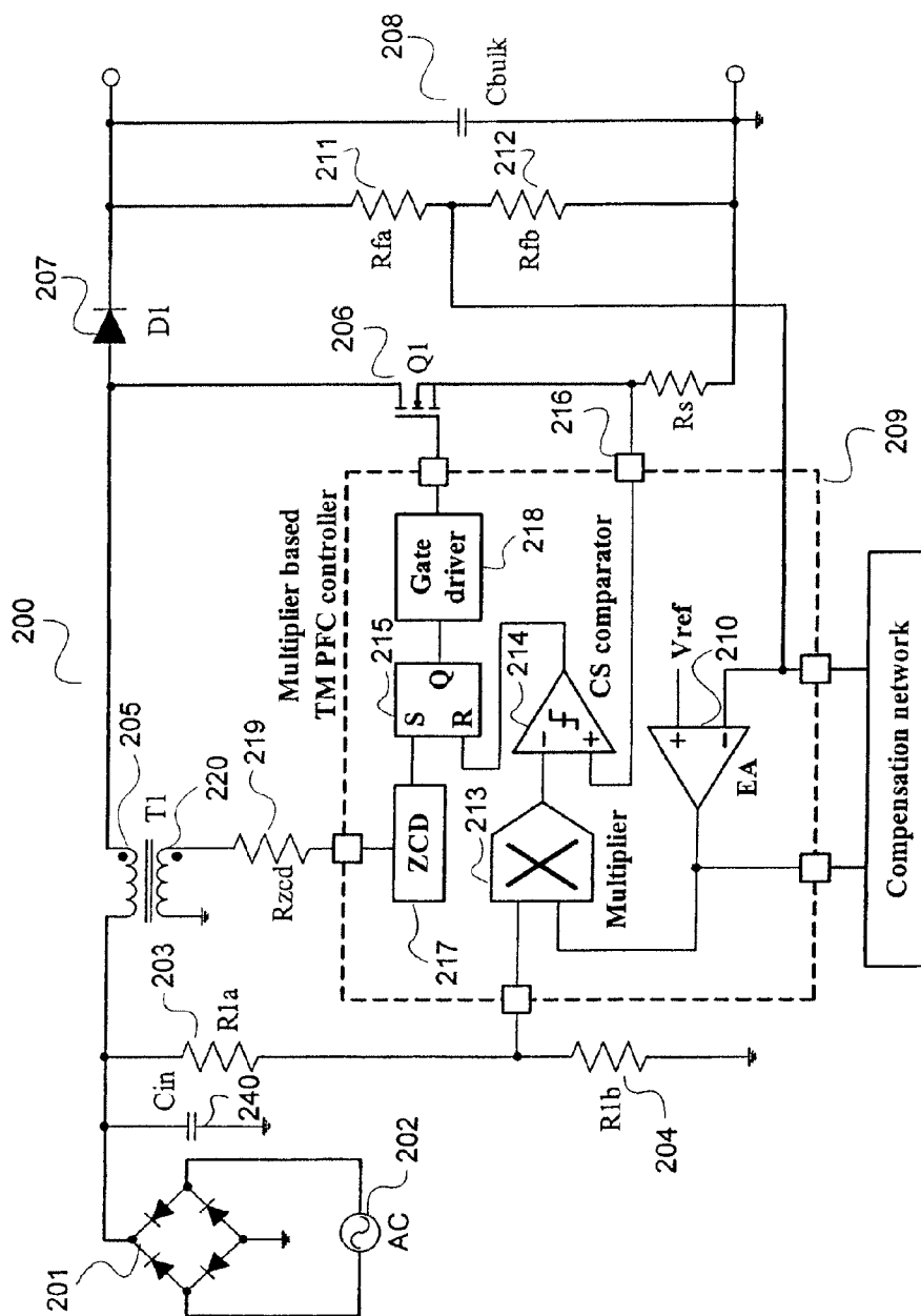
FIG. 2 (Boost Converter)
