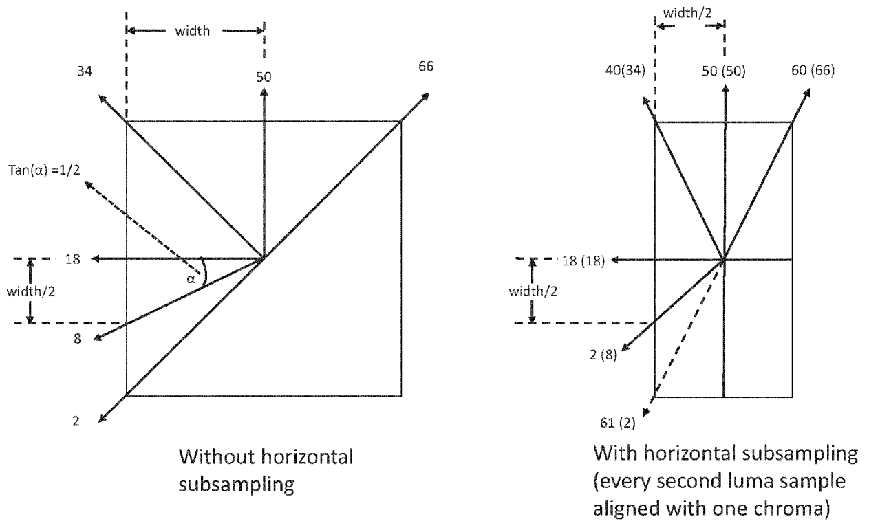
FIG. 10: an example of corresponding modes of original mode and the case when chroma subsampling is applied at horizontal direction using 4:2:2 chroma subsampling format
