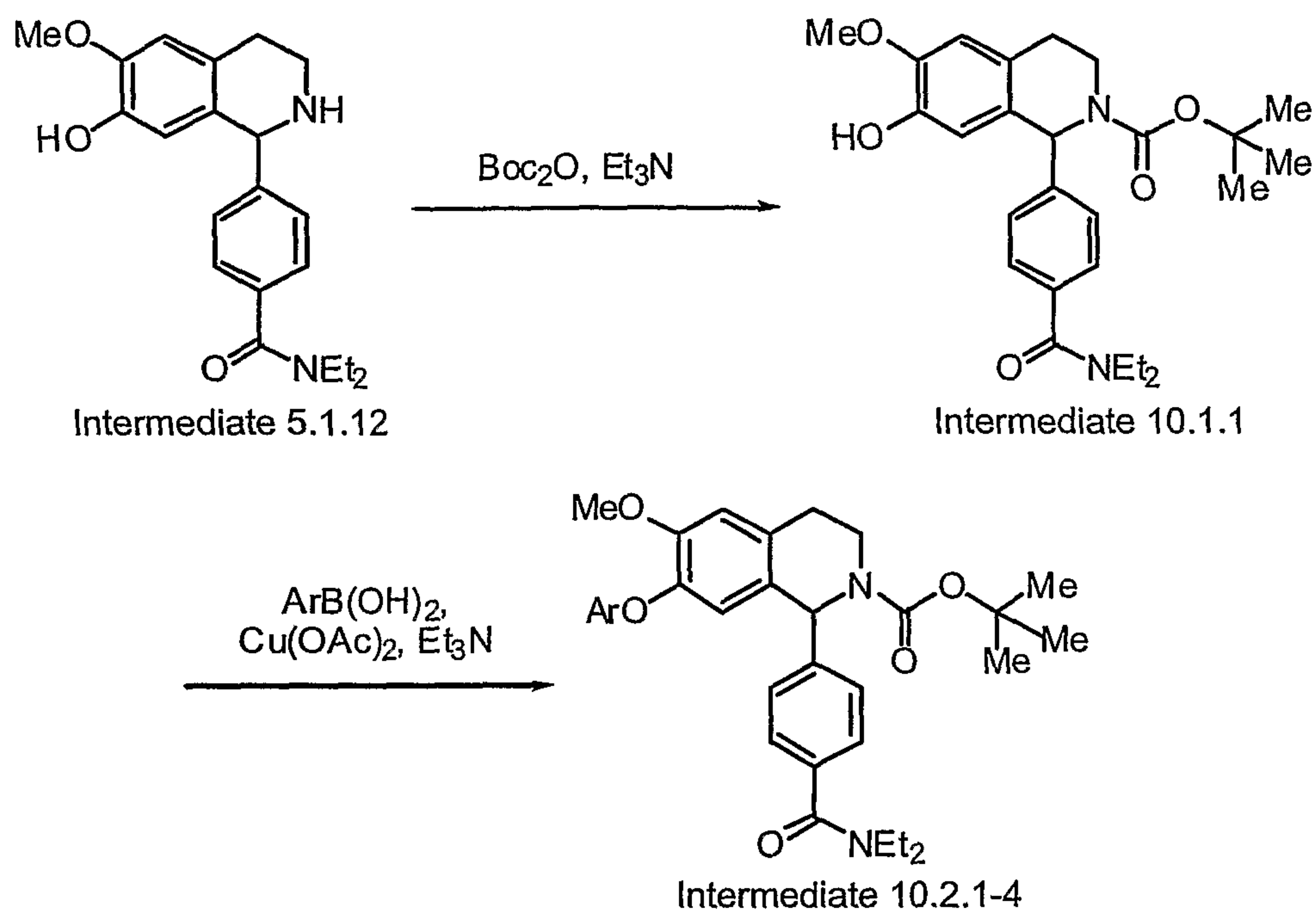
Scheme 10
