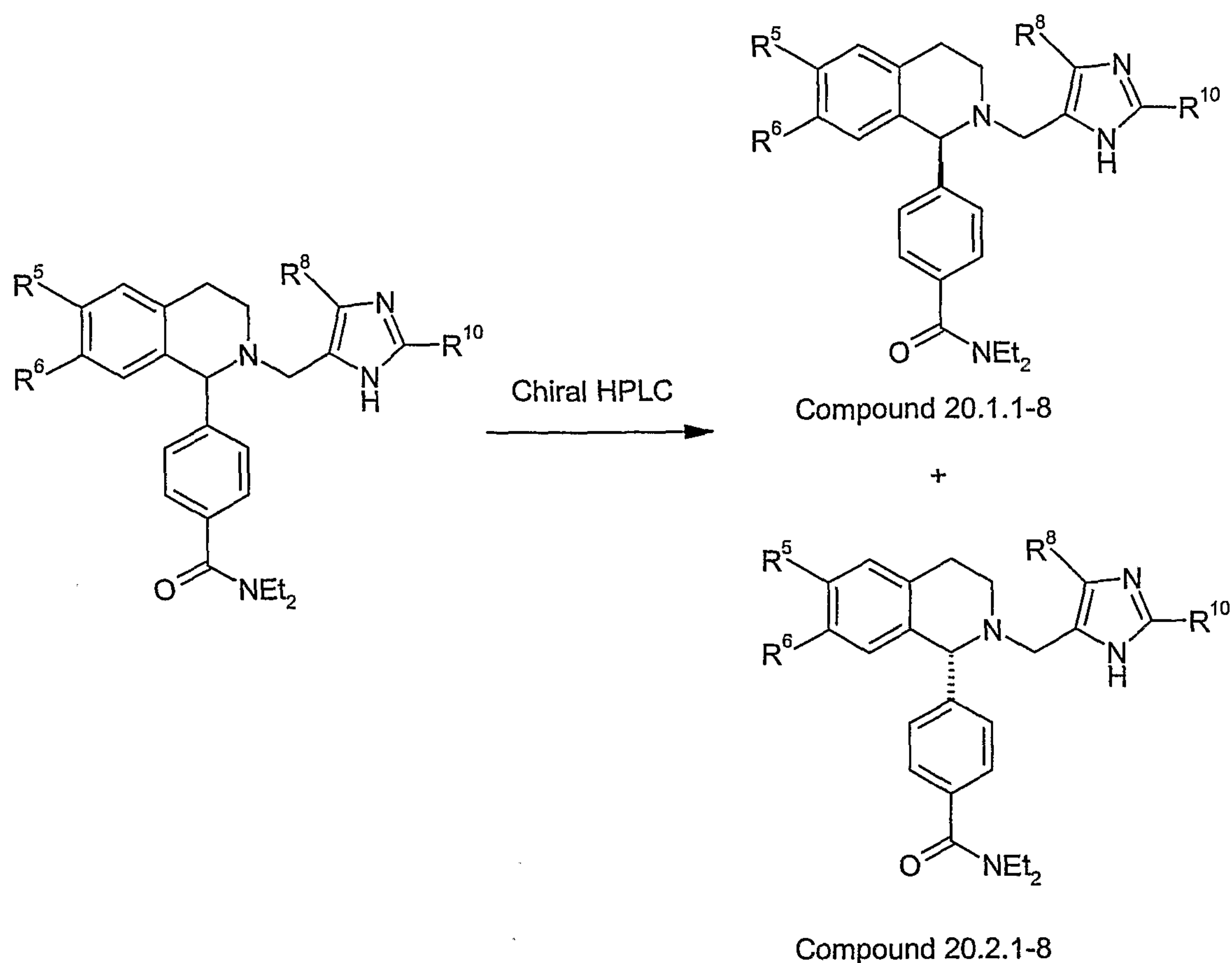
Scheme 20
