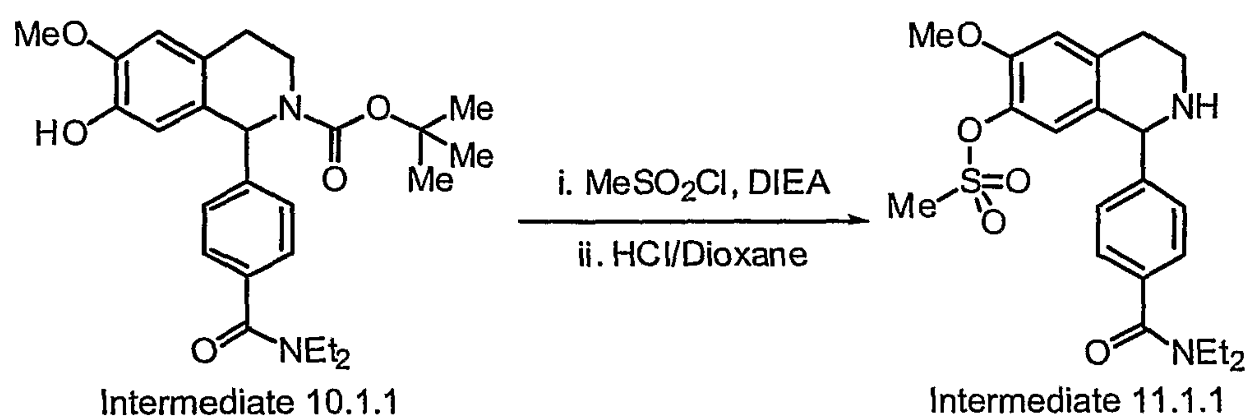
Scheme 11
