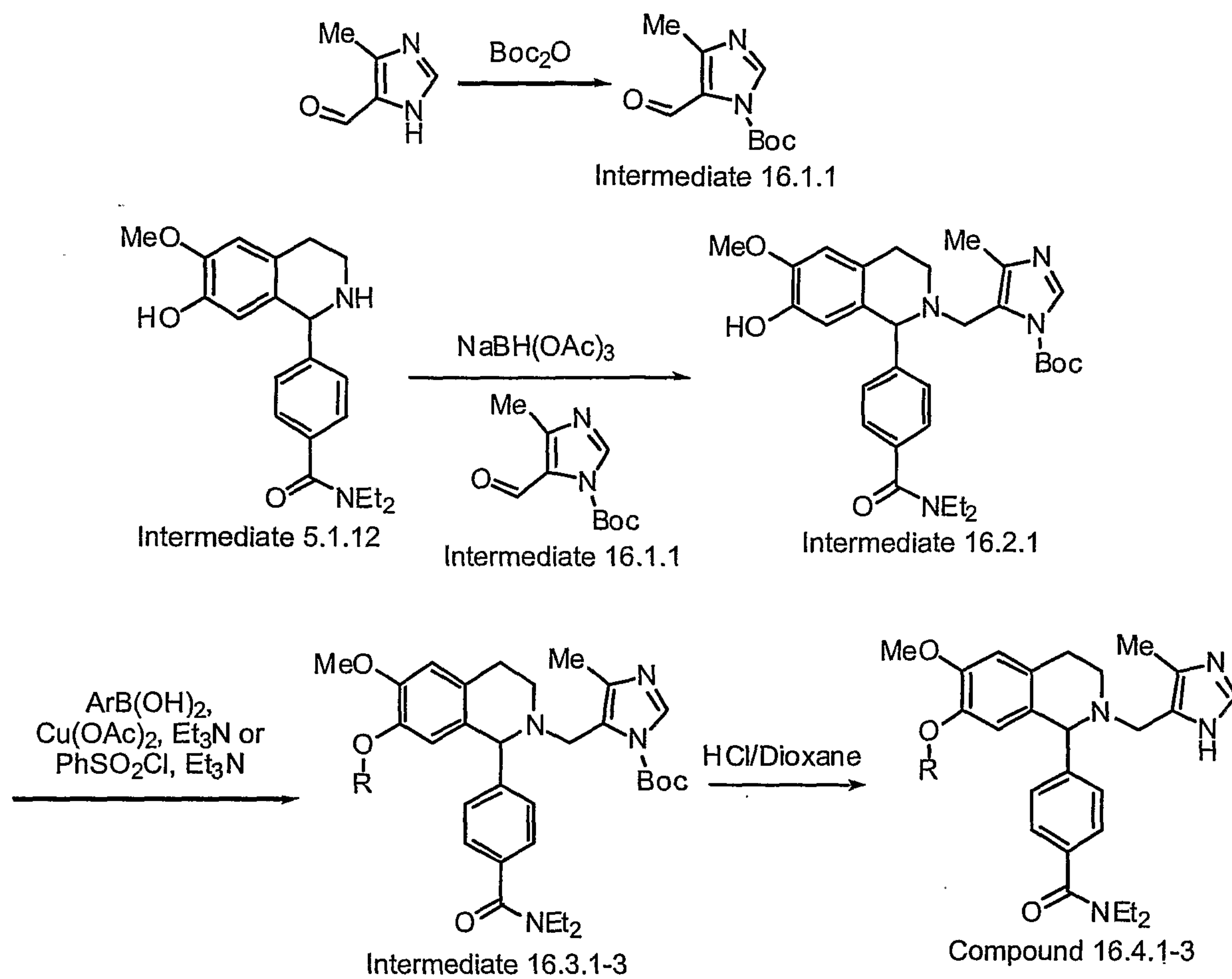
Scheme 16
