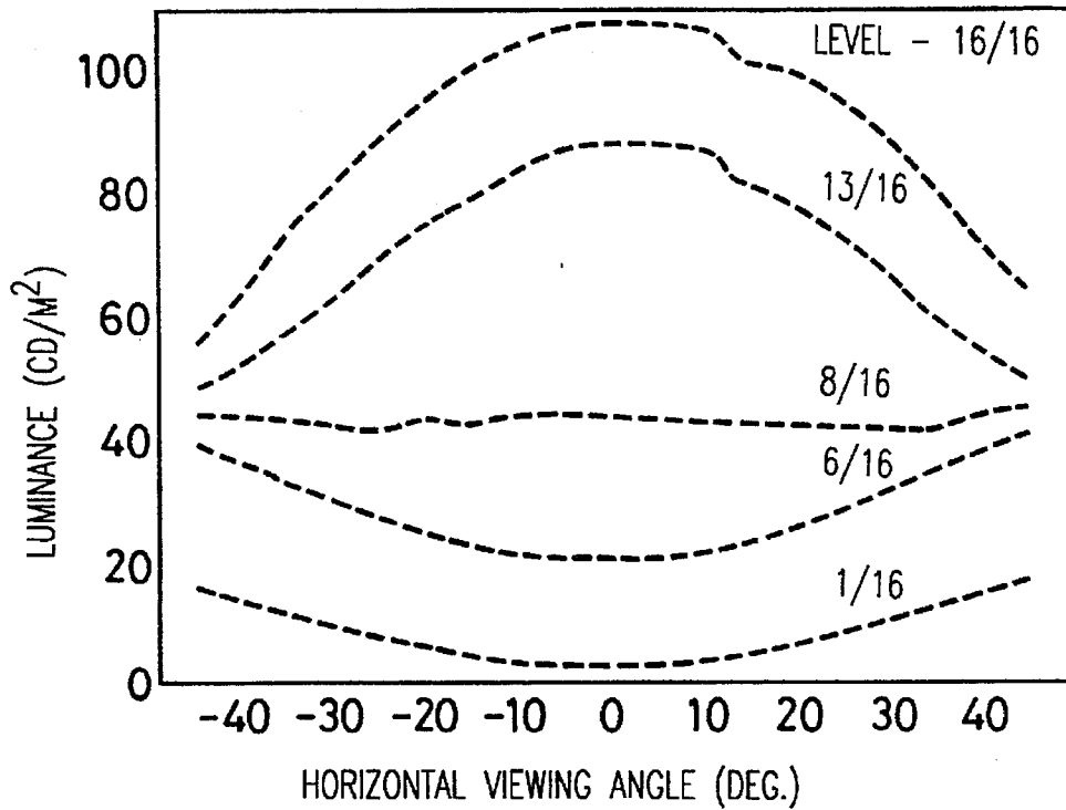
FIG. 12 PRIOR ART
