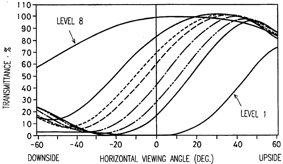
FIG. 8 PRIOR ART
