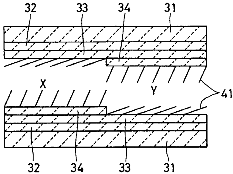
FIG. 9 PRIOR ART
