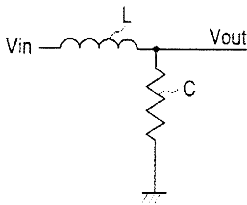
RL INTEGRATION CIRCUIT
