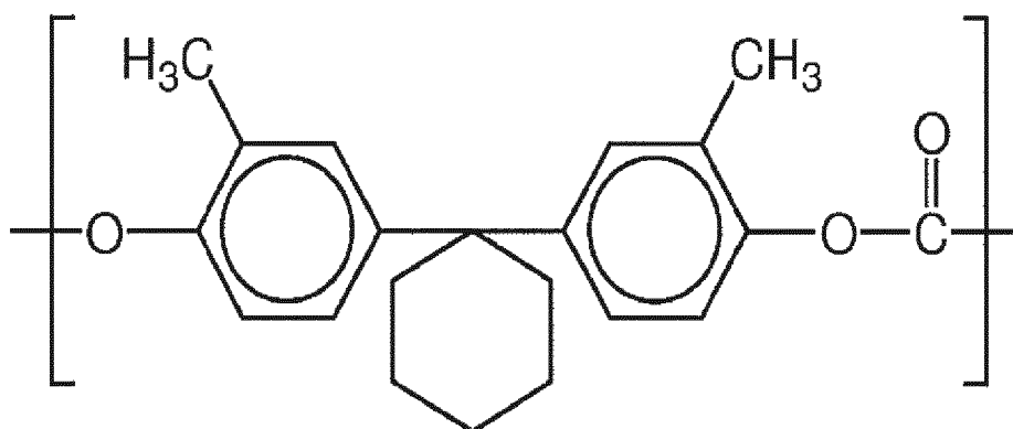
Formula (VI).
