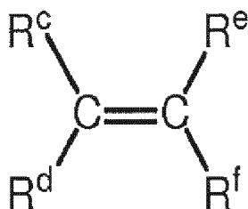
Formula (VI)
