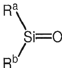
Formula (V)
