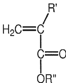
Formula (III)
