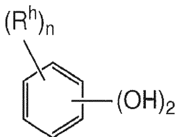
Formula (II)
