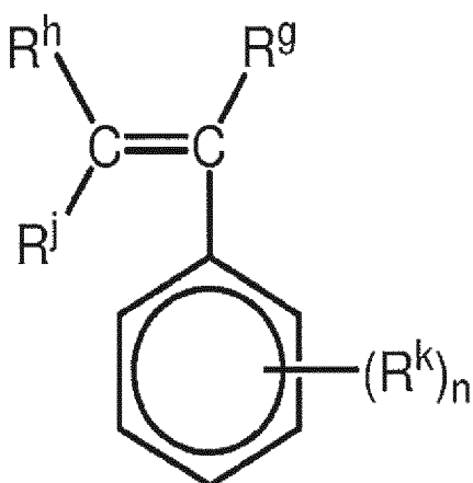
Formula (IV)
