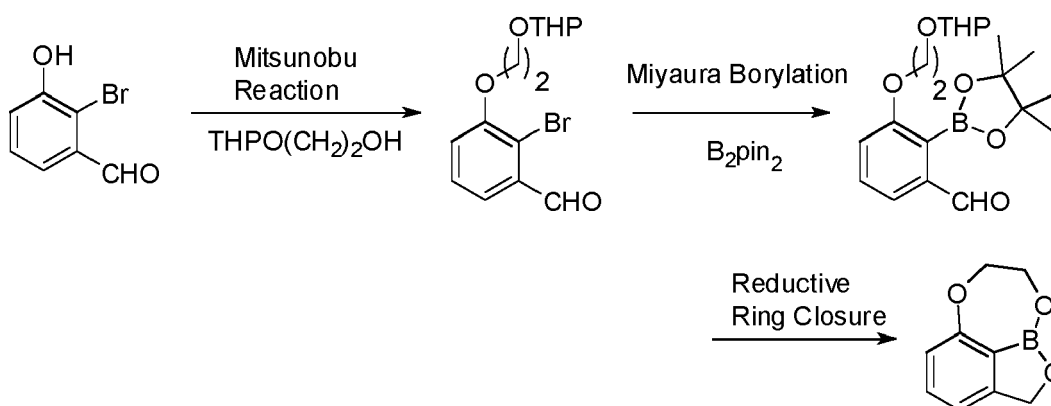
Scheme I
