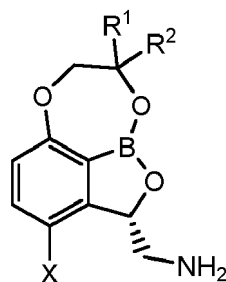
Formula IIa
