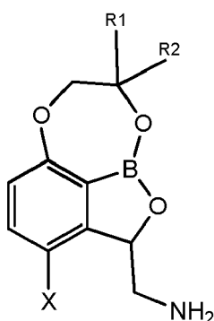
Formula II ,
