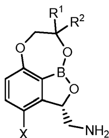
Formula IIa
