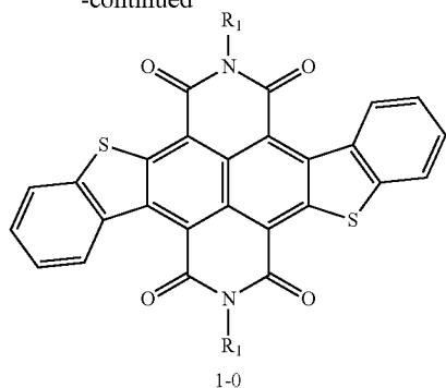
[Scheme 2]
