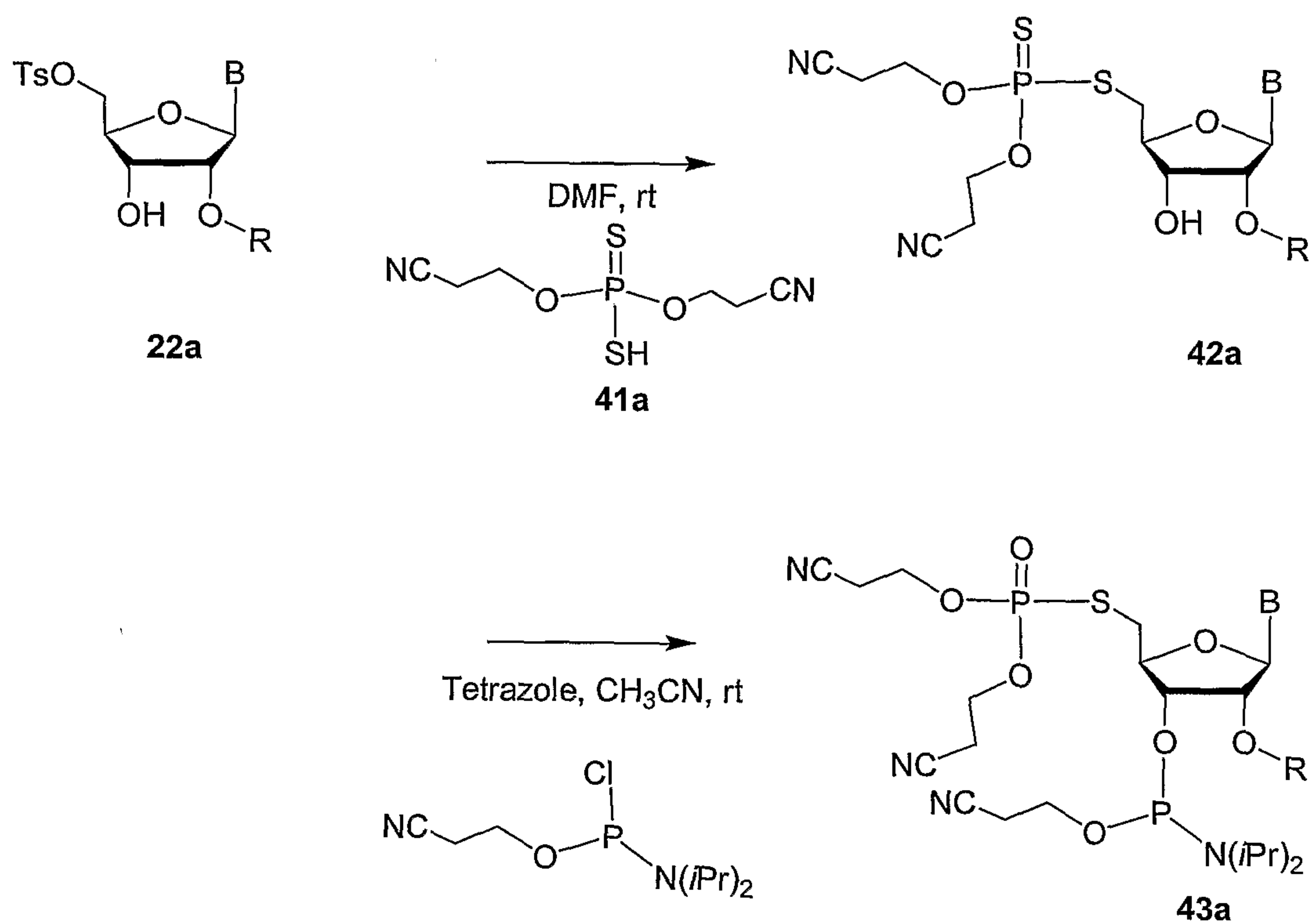
Scheme 2
