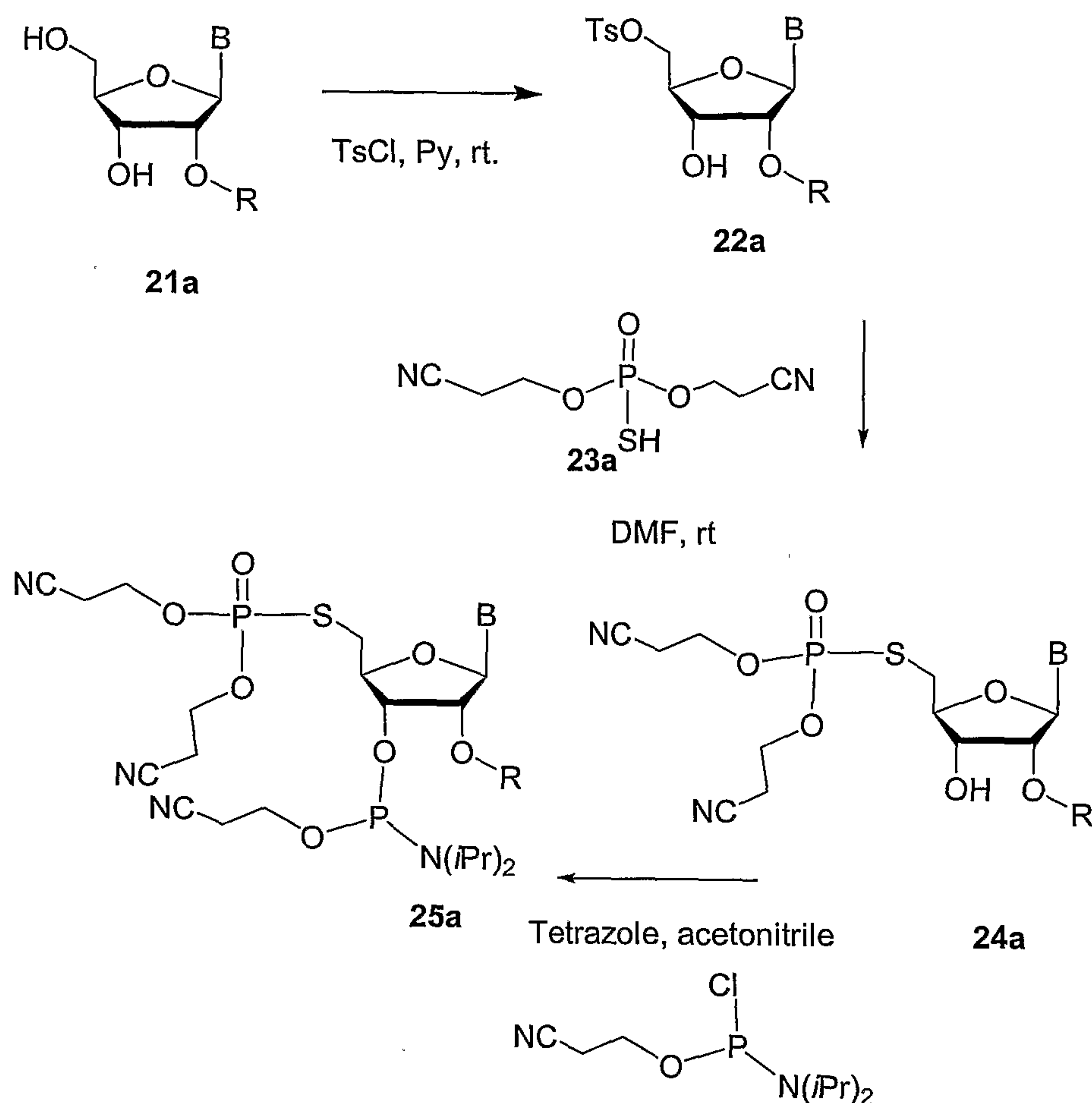
Scheme 1
