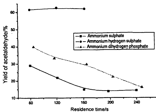
Figure 1: Yields of acetaldehyde in the continuous reaction of acrolein with ammonium salts in near-critical water at 360°C and 30 MPa and with different residence times.
