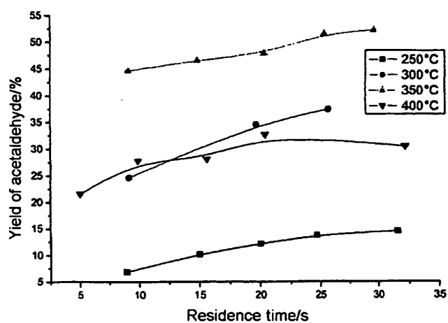
Figure 2: Yields of acetaldehyde in the continuous reaction of 0.25% (g g -1 ) of acrolein with 0.59% (g g -1 ) of ammonium sulphate in near-critical water at 30 MPa and with different temperatures and residence times.
