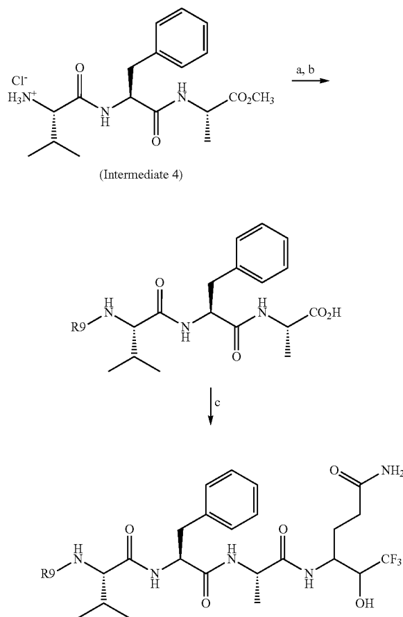
Scheme 2 a
