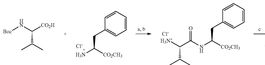
Scheme 3 a
