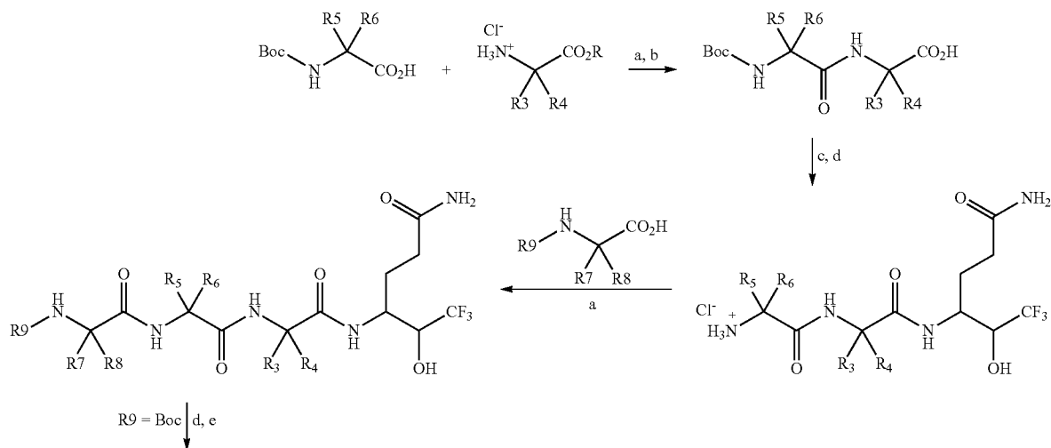
Scheme 7 a
