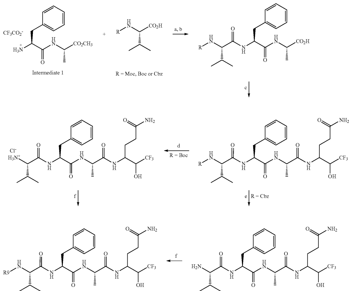
Scheme 1 a
