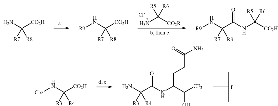
Scheme 5 a
