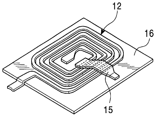
FIG. 11 PRIOR ART
