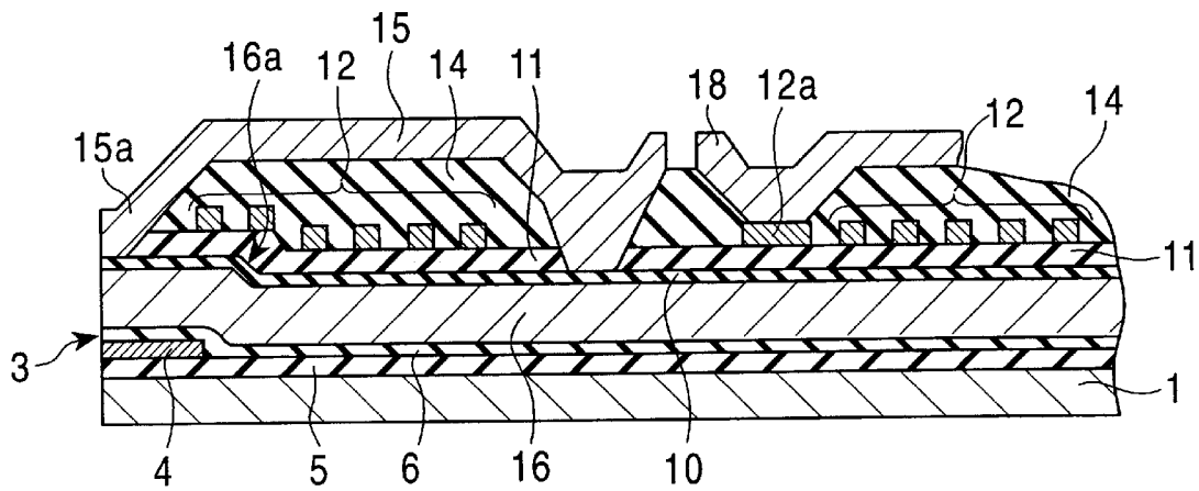
FIG. 12 PRIOR ART
