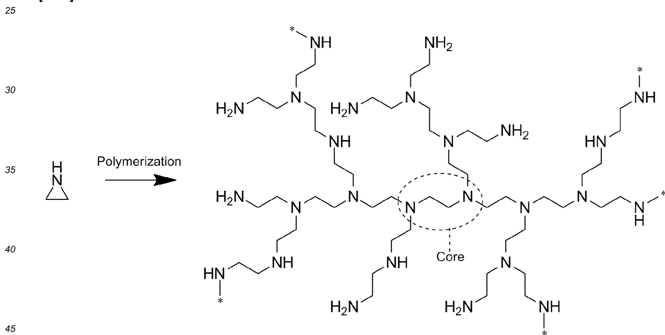
Scheme 2. Synthesis of a PEI hyperbranched polymer. In Scheme 2: the PEI hyperbranched polymer is of the 4 th generation having a ethane-1,2-diamine core (Mw = 56 Da). * indicates exemplary positions where further aziridine monomers may be added.
