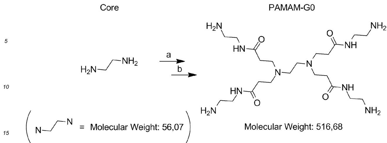
Scheme 1. Synthesis of a PAMAM-G0 dendrimer. In Scheme 1: a is methyl acrylate and b is ethane-1,2-diamine.
