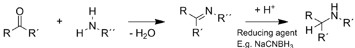
Scheme 4. Reductive amination
