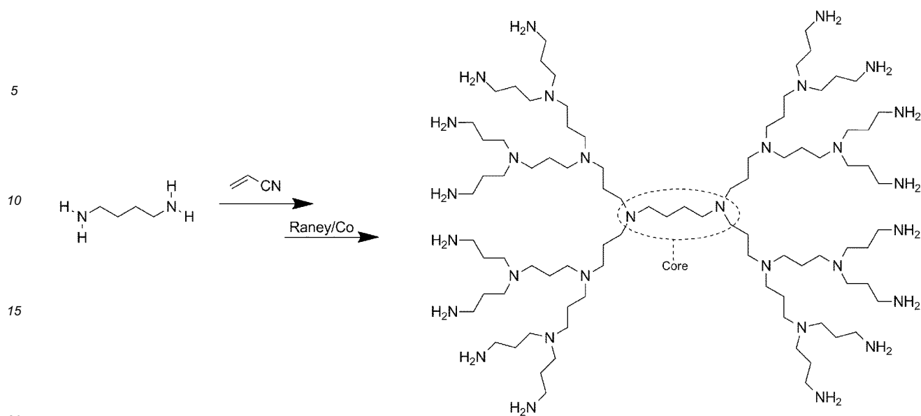
Scheme 3. Synthesis of PPI dendrimer. In Scheme 3: the PPI dendrimer is of the 3 rd generation having a butane-1,4-diamine core (Mw = 84 Da).
