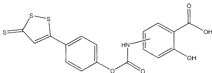
2-Hydroxy-4 or 5[4-(5-thio-5H-[1,2]dithiol-3-yl)-phenoxy-carbonylamino]-benzoic acid (V),
