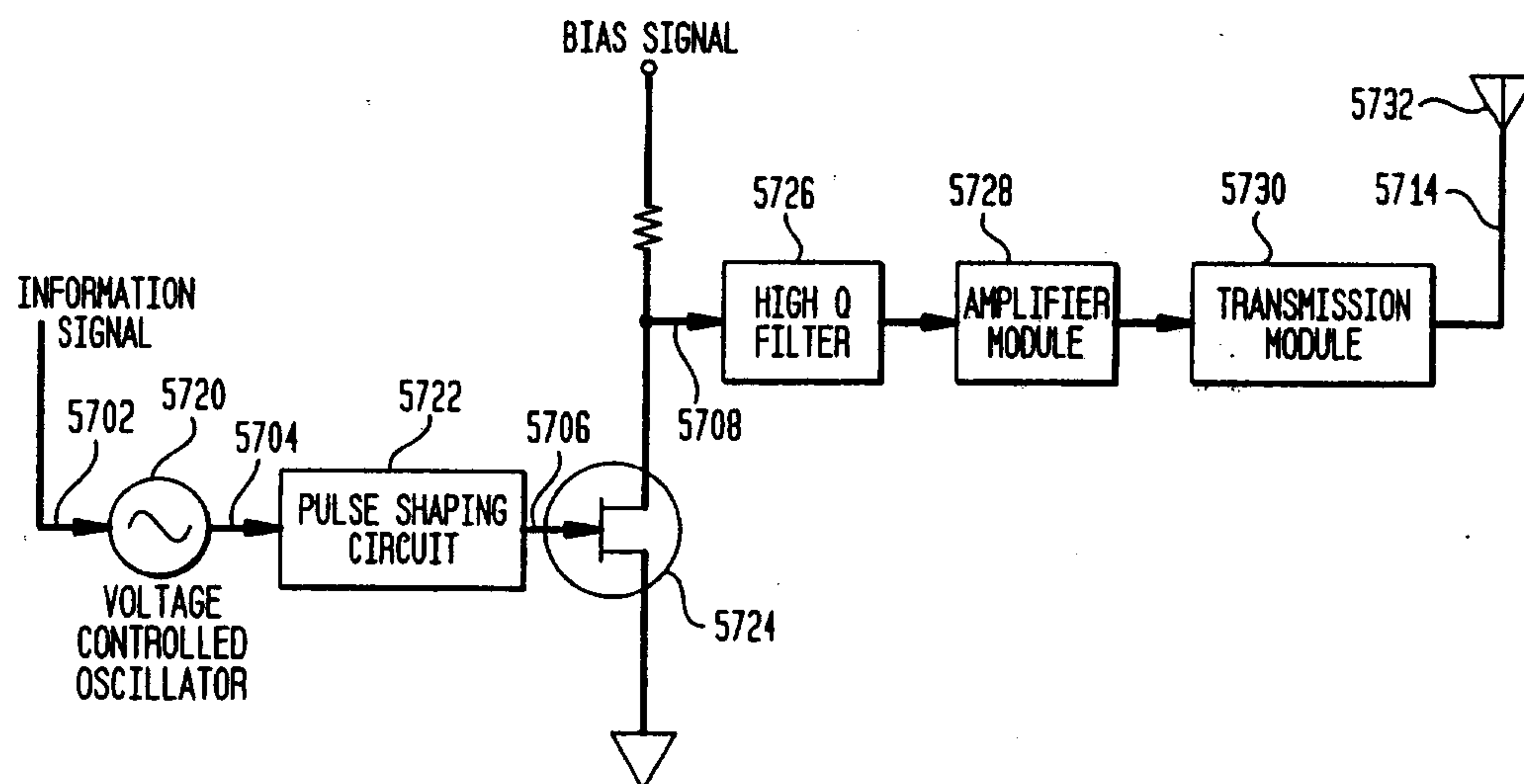
FIG. 57A TRANSMITTER IN THE FM EMBODIMENT
