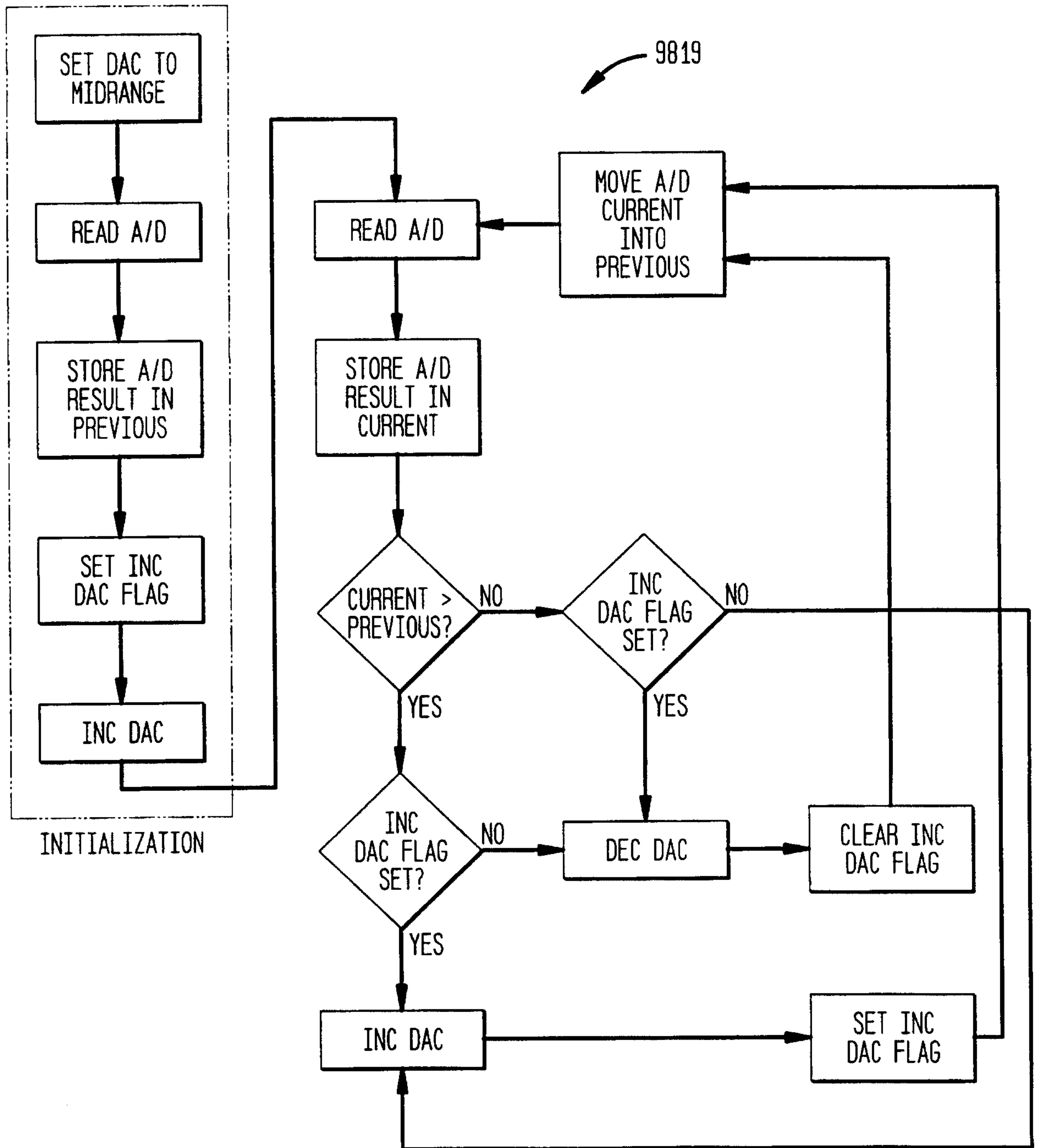
STATE MACHINE FLOWCHART
